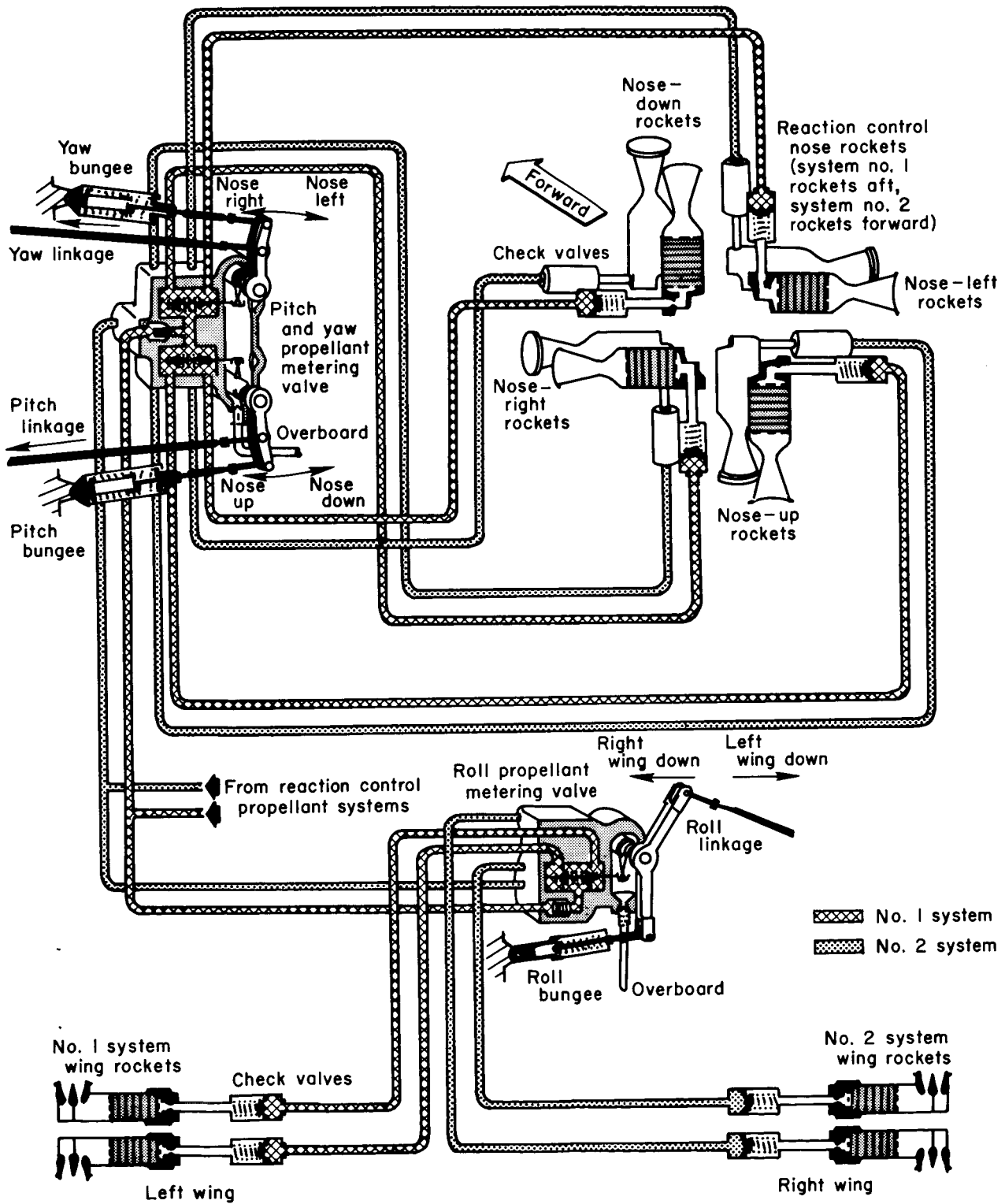
Figure 3.— Schematic diagram of X-15 manual reaction control system components.
