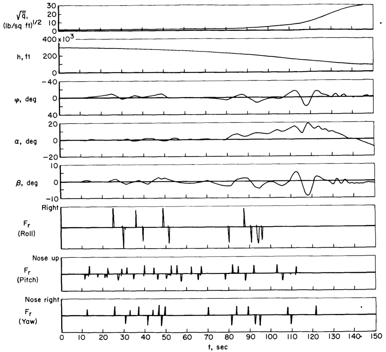
Figure 17.- X-15 manual acceleration command reentry made with six-degree-of-freedom flight simulator. Ventral-on configuration.
