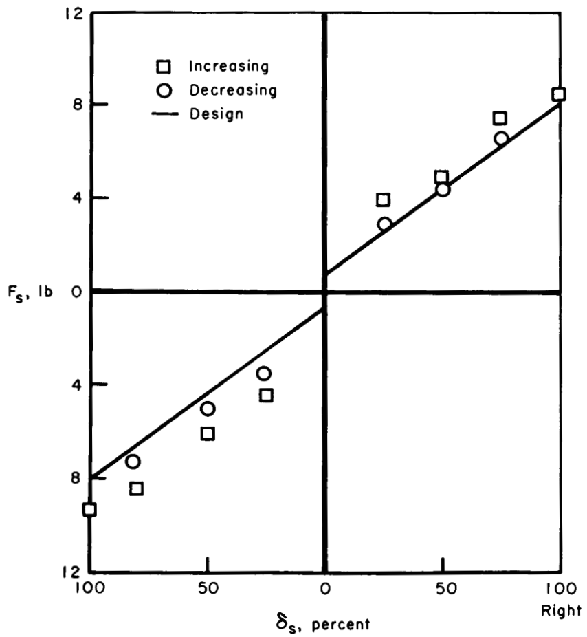
(b) Roll axis; maximum \delta_s = \pm 18^\circ .
