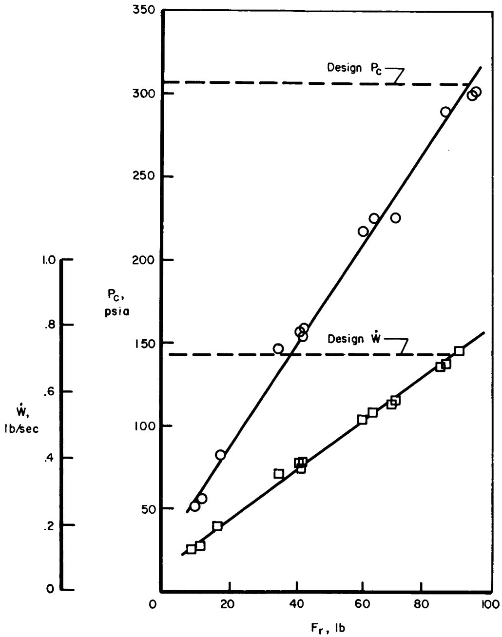
(a) Type A control rocket.
