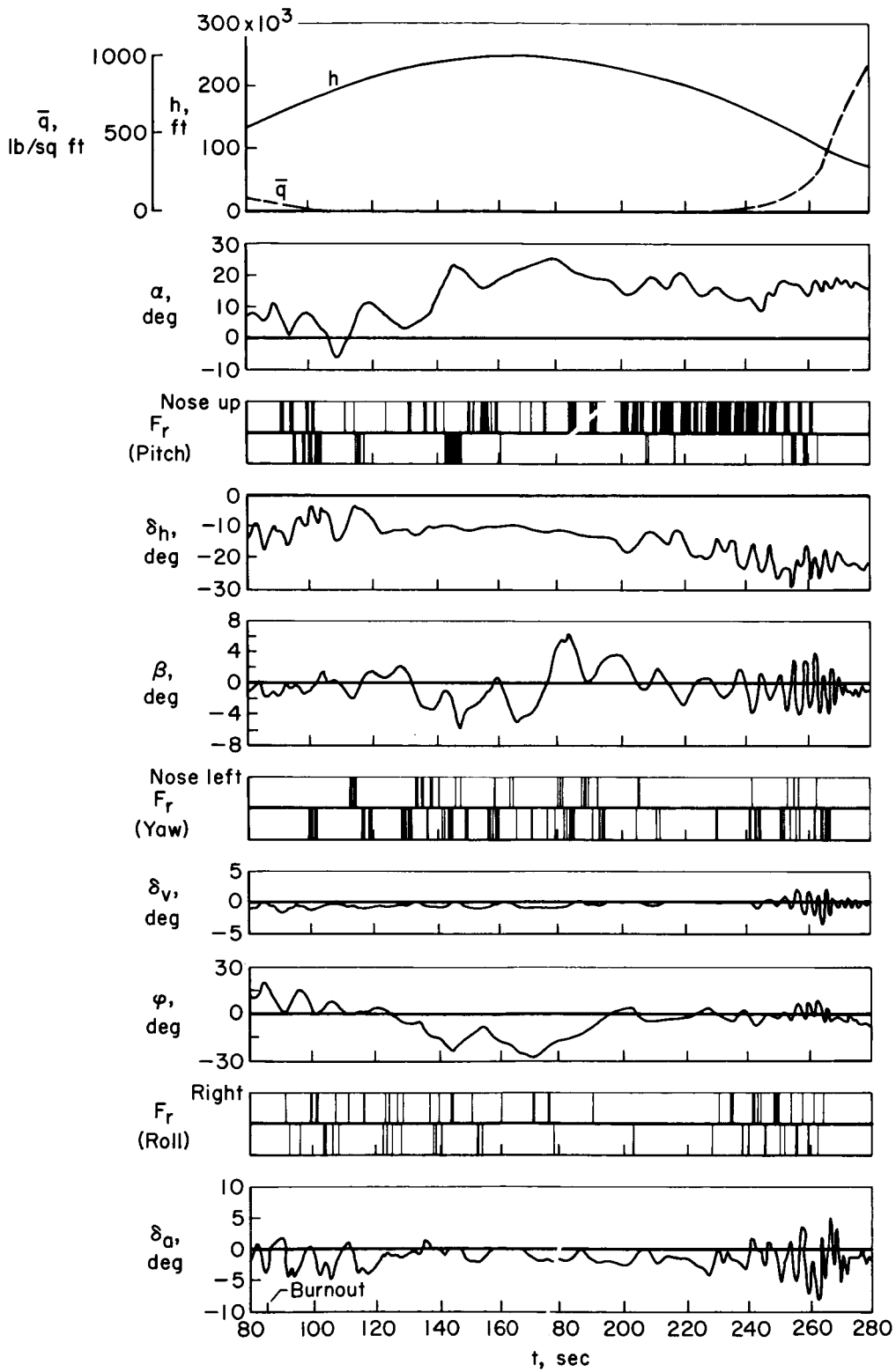
Figure 14.- Time history of reaction control portion of an X-15 high-altitude flight during which manual acceleration command system was used (time t referenced to launch).
