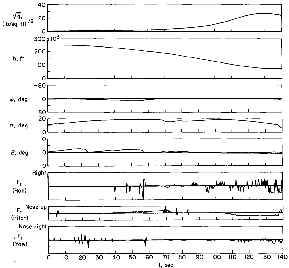
Figure 18.- X-15 reentry performed on a six-degree-of-freedom flight simulator using reaction control damping. Ventral-on configuration.
