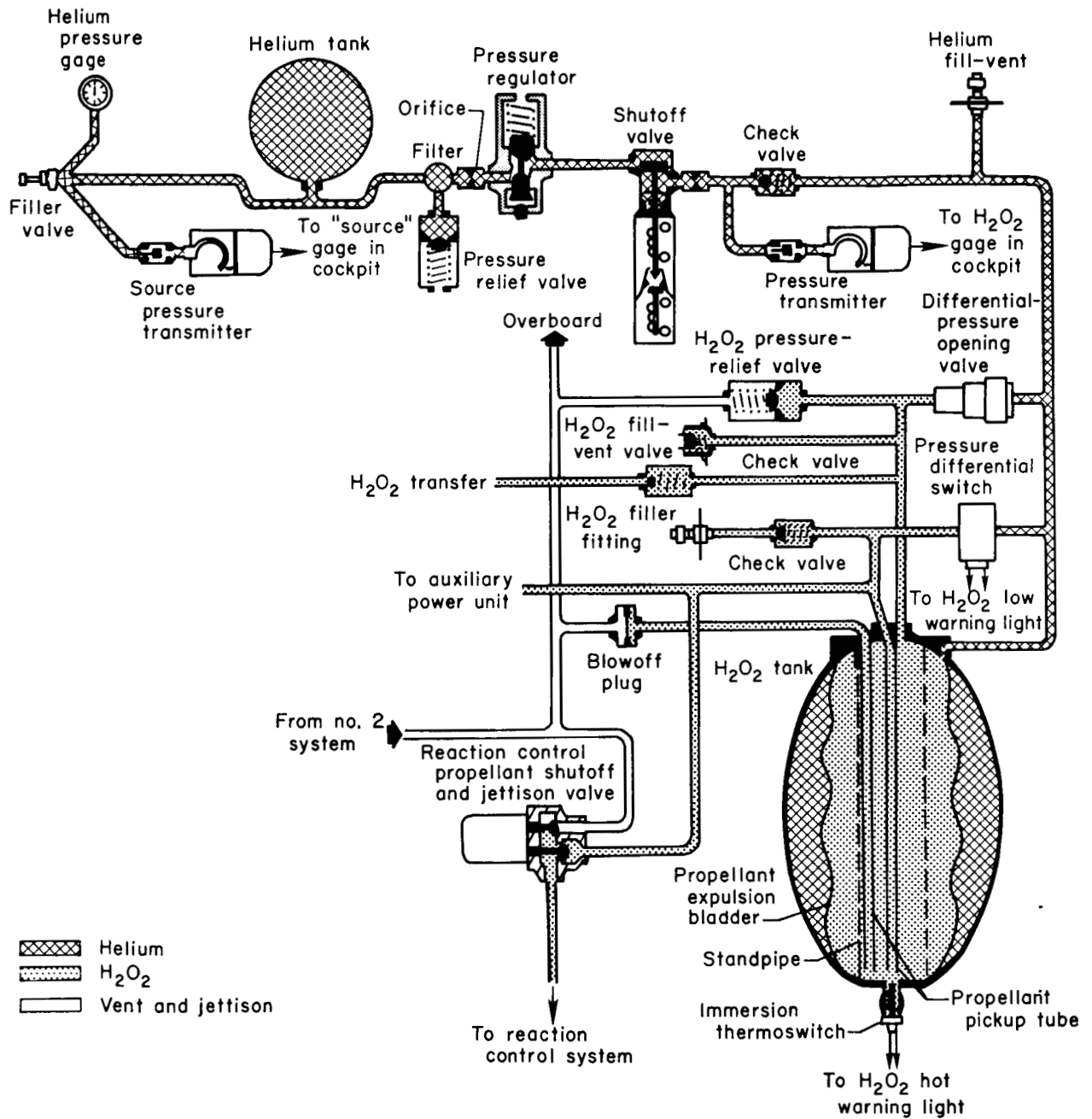
Figure 8.- X-15 reaction control propellant supply system (no. 1).
