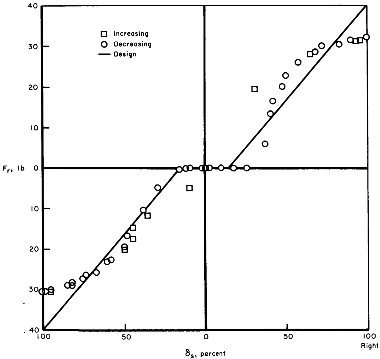
(b) Roll axis; maximum \delta_s = \pm 18^\circ .
