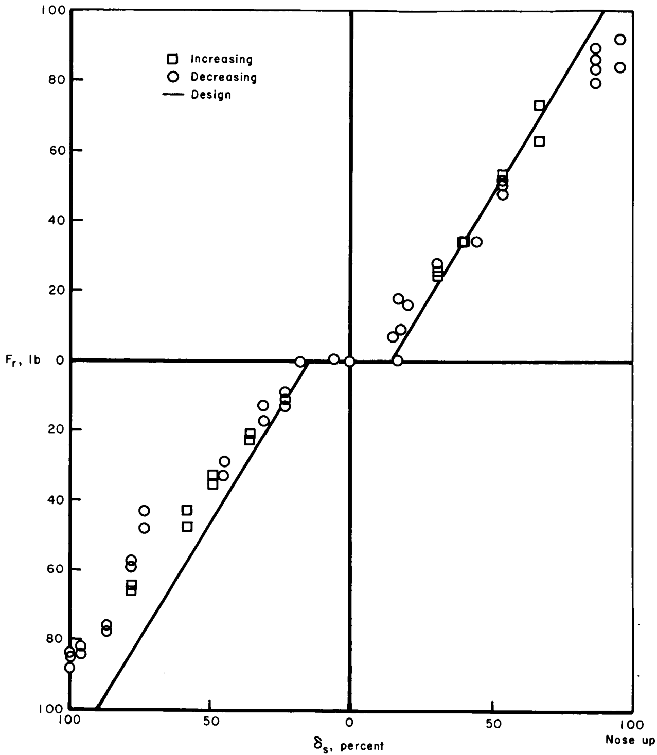
(a) Pitch axis; maximum \delta_s = \pm 9^\circ 47' .
