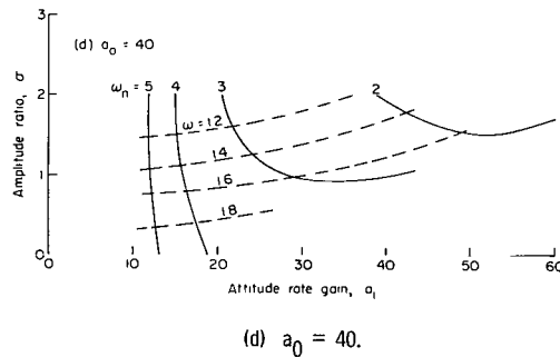
Figure 13.- Nonlinear stability boundaries for \xi = 0.7 .
