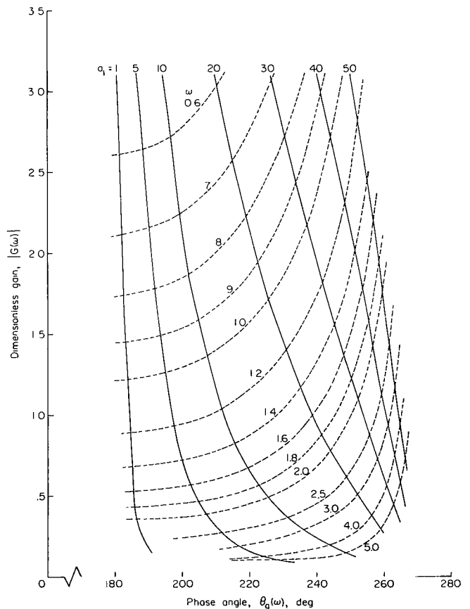
Figure 9.- Typical gain-phase plot of G(\omega) for a_0 = 20 .
