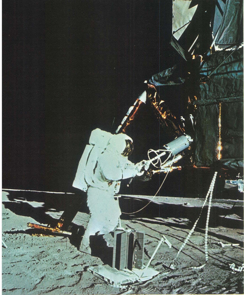
Bean lifts the hot plutonium core, sheathed in its cask, from its place of storage aboard the Intrepid . The generator is in the foreground.
