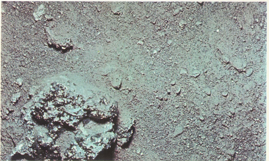
Another lunar rock with an iridescent coating.
