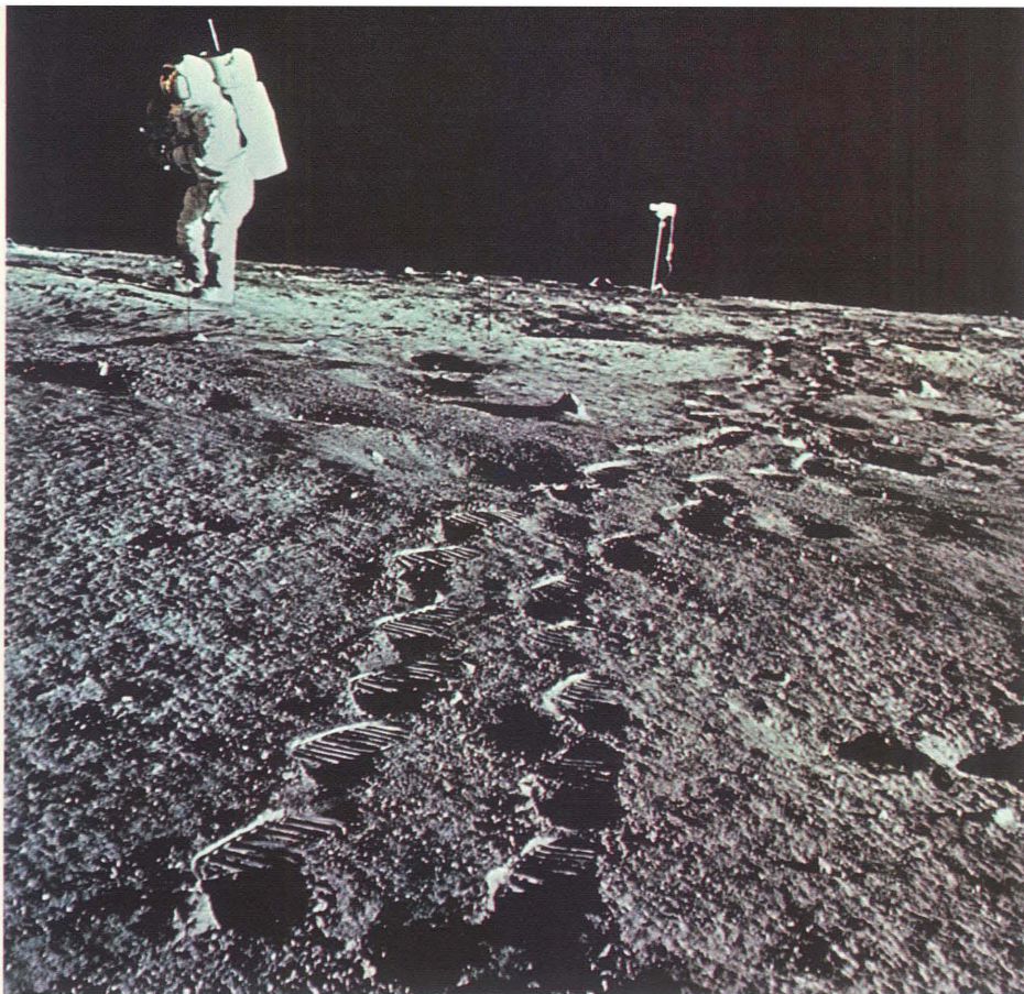
A trail of footprints on the lunar surface. Object in the background is the color television camera that was thought to be sunstruck early in the first of 12's two Moon walks.
