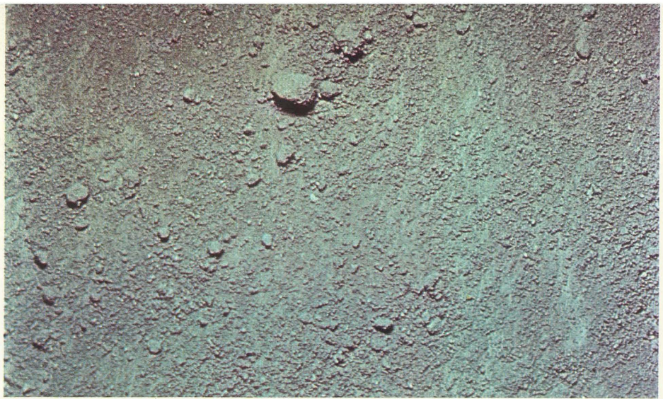
A small rock directly under the Intrepid . The exhaust swept the adjacent surfaces clear of dust but did not move the rock.
