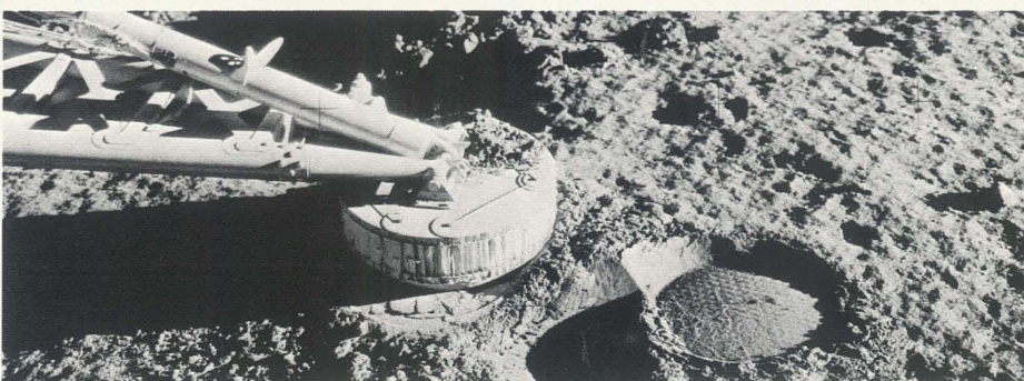
Surveyor footpad next to imprints left by its initial touchdowns. Imprints appear fresh despite 31 months of exposure to the lunar environment.
