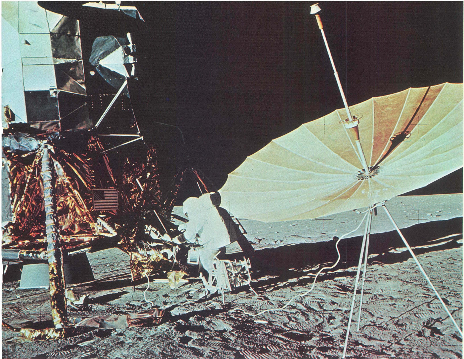
An astronaut prepares an ALSEP experiment for movement to the site where it will be set up. At right, the S-band dish antenna.
