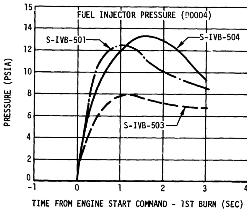
Figure 9-10. Fuel Lead - First Burn
