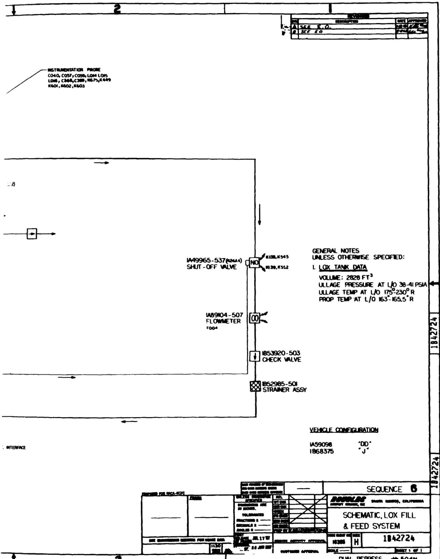
Figure 11-21. Schematic, LOX Fill and Feed System
