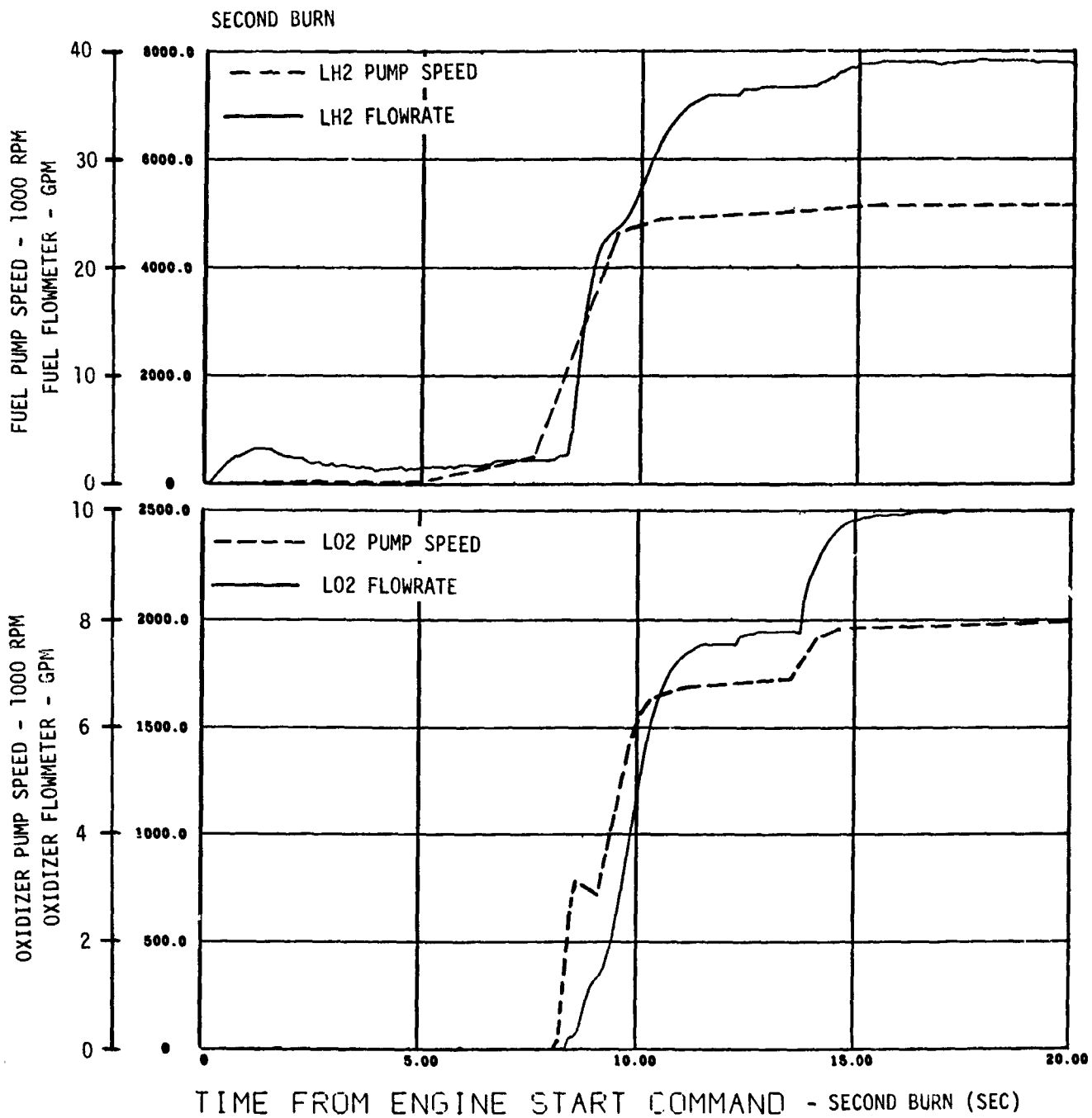
Figure 9-3i. LOX and LH2 Pump Performance (Sheet 2 of 3)
