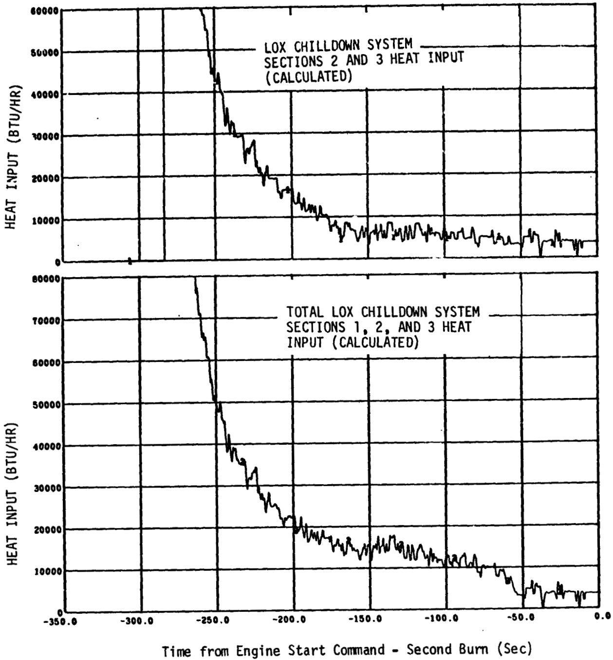
Figure 11-20. LOX Pump Chilldown System Performance - Second Burn (Sheet 2 of 2)
