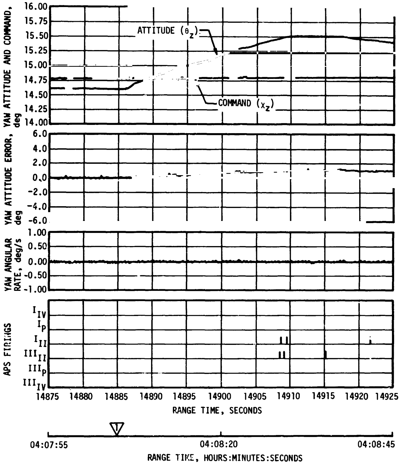
Figure 21-26. Yaw Attitude Control During LM Extraction
