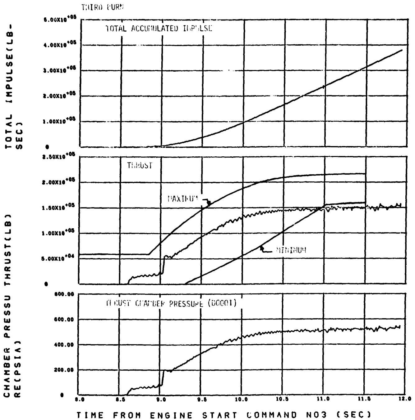
Figure 9-29. Engine Start Transient Characteristics (Sheet 3 of 3)
