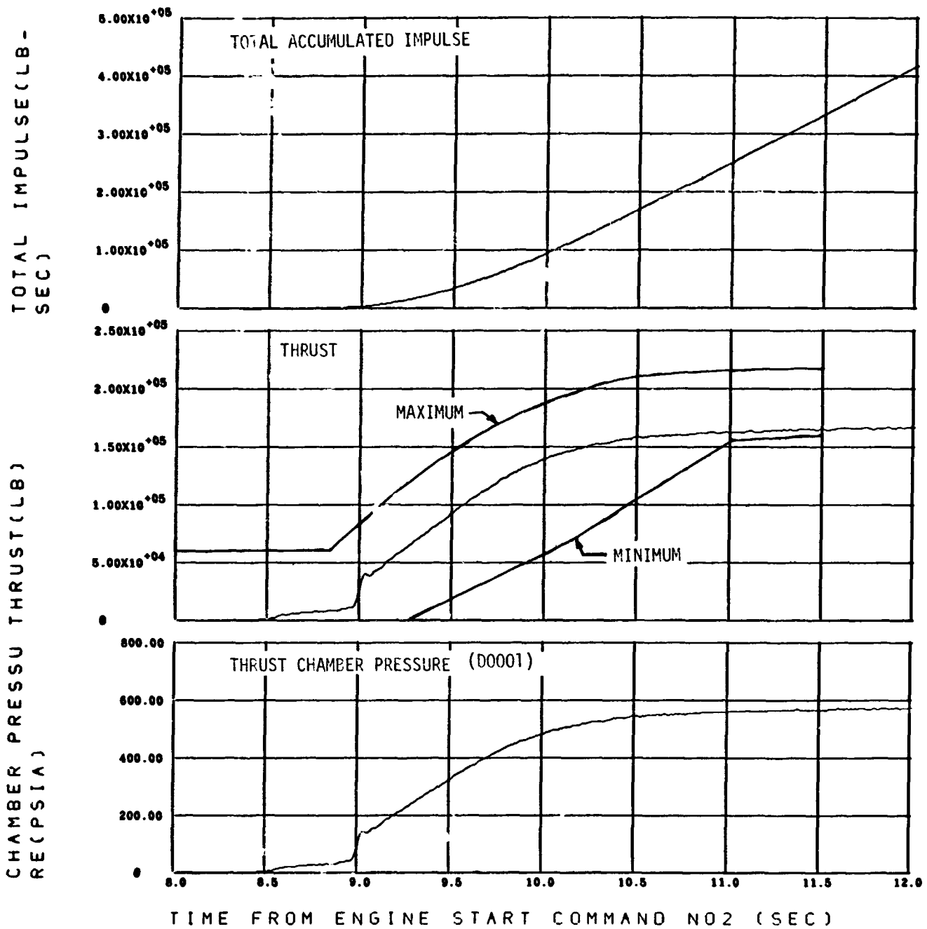
Figure 9-29. Engine Start Transient Characteristics (Sheet 2 of 3)
