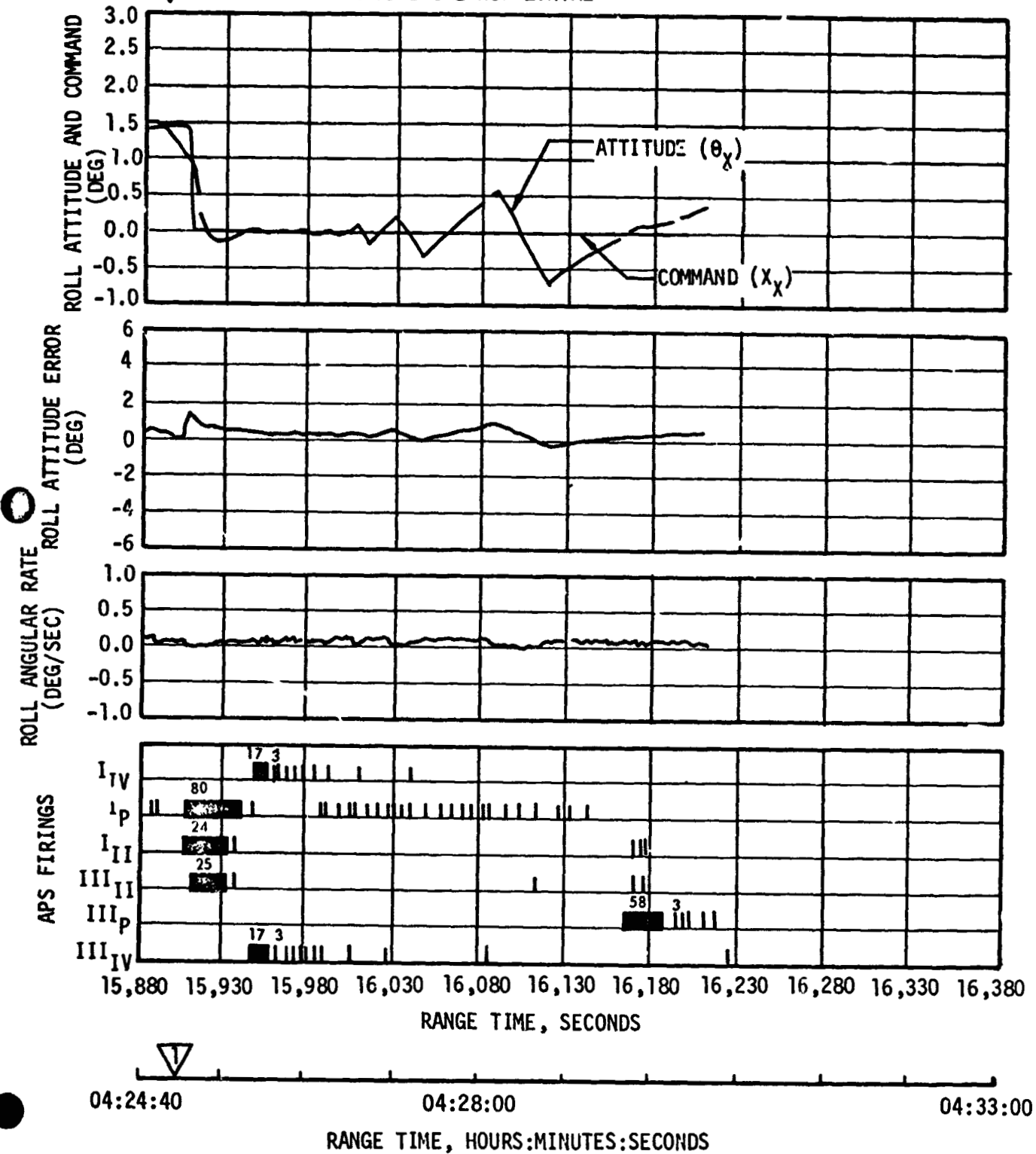
Figure 21-30. Roll Attitude Control during Alignment of S-IVB to Local Horizontal prior to Second Burn
