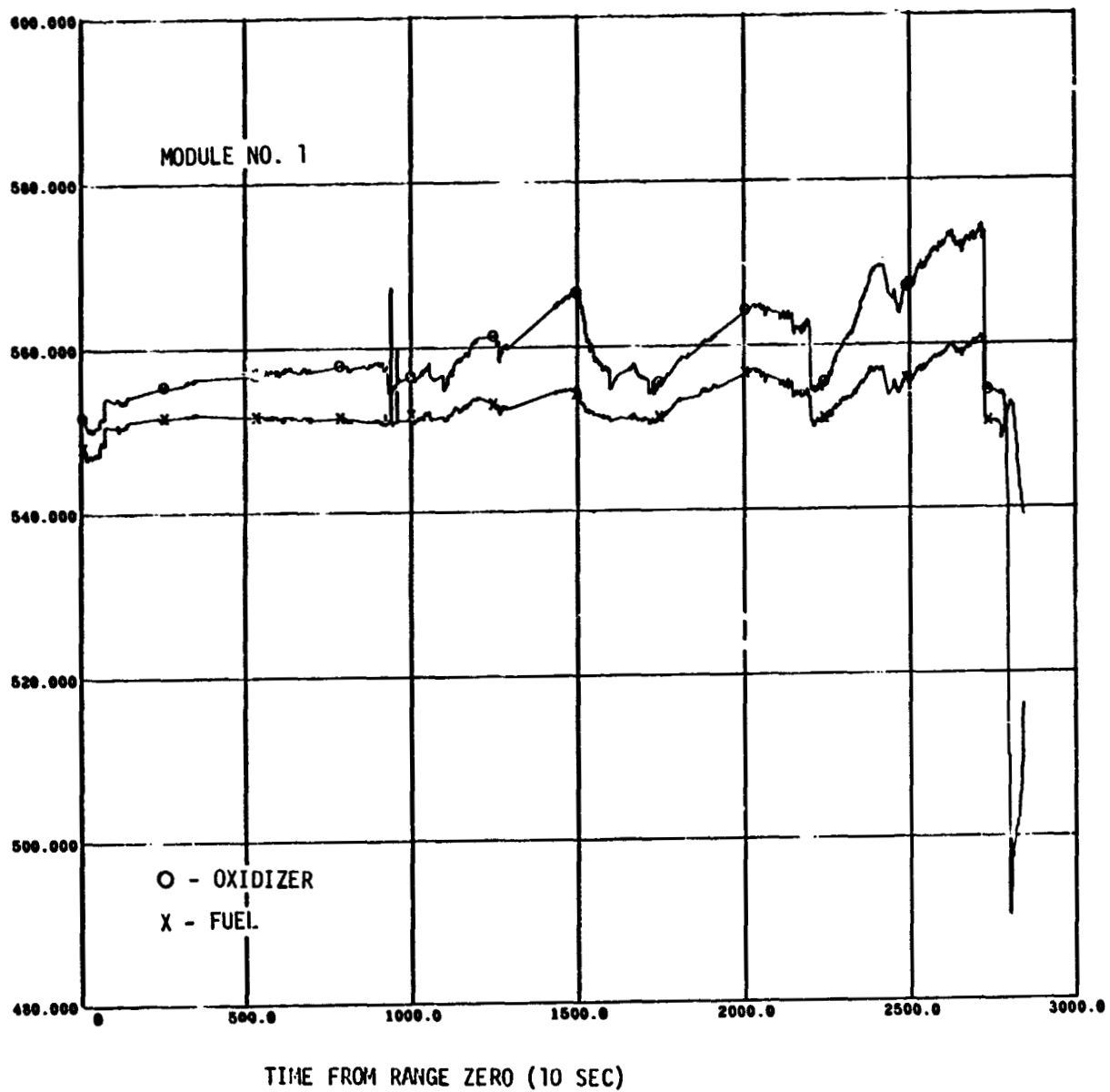
Figure 14-8. APS Module No. 1 Propellant Temperatures
