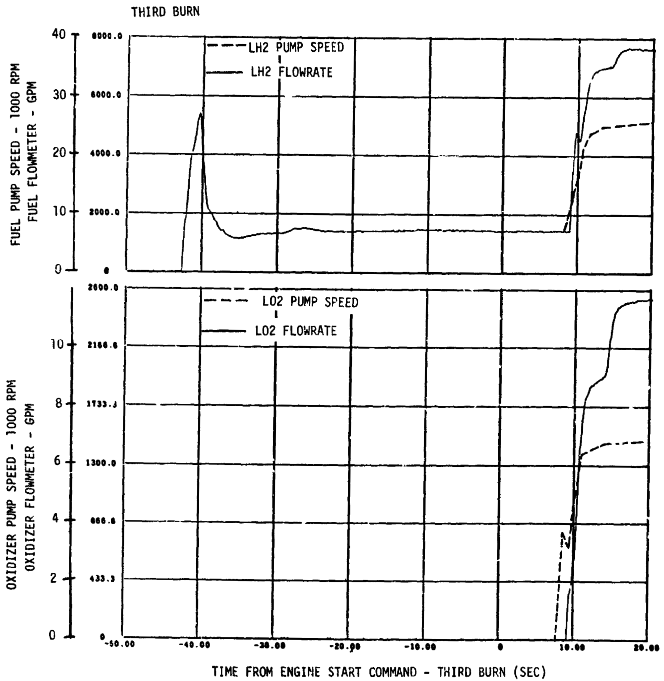
Fig. 9-31. LOX and LH2 Pump Performance (Sheet 3 of 3)
