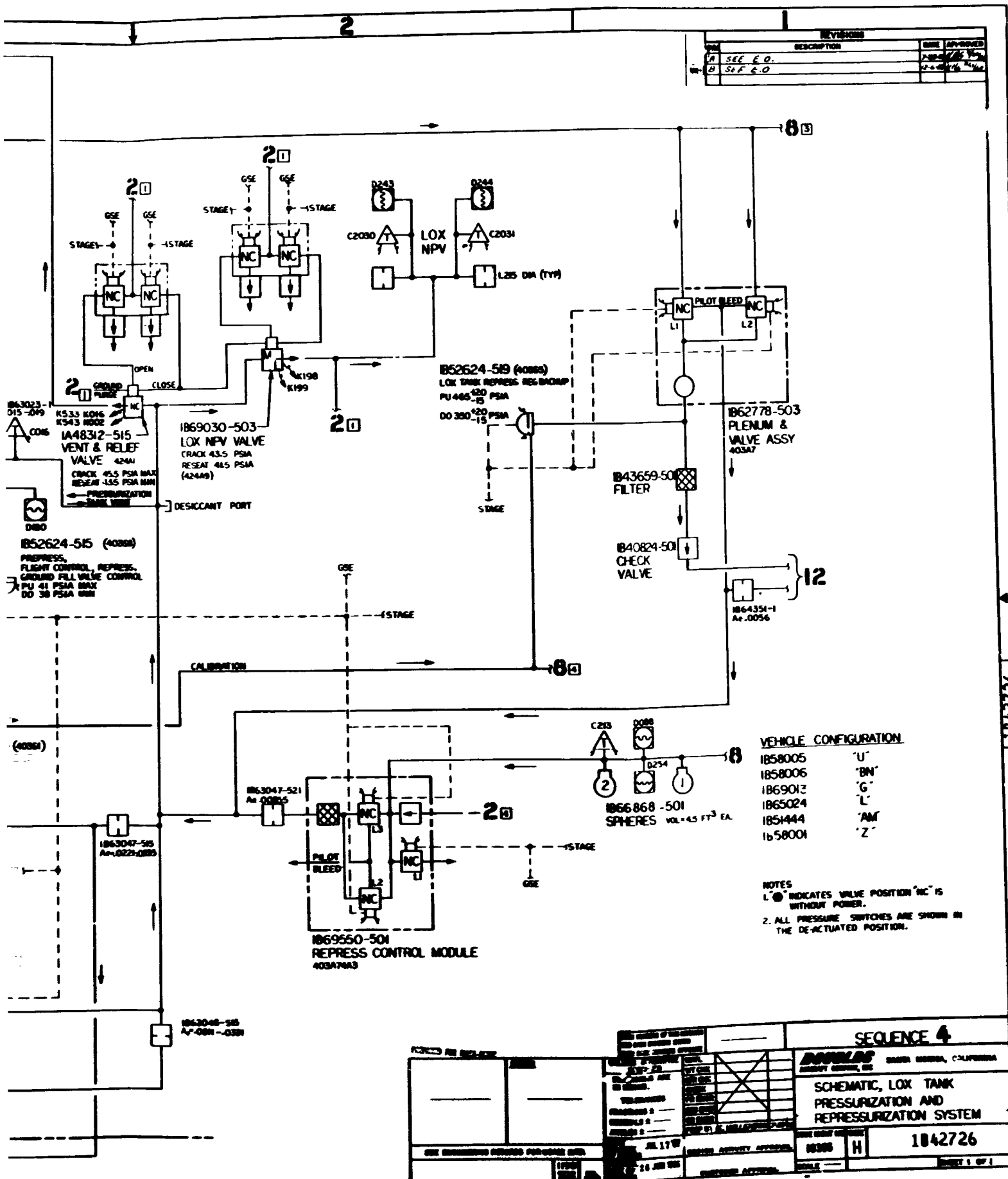
2 Figure 11-1. Schematic, LOX Tank Pressurization and Repressurization System
