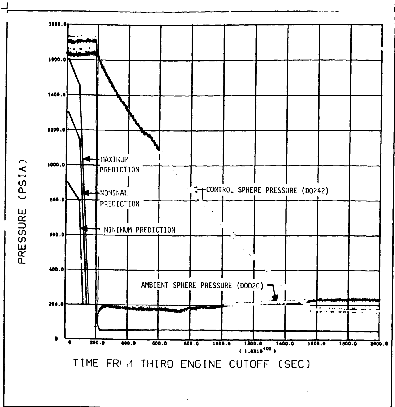
Figure 9-25. Control Sphere Pressure -- Passivation
