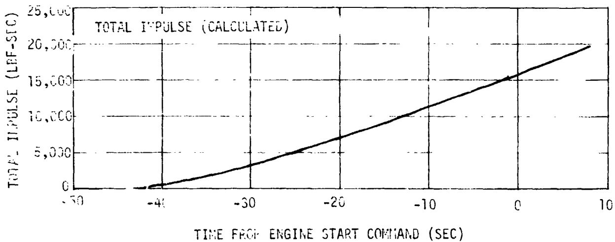
Figure 9-28. Fuel Leak Characteristics - Third Burn (Sheet 2 of 2)
