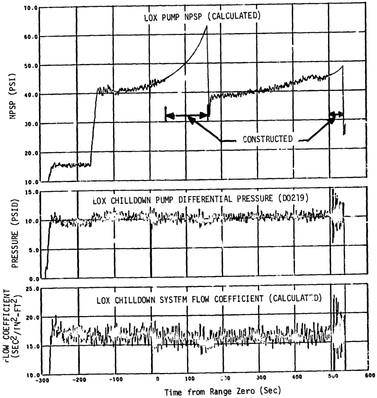
Figure 11-18. LOX Pump Chillover System Performance - Boost and First Burn (Sheet 1 of 2)
