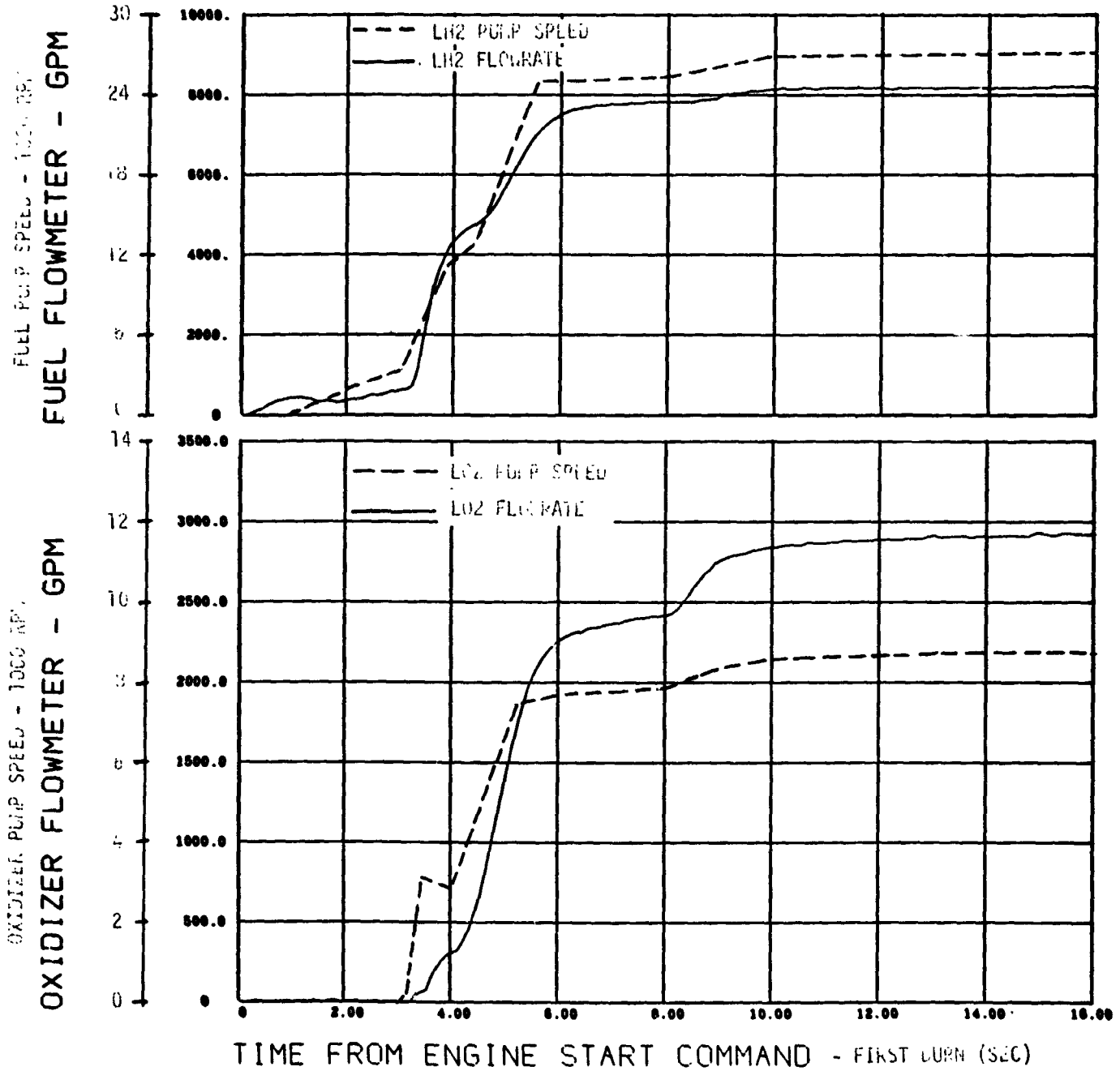
Figure 9-31. LOX and LH2 Pump Performance (Sheet 1 of 3)
