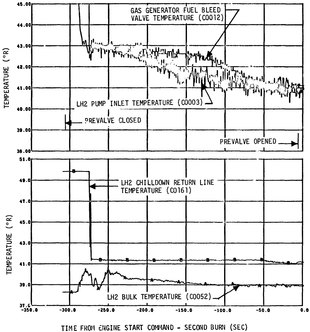
Figure 12-17. LH2 Pump Chilldown System Performance - Second Burn (Sheet 2 of 2)
