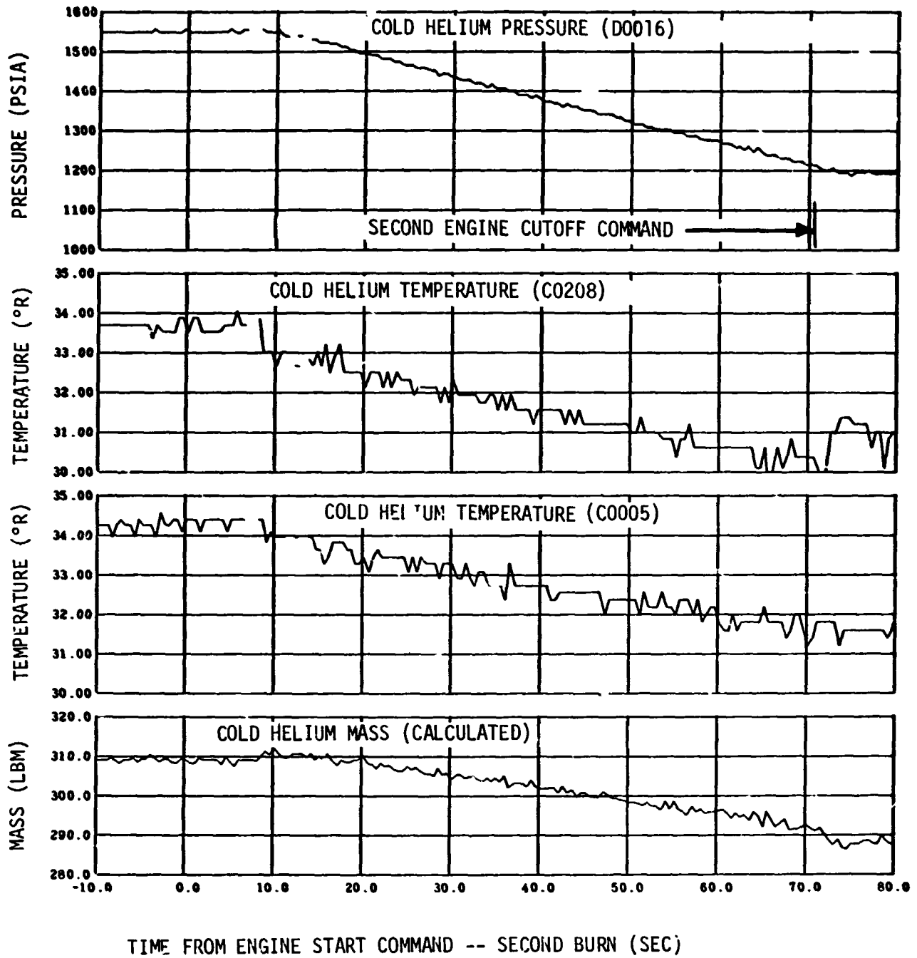
Figure 11-7. Cold Helium Supply -- Second Burn
