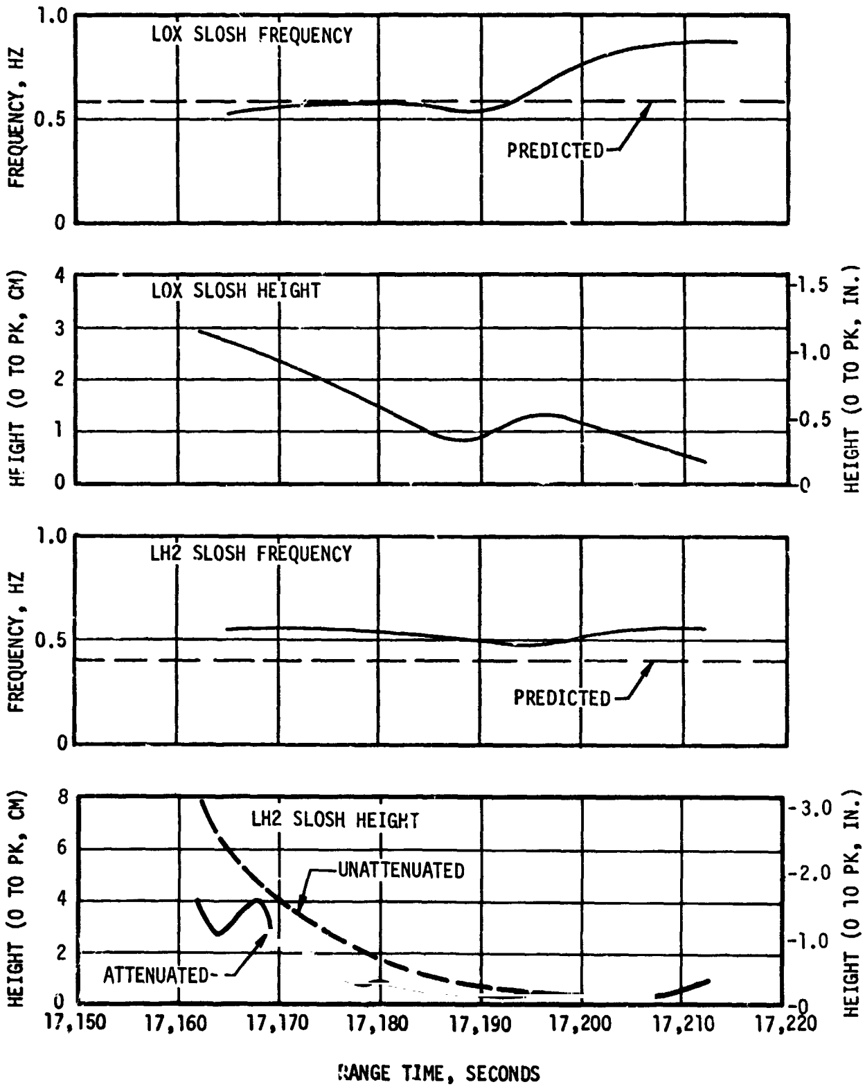
Figure 21-8. S-IVB Slosh Frequencies and Height during Second Burn
