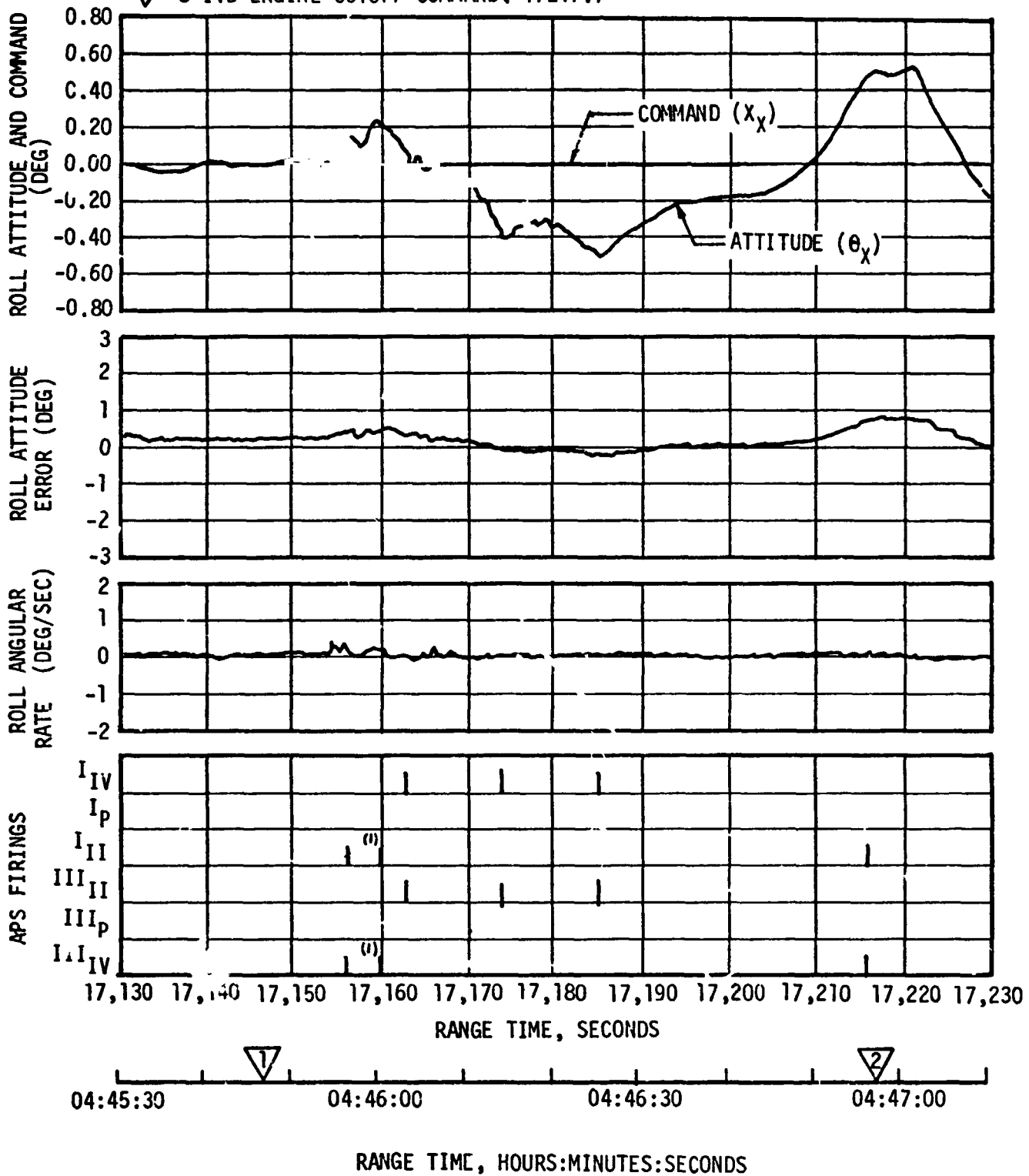
Figure 21-7. Roll Attitude Control During S-IVB Second Burn
