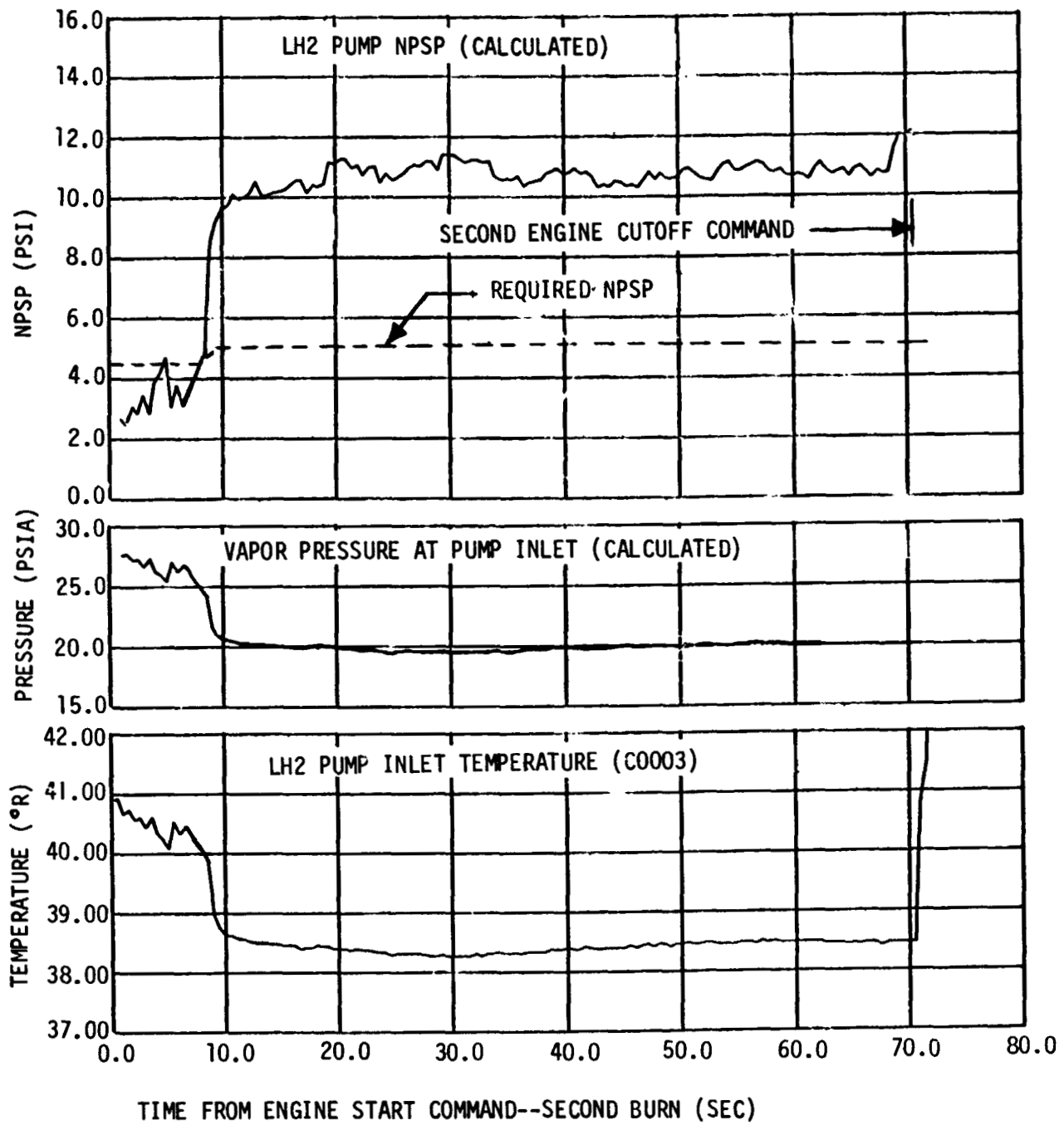
Figure 12-23. LH2 Pump Inlet Conditions--Second Burn (Sheet 1 of 2)
