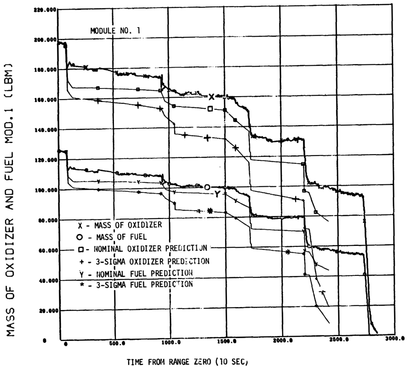
Figure 14-9. APS Module 1 Propellant Masses
