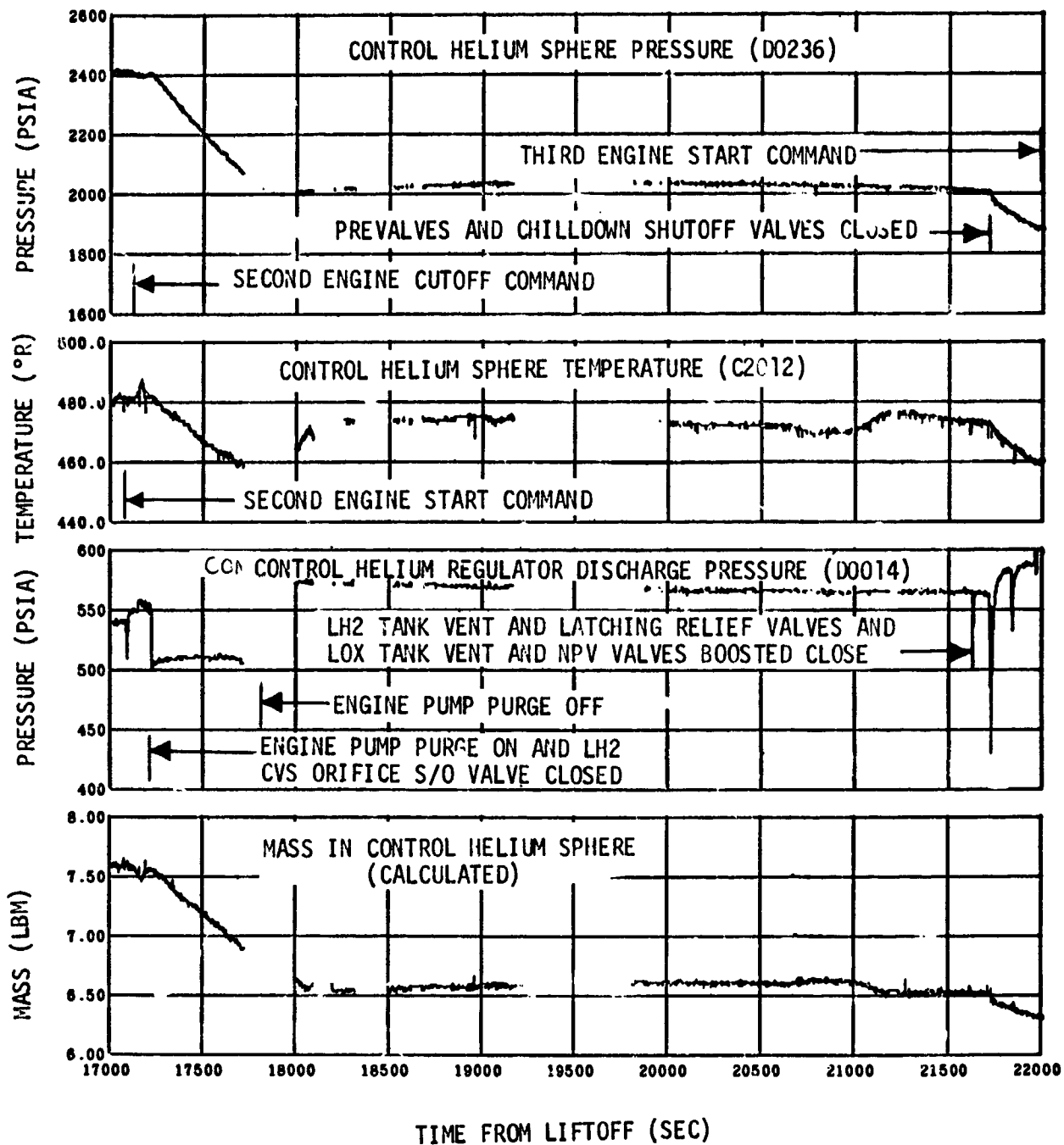
Figure 15-5. Pneumatic Control and Purge System Performance -- Intermediate Orbit
