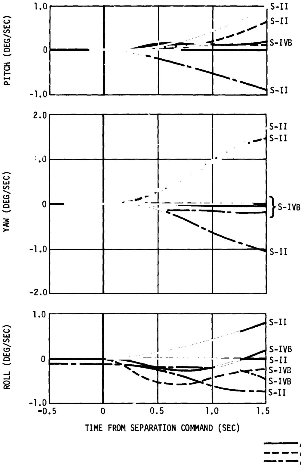
Figure 17-2. Angular Velocity
