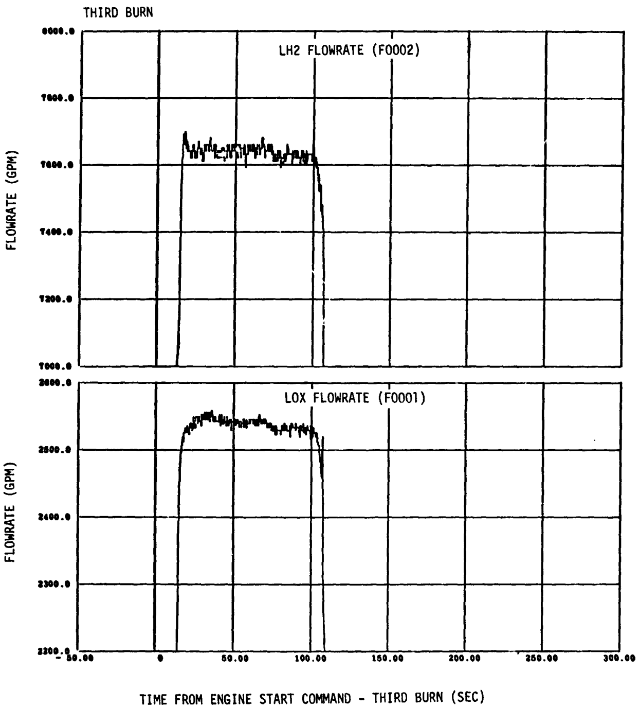
Figure 9-34. J-2 Engine Pump Flowrates (Sheet 4 of 4)
