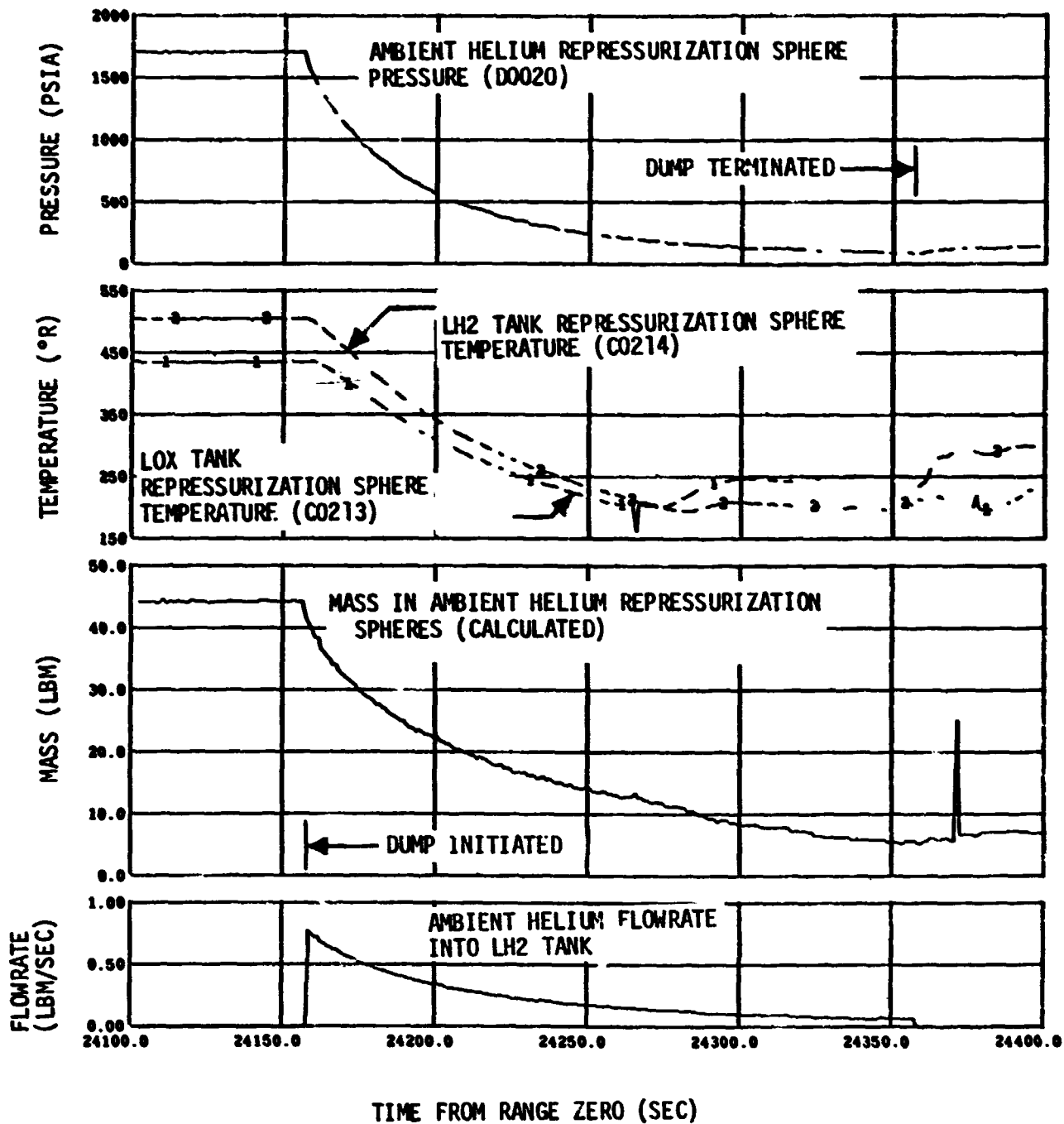
Figure 25-1. Ambient Repressurization Helium Dump
