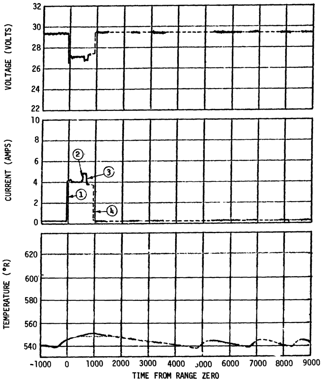
Figure 19-2. Forward Battery No. 2 Performance (Sheet 1 of 3)
