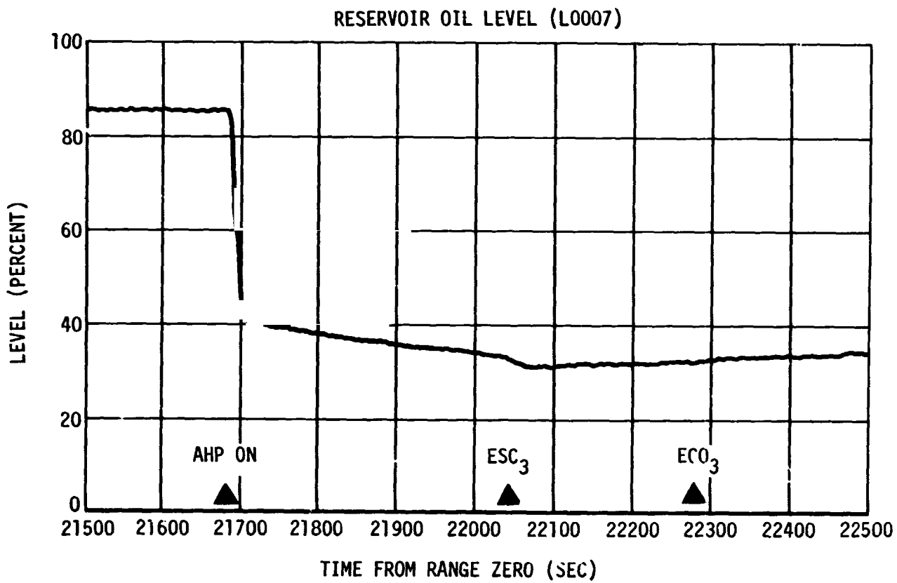
Figure 22-8. Hydraulic System - Third Burn (Sheet 2 of 4)
