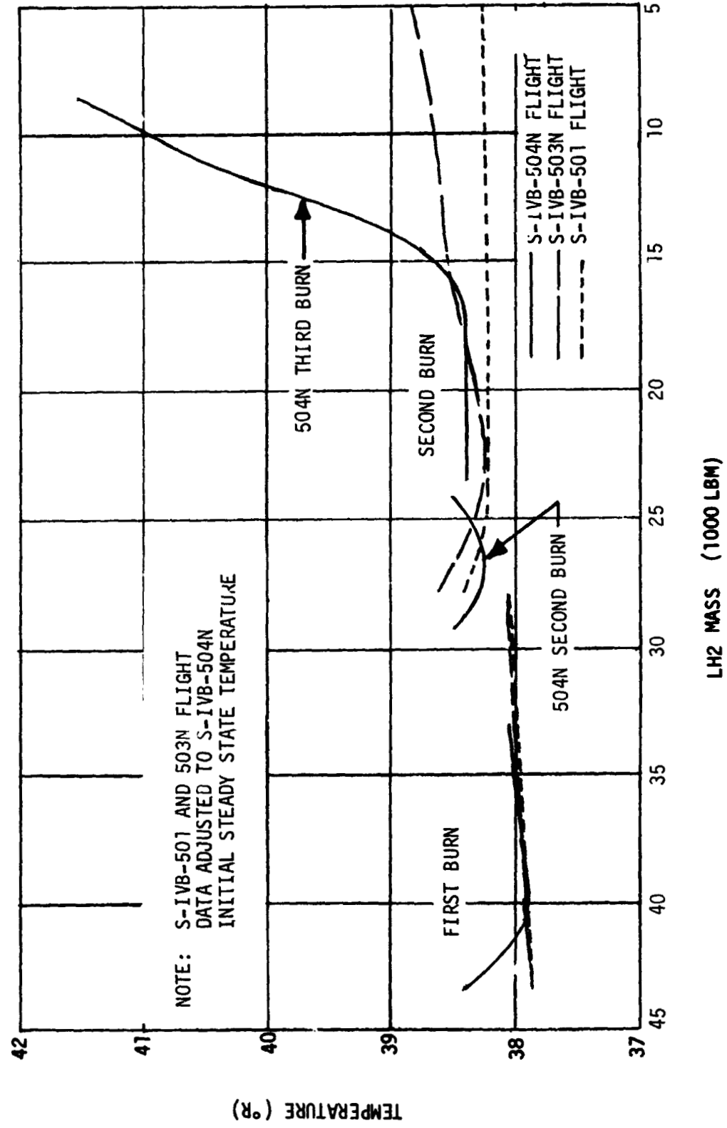
Figure 12-22. Effect of LH2 Mass Level on LH2 Pump Inlet Temperature
