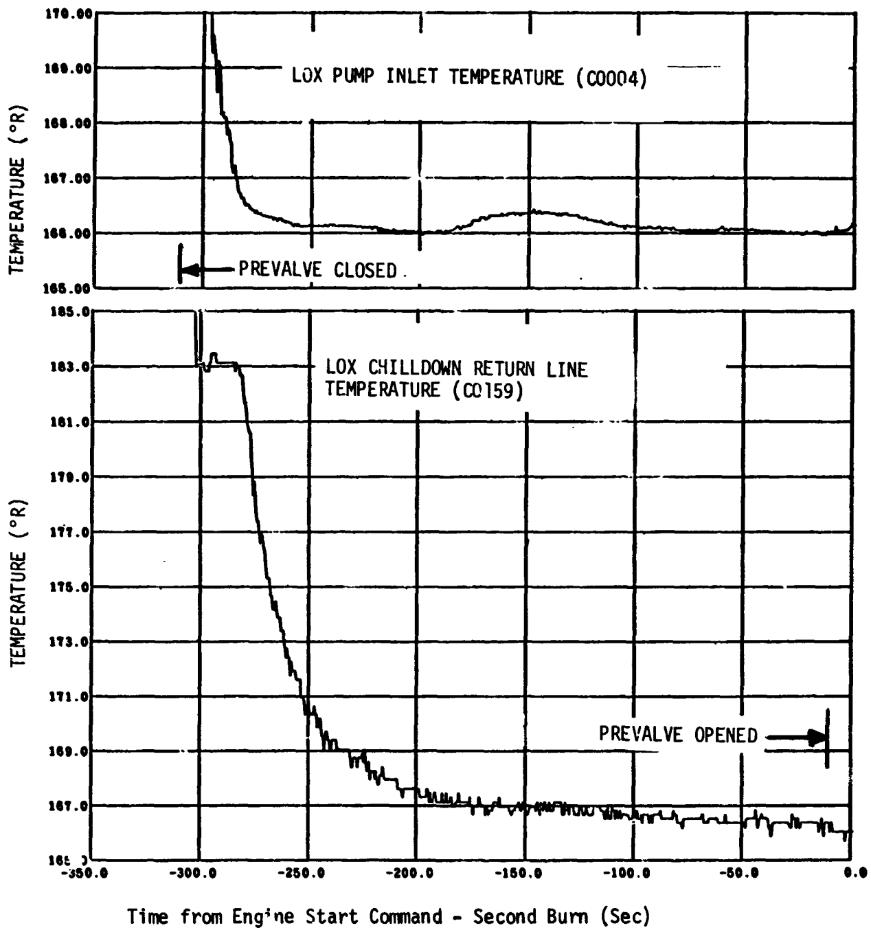
Figure 11-19. LOX Pump Chilldown System Operation - Second Burn (Sheet 2 of 2)
