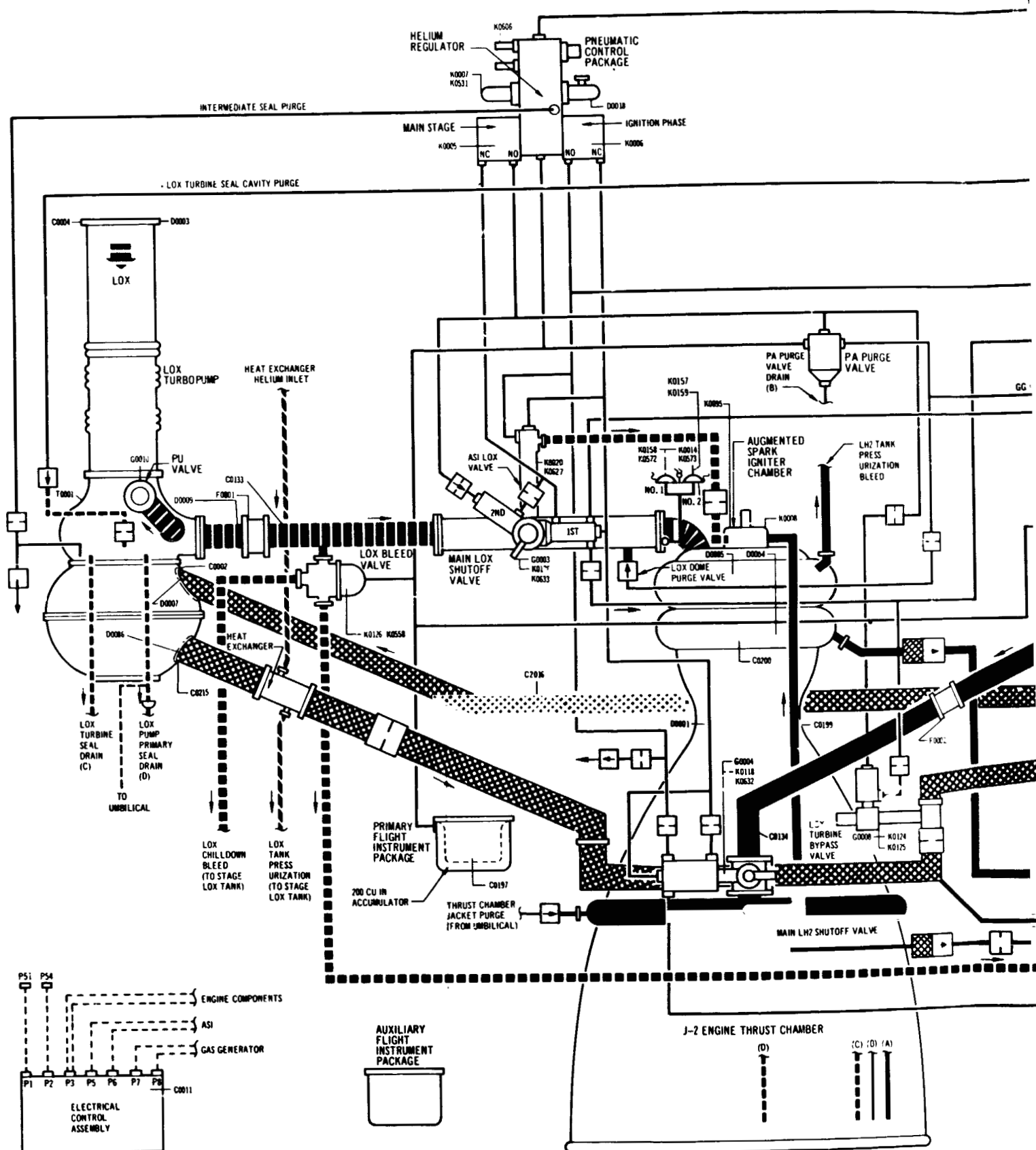
Figure 9-1. J-2 Engine System and Instrumentation
