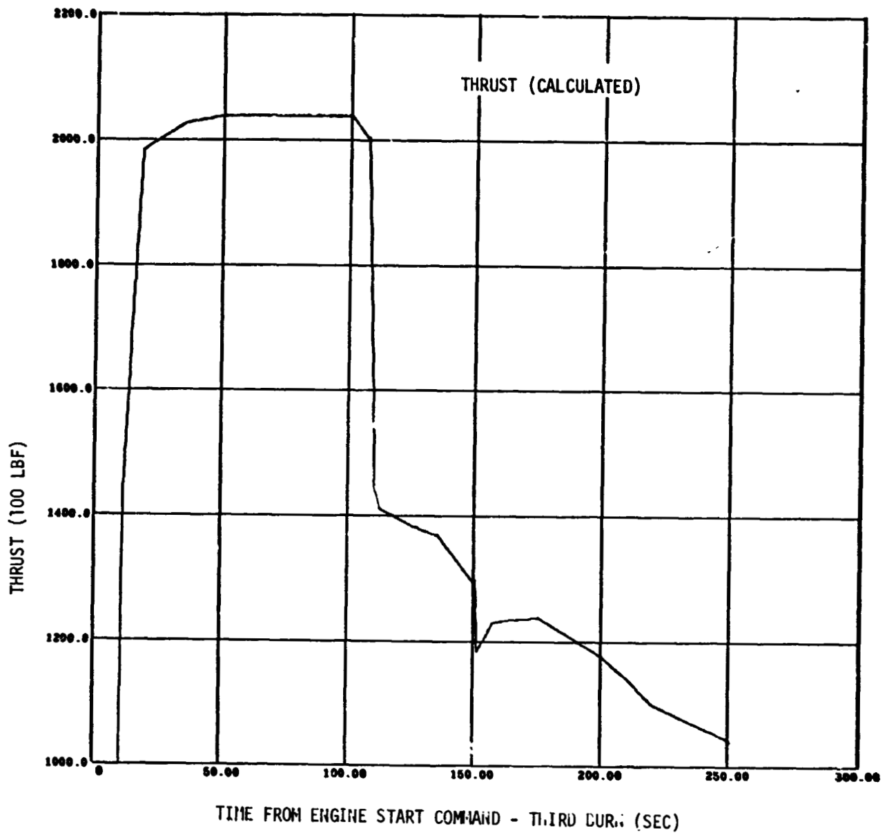
Figure 9-40 Engine Steady-State Performance - Third Burn (Sheet 3 of 3)
