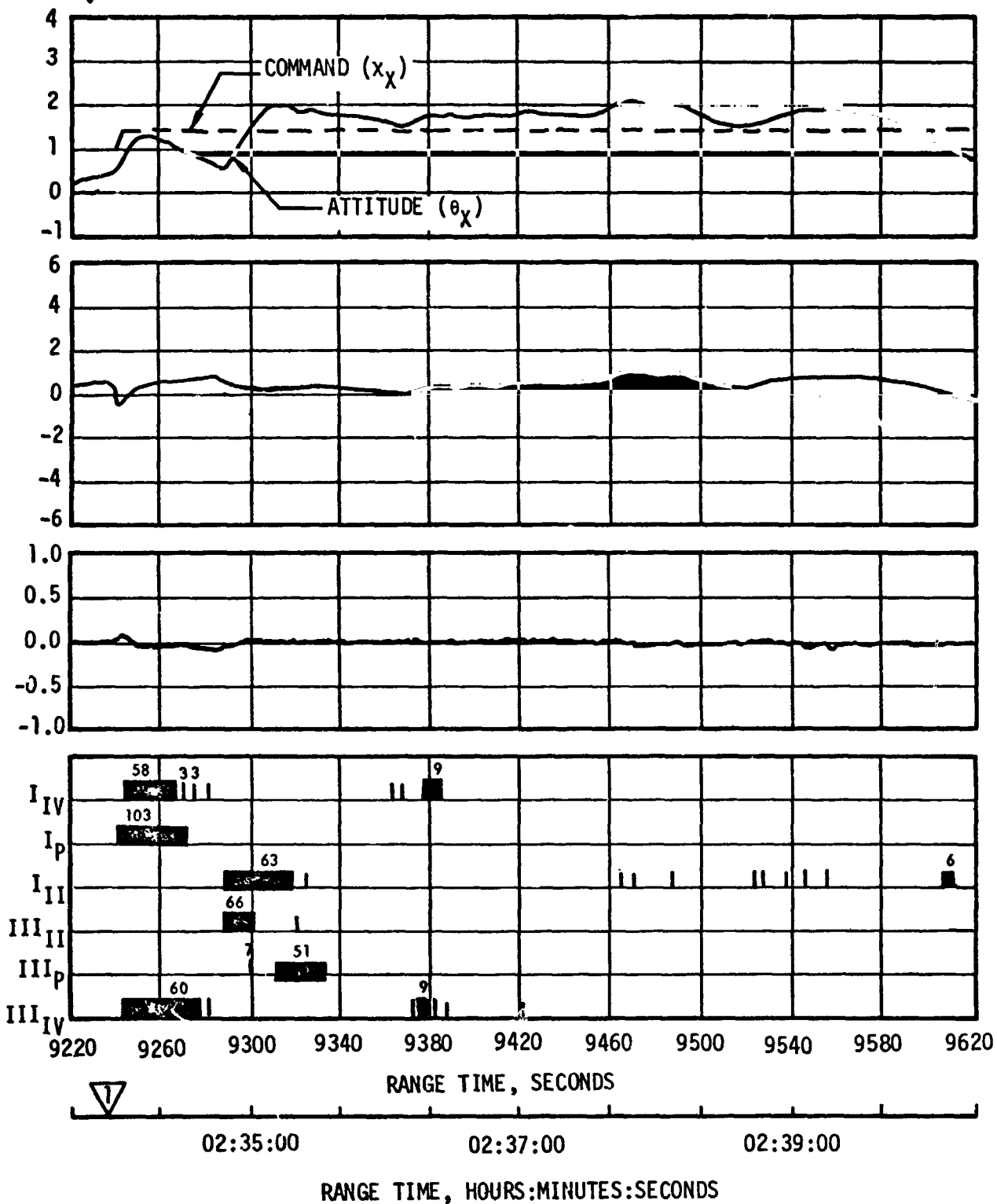
Figure 21-18. Roll Attitude Control during TD&E Maneuver
