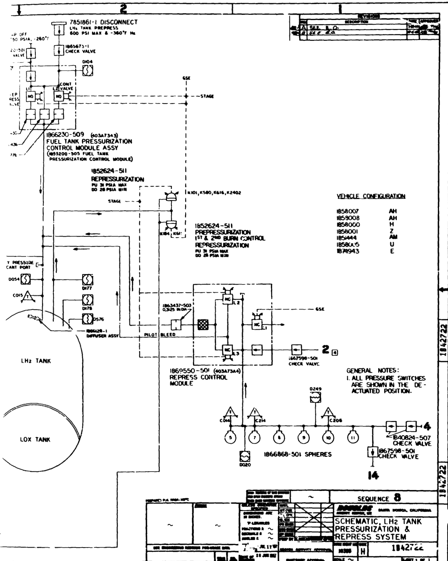
Figure 12-1. Schematic, LH2 Tank Pressurization and Repress System
