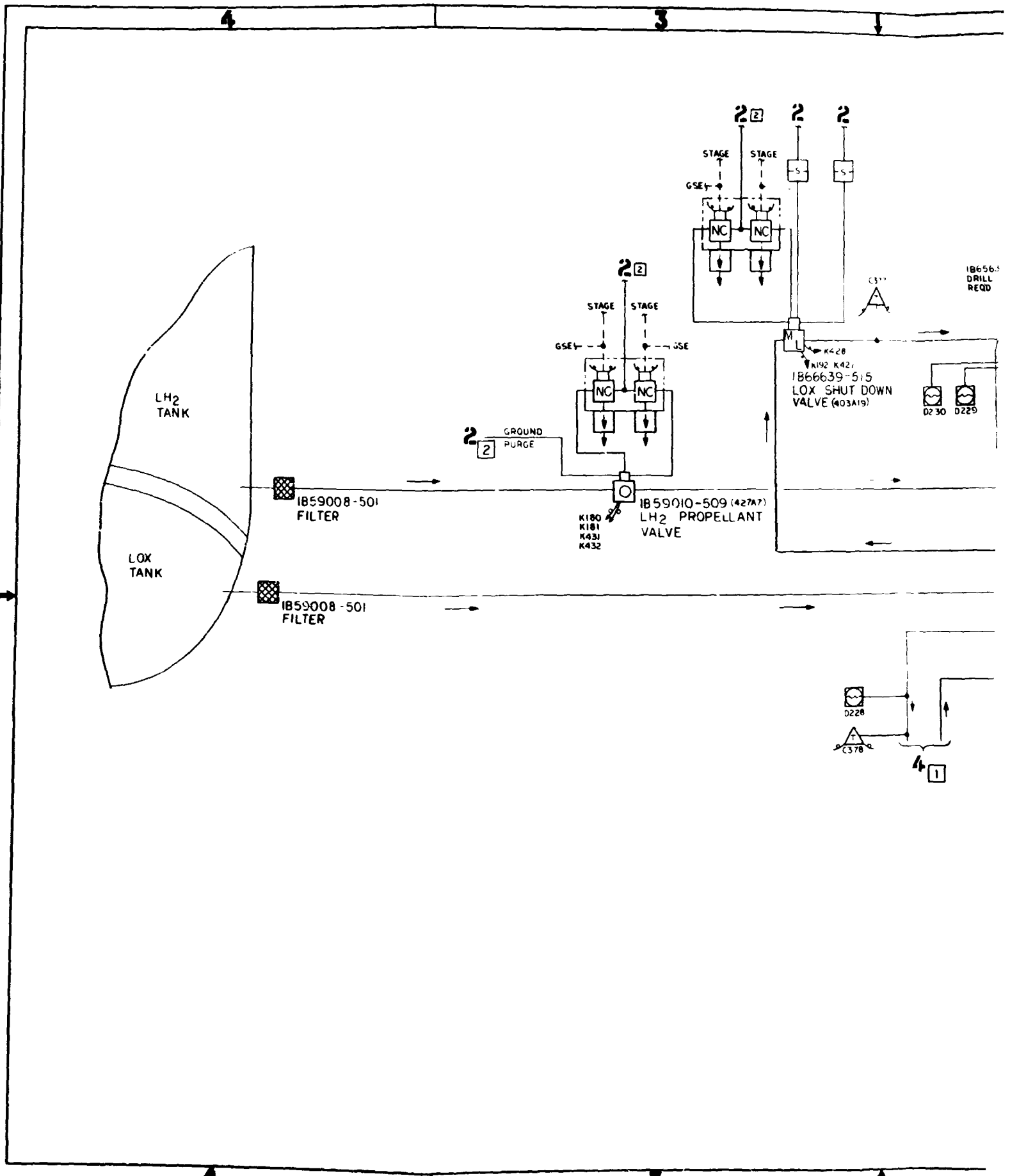
Figure 13-1. Schematic, Oxygen Hydrogen Burner
