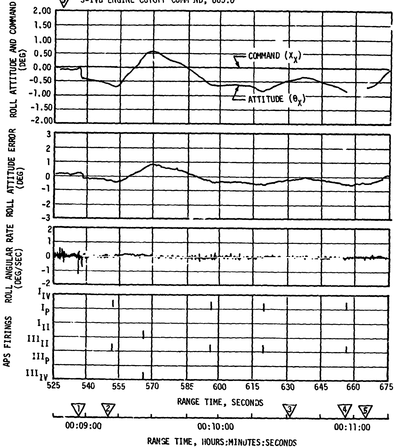
Figure 21-3. Roll Attitude Control during S-IVB First Burn
