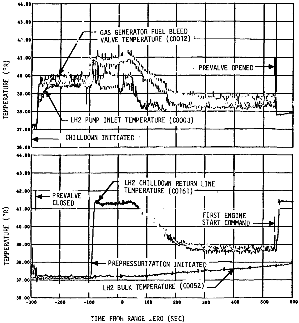
Figure 12-15. LH2 Pump Chilldown Performance - First Burn (Sheet 2 of 2)
