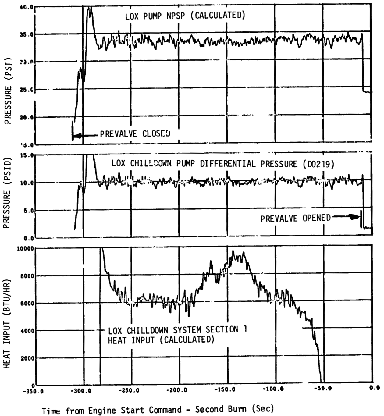
Figure 11-20. LOX Pump Chilldown System Performance - Second Burn (Sheet 1 of 2)
