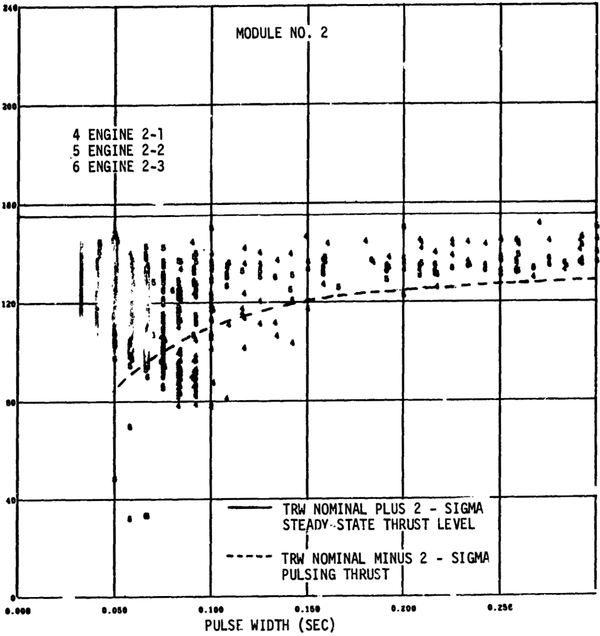
Figure 14-17. APS Thrust ( Module 2 )
