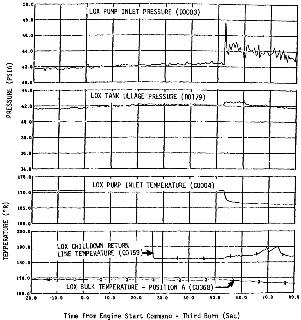
Figure 11-28. LOX Supply Conditions During Extended Fuel Lead - Third Burn
