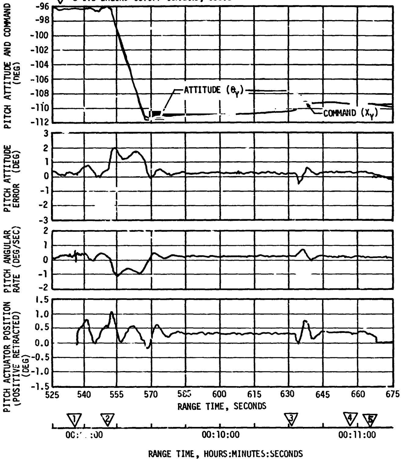
Figure 21-1. Pitch Attitude Control During S-IVB First Burn
