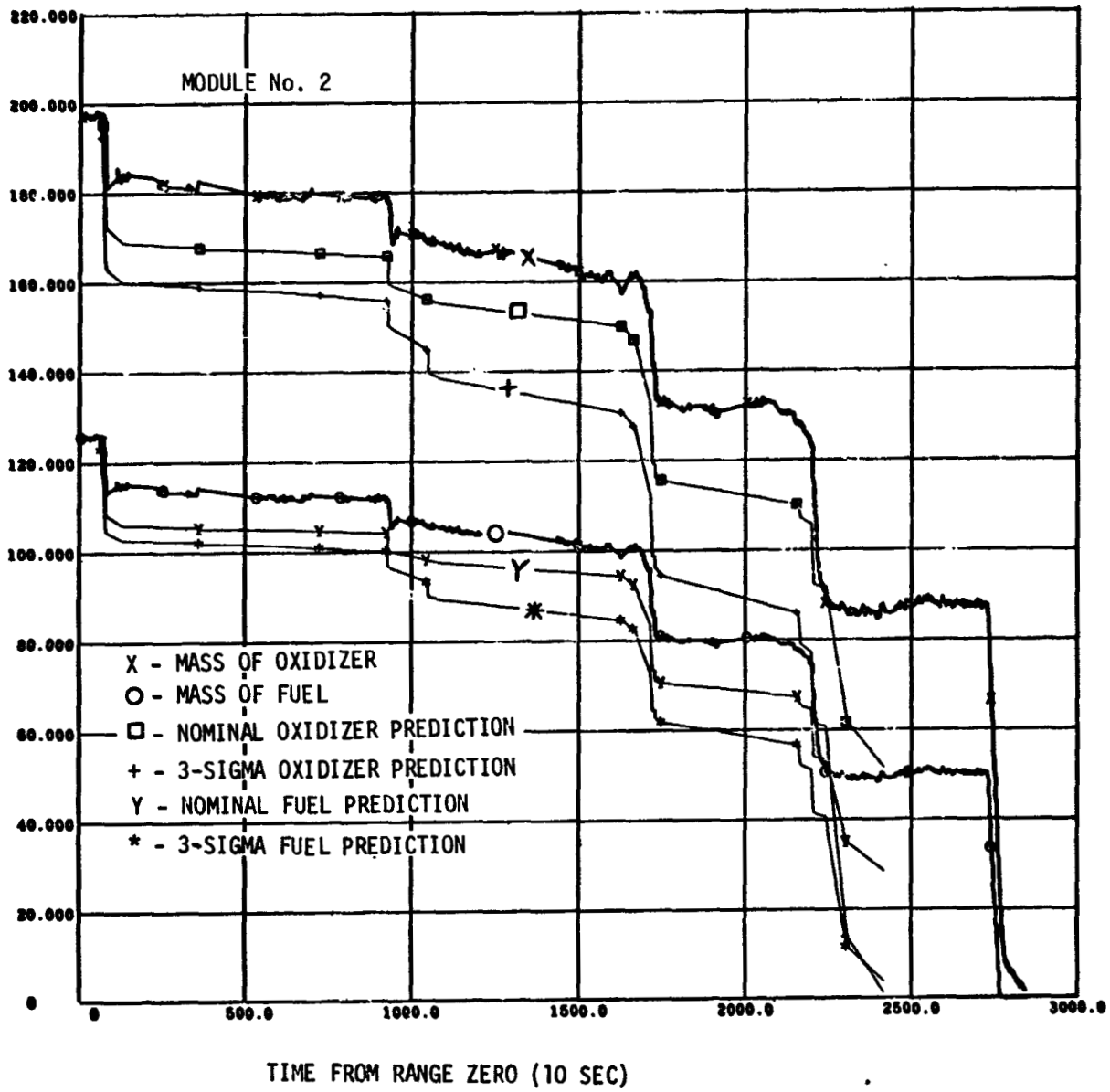
Figure 14-11. APS Module 2 Propellant Masses
