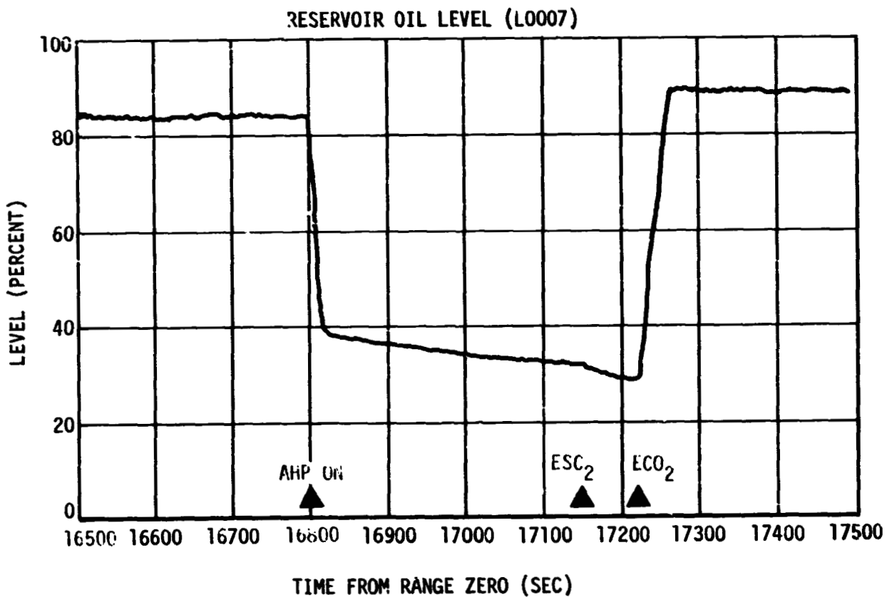
Figure 22-6. Hydraulic System - Second Burn (Sheet 2 of 3)
