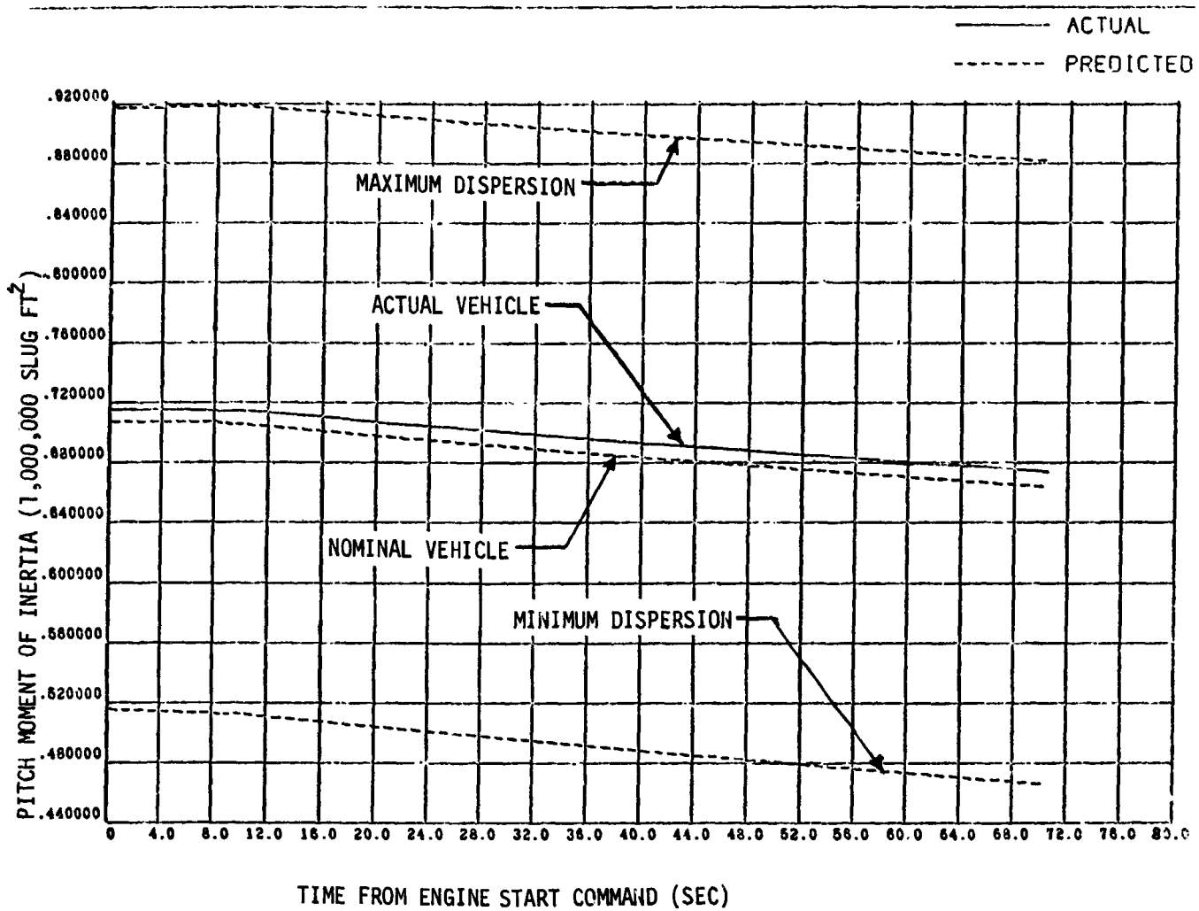
Figure 8-11. Third Flight Stage Vehicle Pitch Moment of Inertia (Second Burn).
