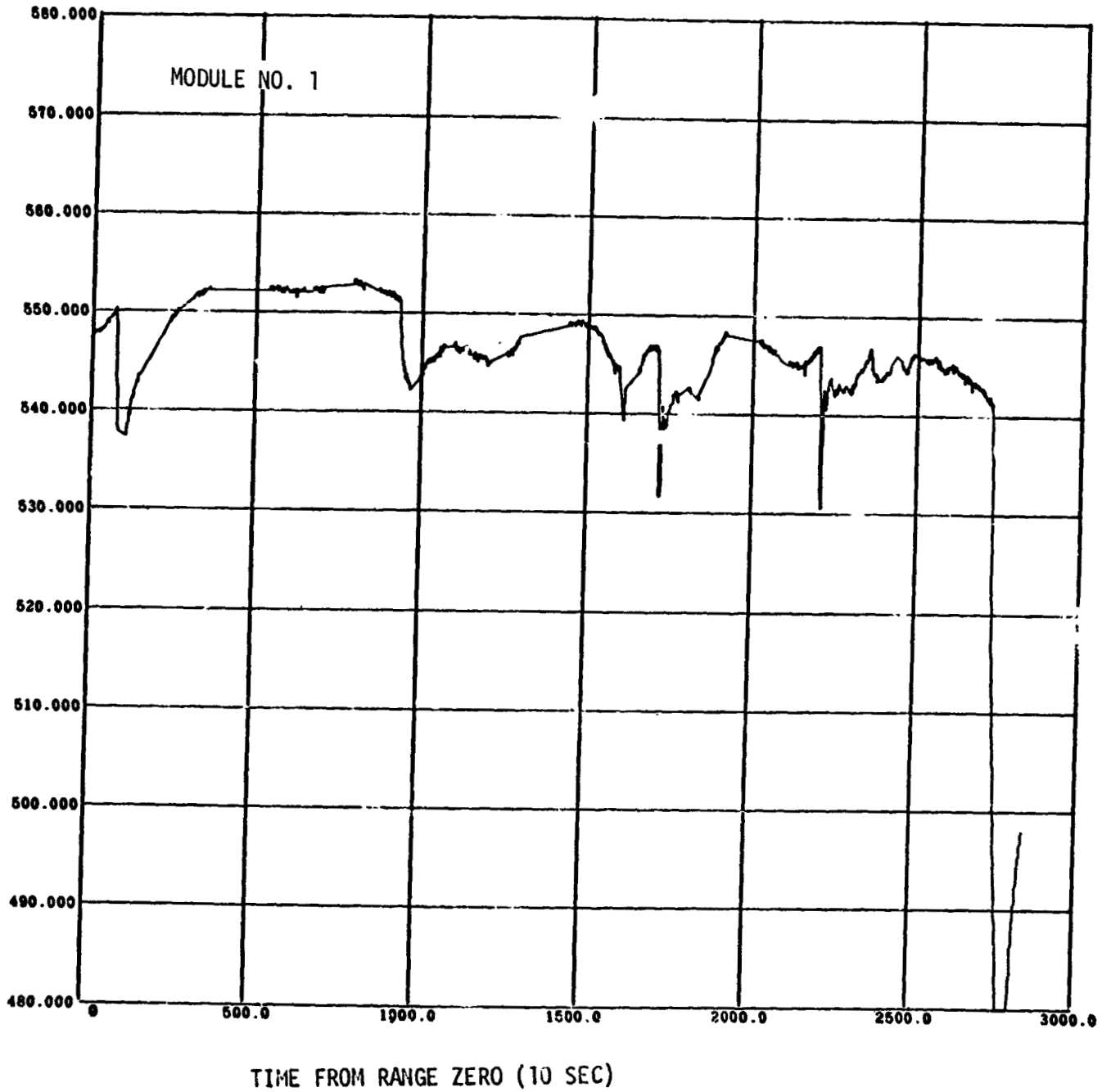
Figure 14-2. APS Module 1 Helium Bottle Temperature
