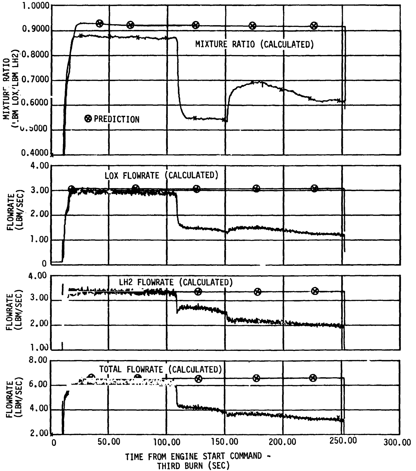
Figure 9-53. Gas Generator Performance (Sheet 3 of 3)
