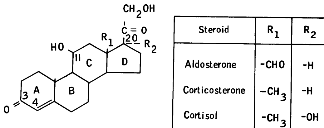
Figure 7-7.- Structures of aldosterone, corticosterone, and cortisol. The C 18 (R 1 ) aldehyde of aldosterone exists in solution in a hemiacetal link with the C 11 (from ref. 7-8).
