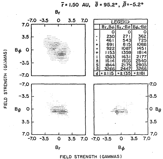
Figure 9. Joint distributions of pairs of component variables from measurements taken near 1.5 AU, Bartels' solar rotation 1804, May 22-June 17, 1965 by Mariner 4 [Coleman et al. , 1969]
