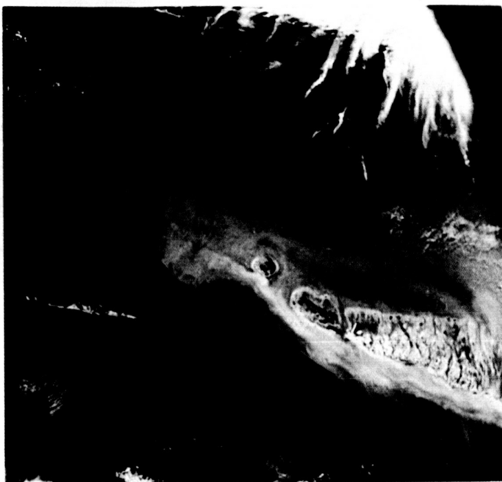
Figure 16. Apollo IX photograph of West Florida keys in natural color.
