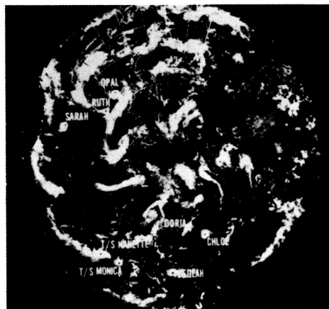
Figure 20. ESSA V tracks eight major storms on September 14, 1967.
