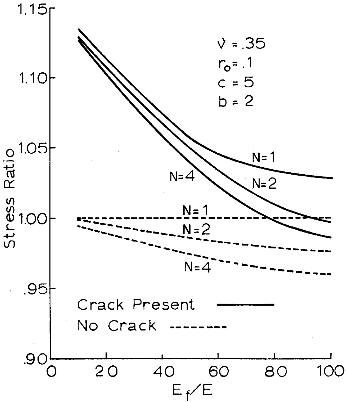
Figure 12. The ratio of the maximum filament stress in a crack and in an uncracked matrix to that for a single filament in an uncracked matrix.
