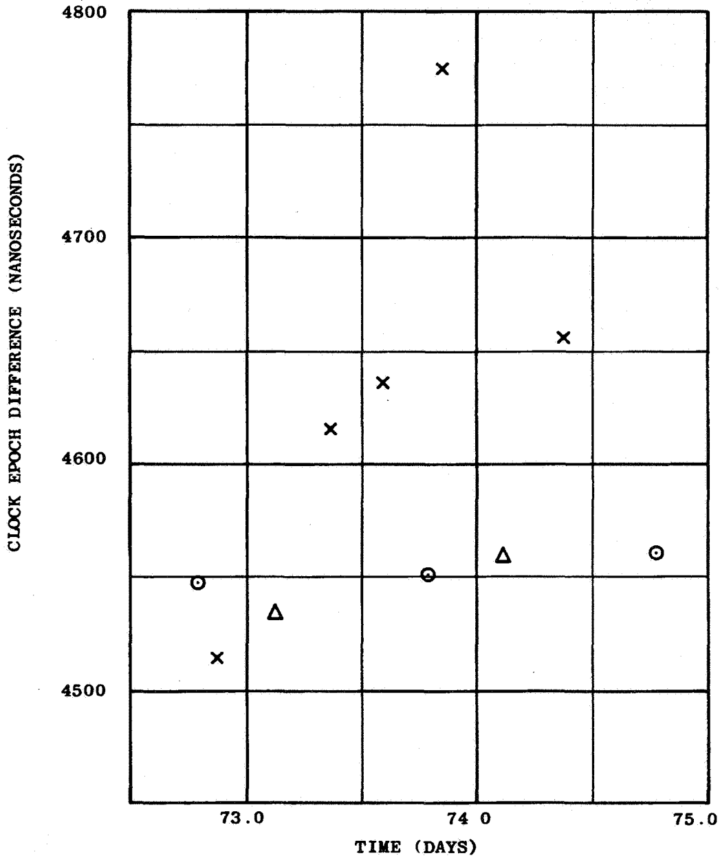
FIG. 4 GLOBAL CLOCK SYNCHRONIZATION DATA
