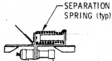
EXPLOSIVE NUT BOLT CATCHER
