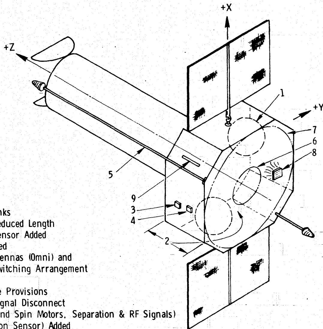
Figure 2-32. Spin/Despin SSUS-Launched EO-09A
