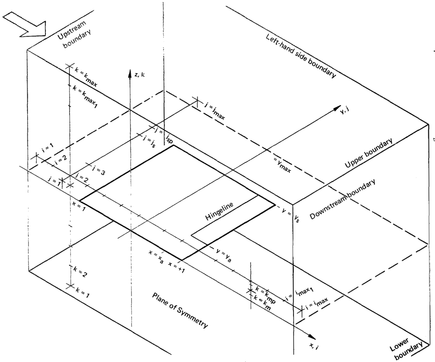
Figure 18. — Schematic of Mesh for Three-Dimensional Problem
