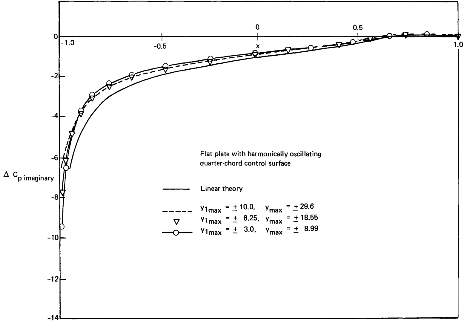
Figure F15. — Comparison of Solutions With Variation of Location of Upper and Lower Boundaries
