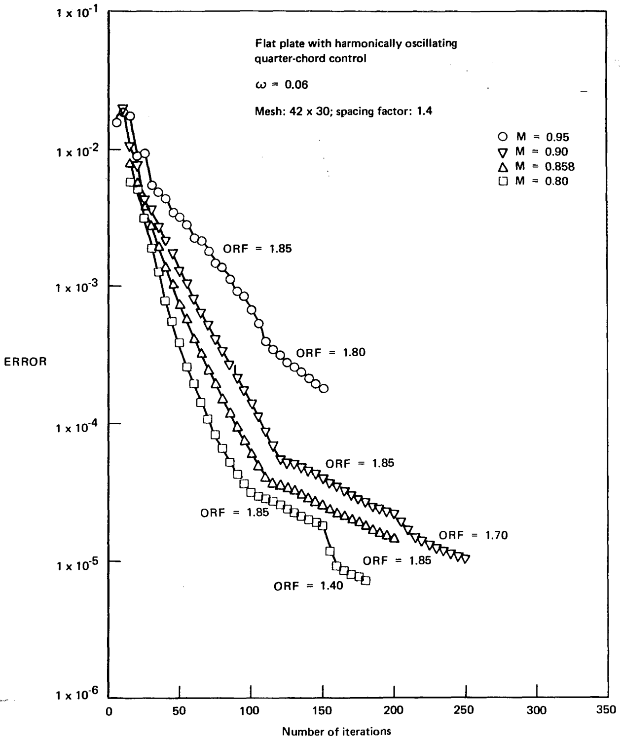
Figure F2— Variation of Solution Convergence With Mach Number
