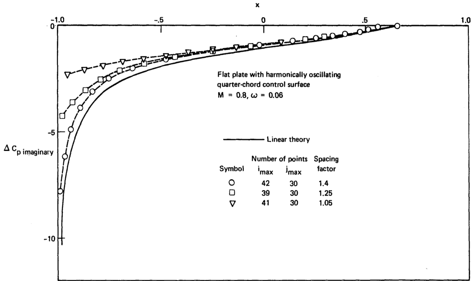
Figure F9. — Comparison of Solutions for Different Mesh-Point Spacings
