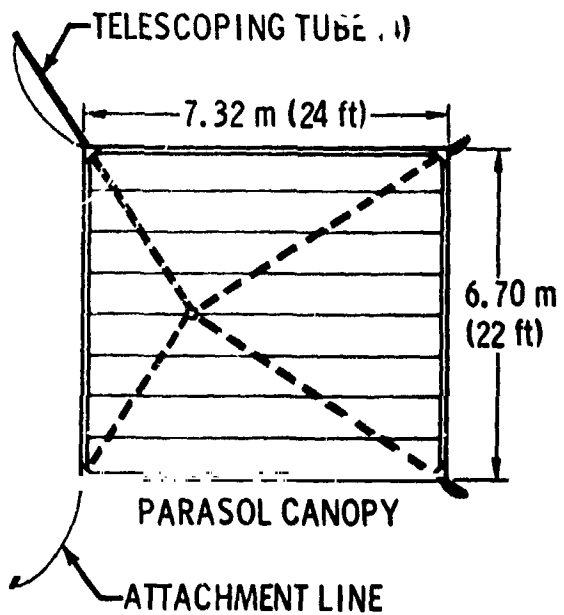
Figure 5. Parasol Canopy Details
