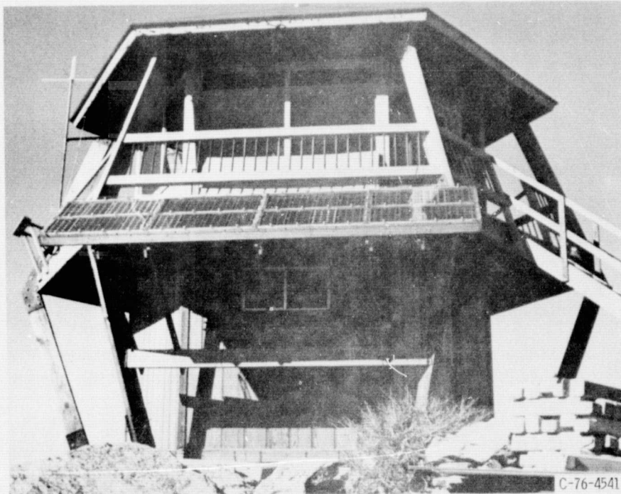
Figure 6. - U. S. Forest Service fire lookout - Pilot Peak, Plumas National Forest, California.
