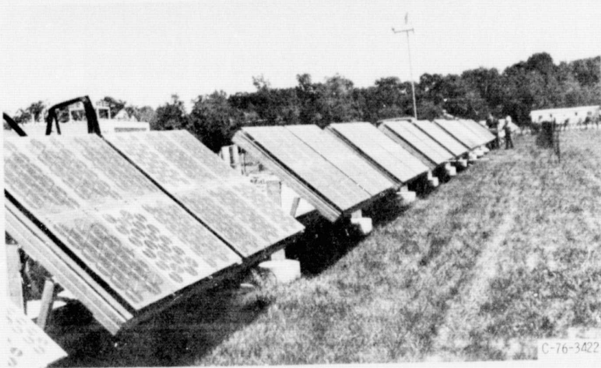
Figure 7. - Photovoltaic System Test Facility: NASA-Lewis Research Center, Cleveland, Ohio.
