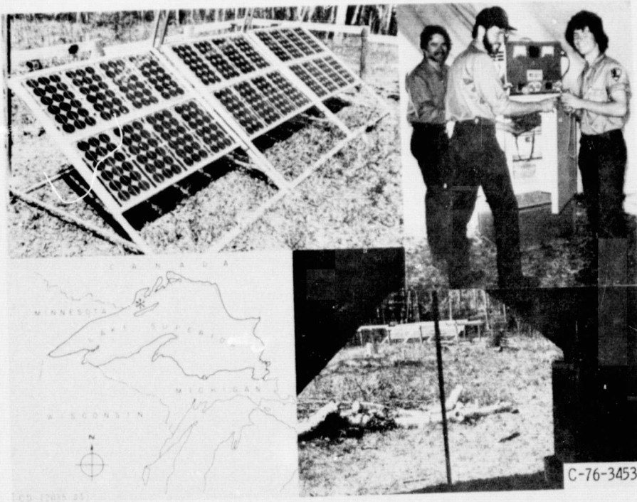
Figure 1. - Photovoltaic powered refrigerator used by park personnel - Isle Royale National Park, Michigan.
