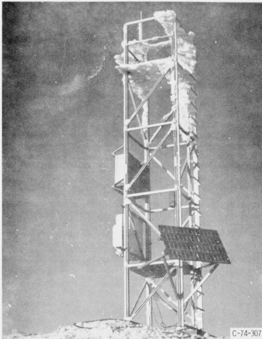
Figure 4. - National Weather Service remote weather station (RAMOS) - Mammoth Mountain, California. Similar to six additional units planned for ERDA application tests.
