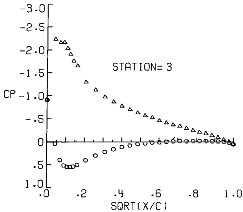
Figure 7.- Pressure distributions at sweep angle of 40^\circ .
