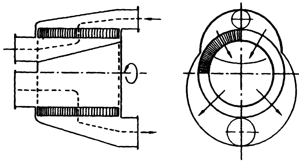
ROTARY HEAT EXCHANGER
