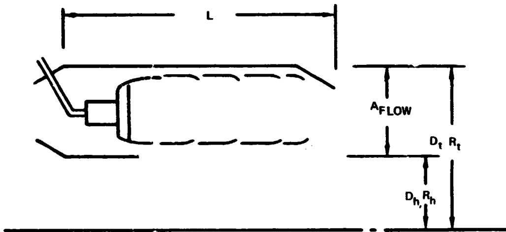
Figure 14. Burner Schematic
