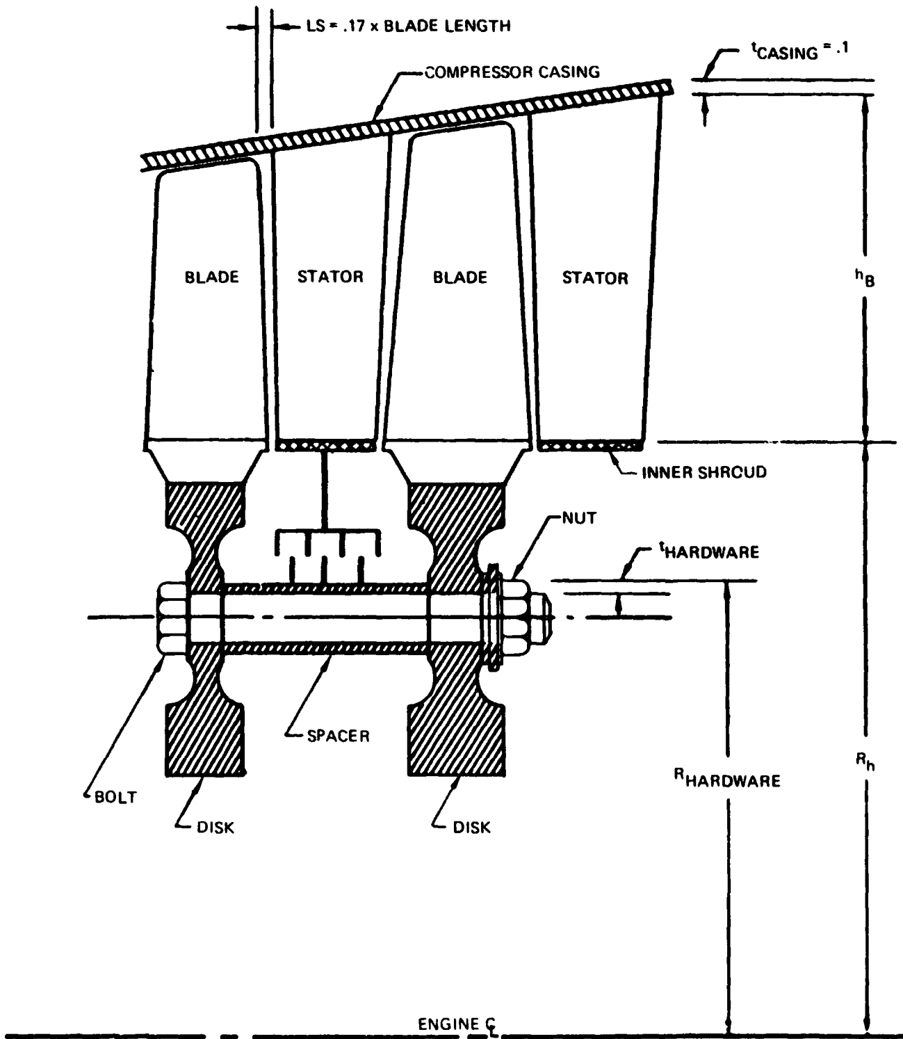
Figure 10. Stage Components
