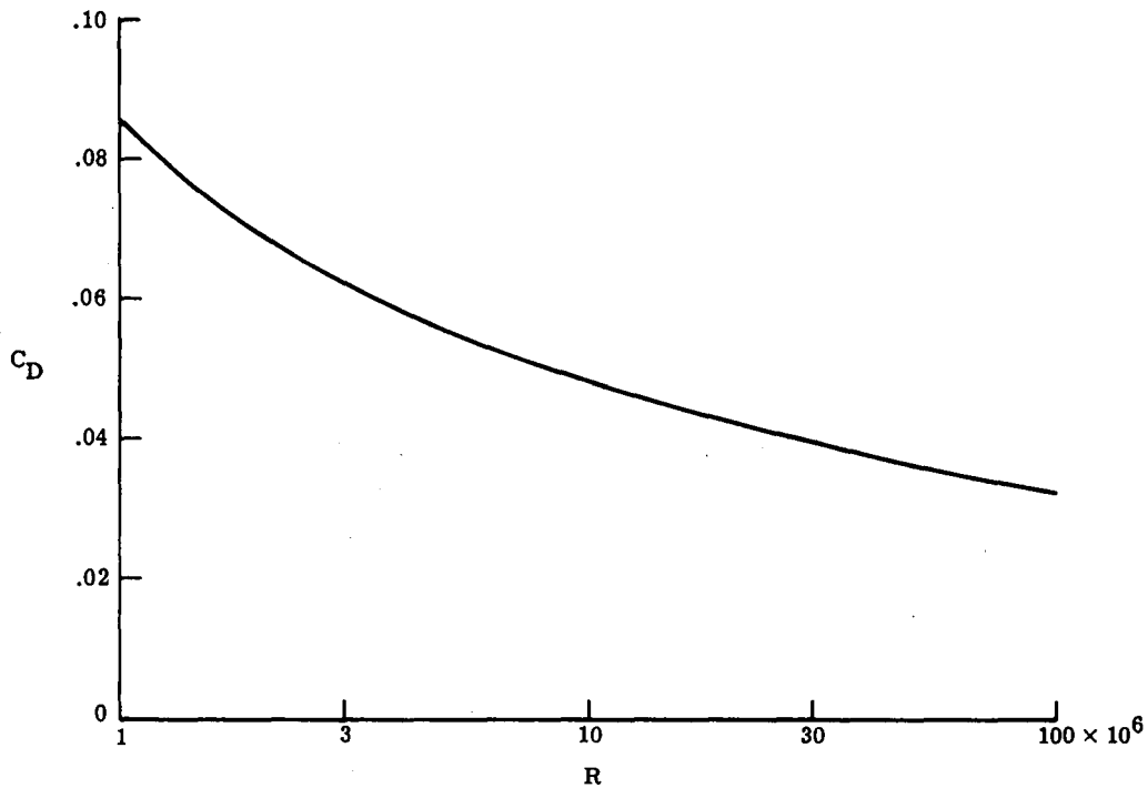
Figure 9.- Drag coefficient versus Reynolds number for energy efficient transport (EET) medium vane, double-slotted flap. M_\infty = 0.2 ; \alpha = 5.0^\circ .
