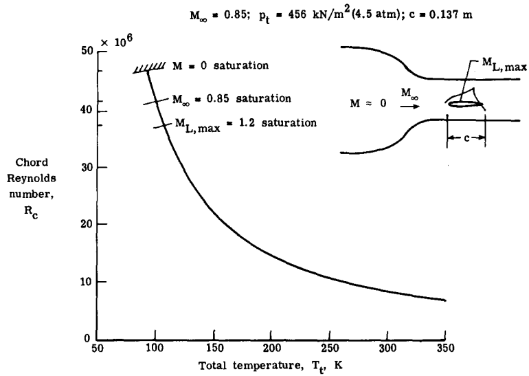
Figure 5.- Potential benefits of operation below saturation temperature.
