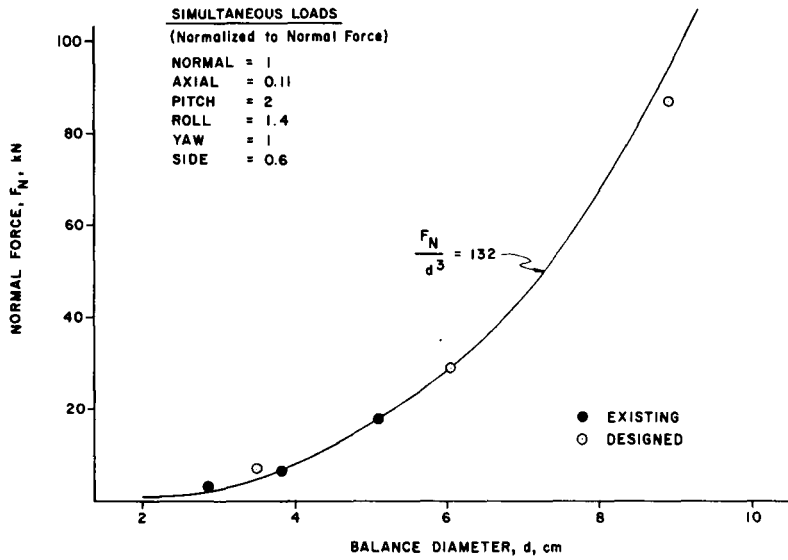
Figure 3.- Balance load as a function of diameter.
