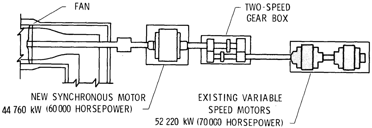
Figure 13.- Schematic of National Transonic Facility drive system.
