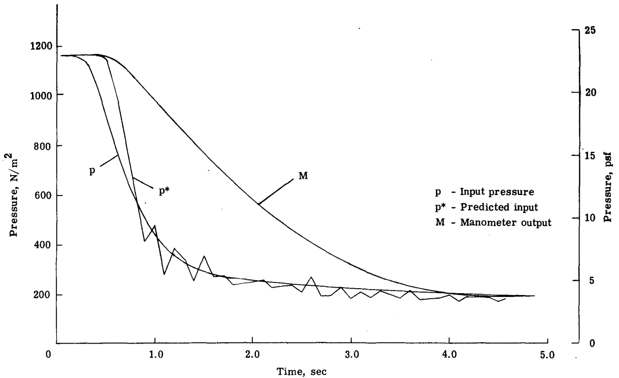
Figure 14.- Step-response data.
