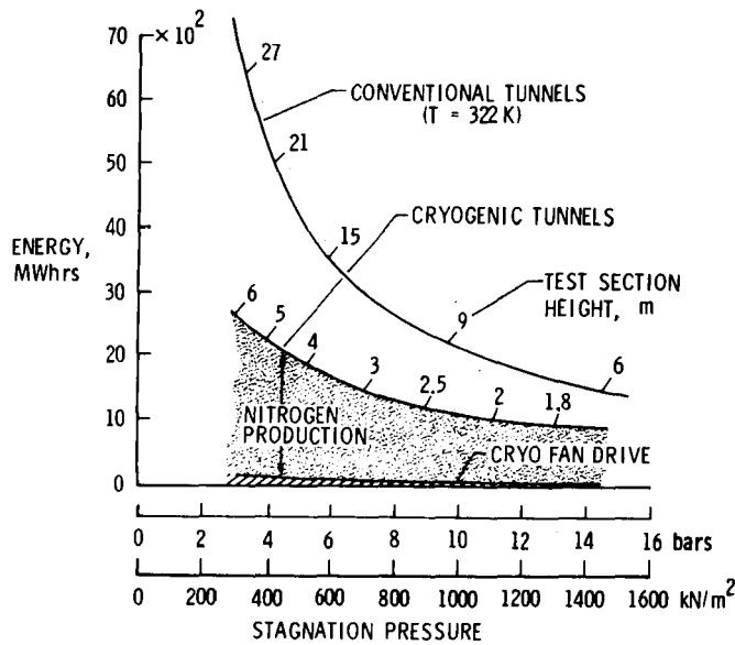
Figure 3.- Comparison of the energy consumed in 1 hour of operation for conventional and cryogenic tunnels, R_{\bar{c}} = 120 \times 10^6 ; M = 1.0 ; \bar{c} = 0.1 test section height.
