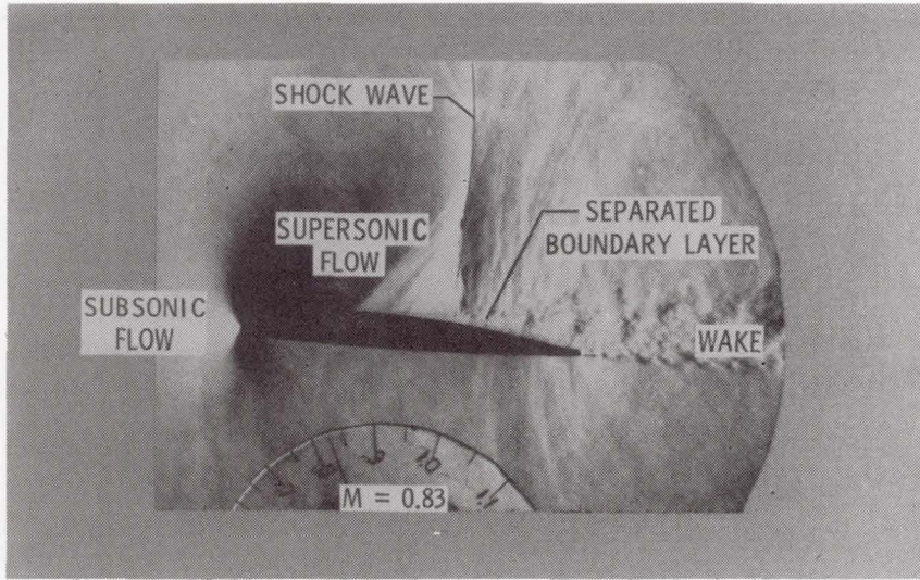
Figure 9.- Complex transonic flows vary with Reynolds number.
