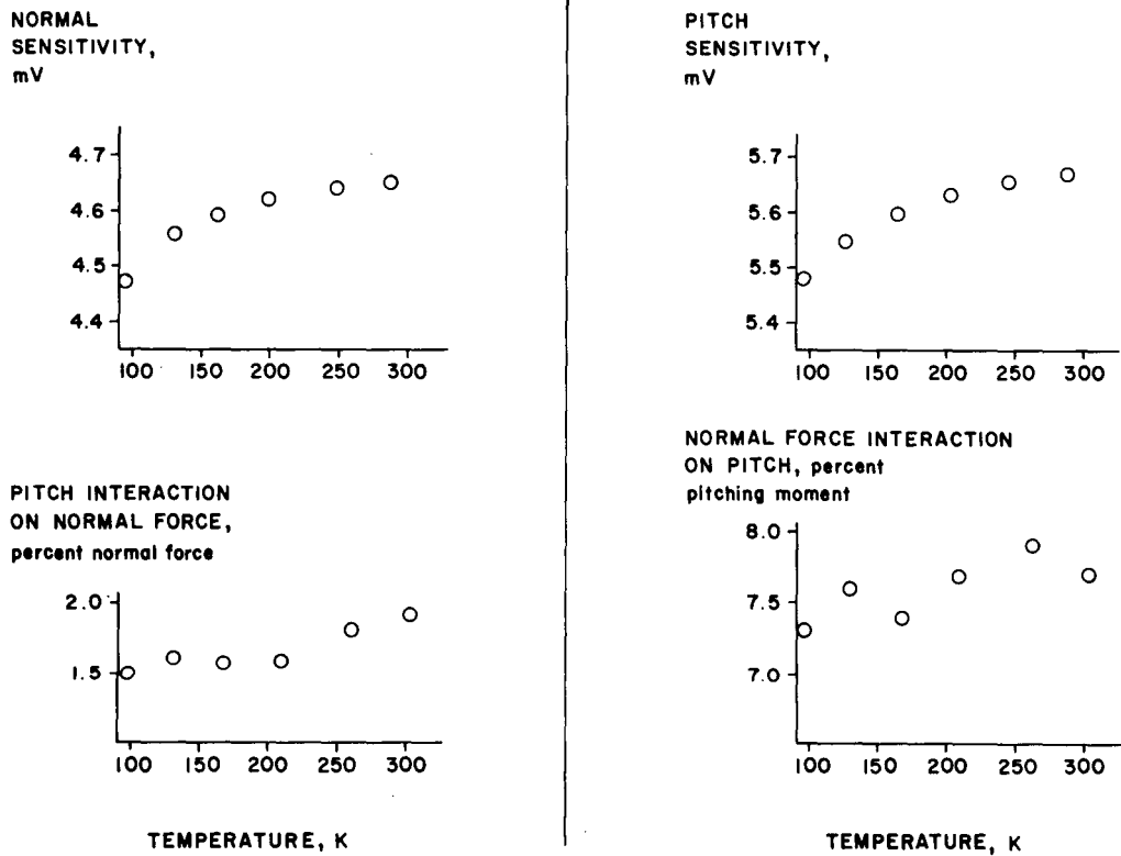
Figure 5.- Balance laboratory calibration as a function of temperature.
