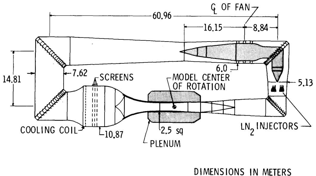
Figure 10.- Lines of the aerodynamic circuit of the National Transonic Facility.
