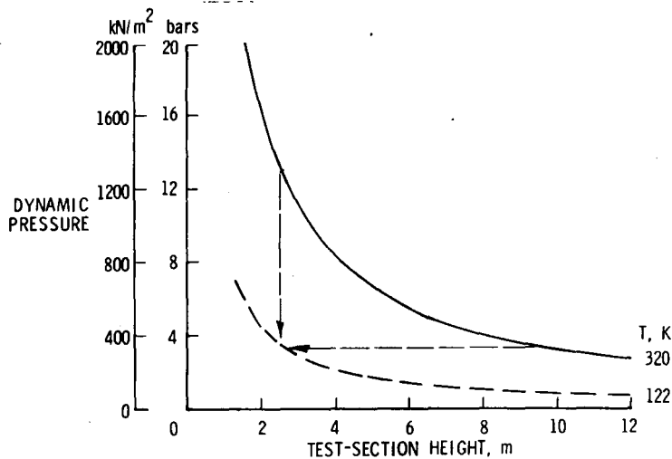
Figure 4.- Effect of cryogenic temperature on dynamic pressure and test-section size. R_{\bar{c}} = 120 \times 10^6 ; M = 1.0 ; \bar{c} = 0.1 test-section height.
