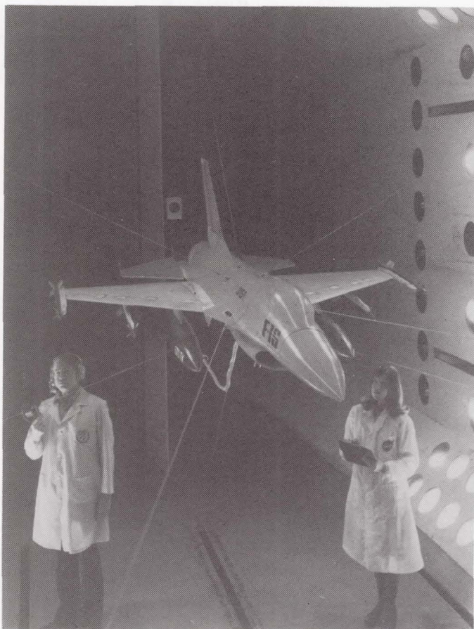
Figure 2.- Flutter model installed on cable support system in Langley 16-foot transonic dynamics tunnel.
