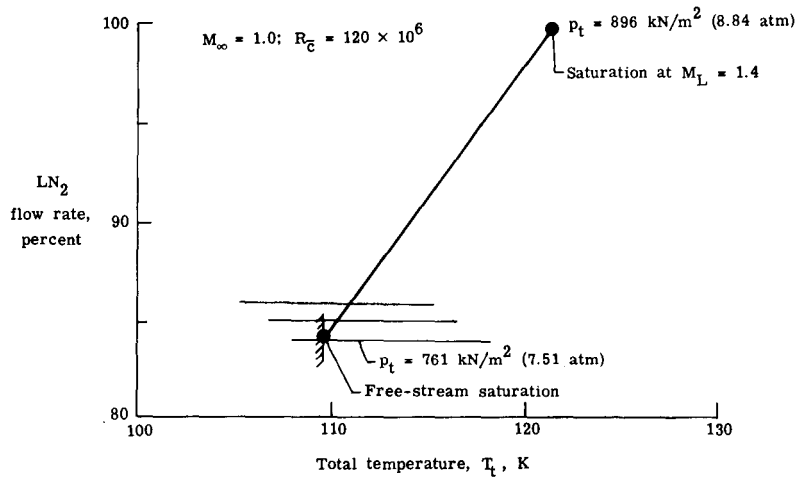
Figure 6.- LN 2 consumption as a function of temperature.
