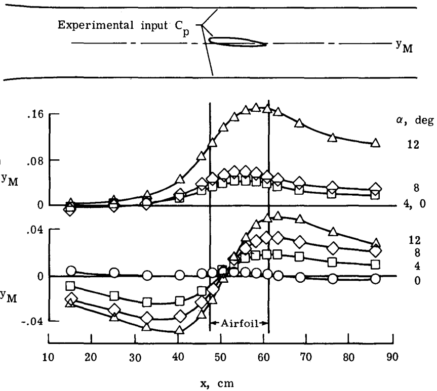
Figure 3.- Wall-induced velocities on tunnel axis. Straight tunnel walls.
