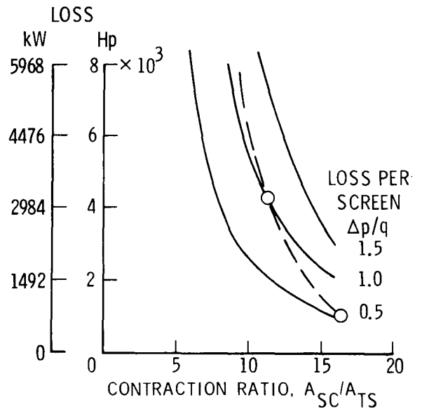
Figure 9.- Effect of contraction ratio on screen stress level and screen loss for three levels of screen pressure drop. Three screens; 0.76 mm wire diameter; p_t = 896 \text{ kN/m}^2 (8.96 bars); 0.61 m sag.
