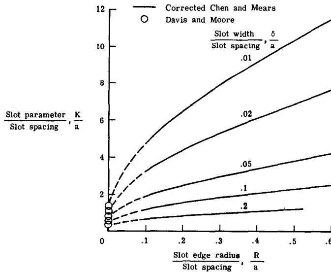
Figure 2.- Slot-parameter correlation.
