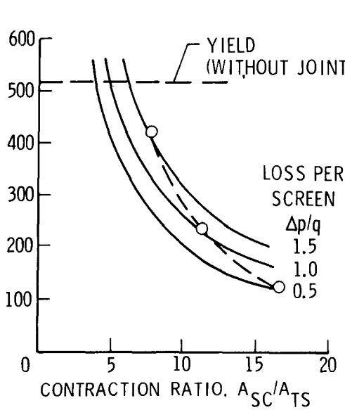
Figure 9.- Effect of contraction ratio on screen stress level and screen loss for three levels of screen pressure drop. Three screens; 0.76 mm wire diameter; p_t = 896 \text{ kN/m}^2 (8.96 bars); 0.61 m sag.
