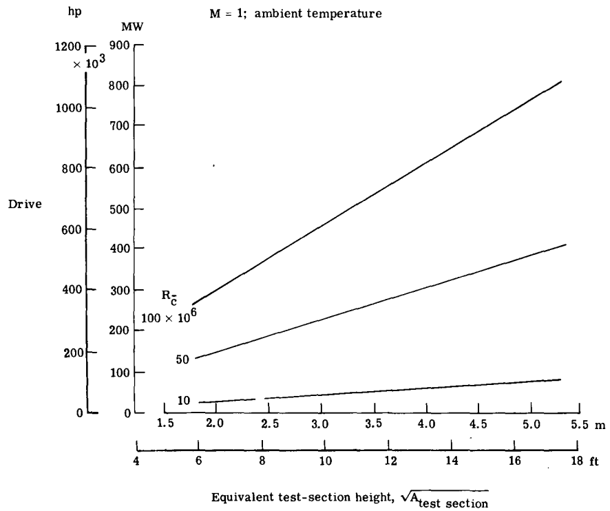
Figure 12.- Drive power requirements.
