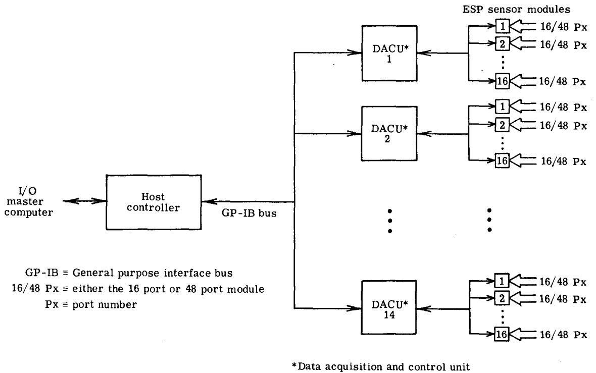
Figure 9.- Prototype electronic scanning pressure (ESP) measurement system.
