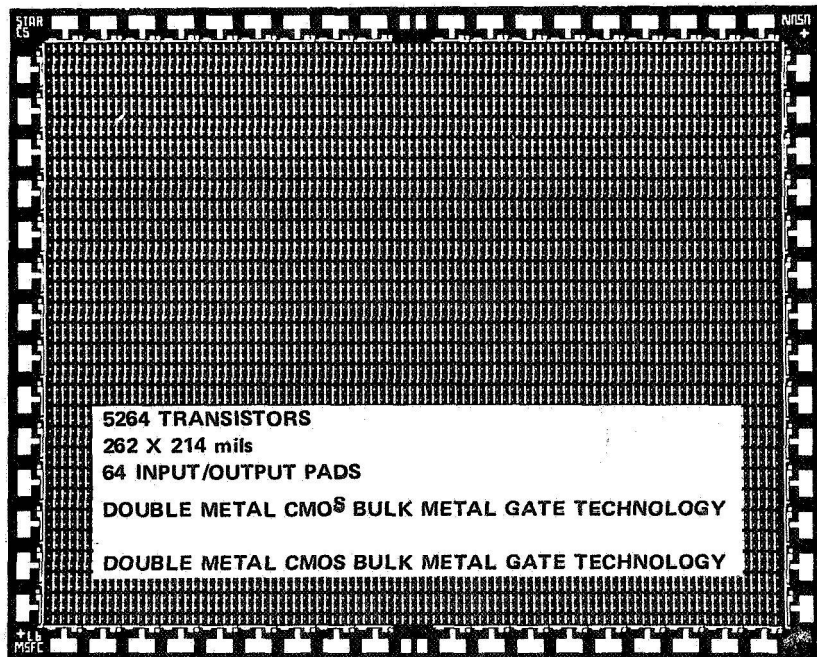
Figure 10. 5264 transistor STAR structure.
