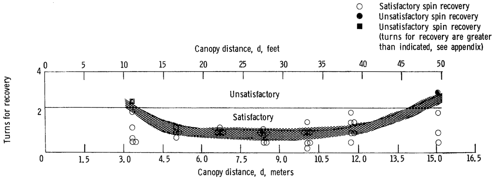
Figure 9.- Effect of canopy distance on turns for recovery from steep spin modes. Dimensions are full scale.
