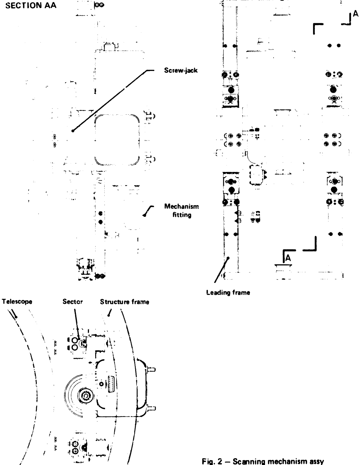
Fig. 2 - Scanning mechanism assy
