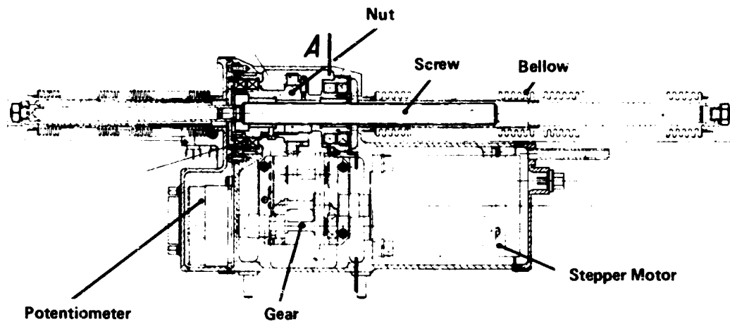
Fig. 3 - Screw-Jack unit
