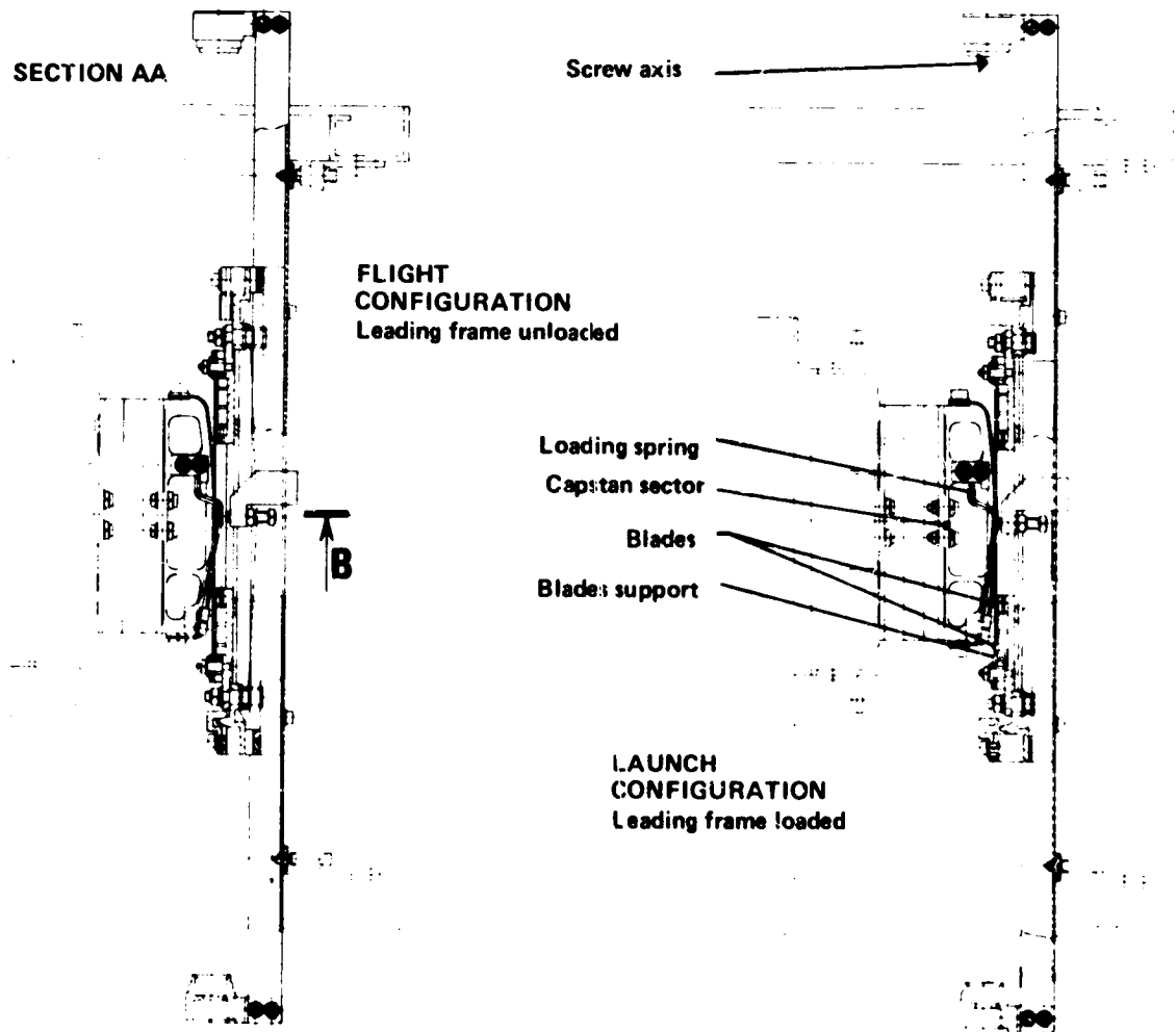
Fig. 4 - Leading frame assy
