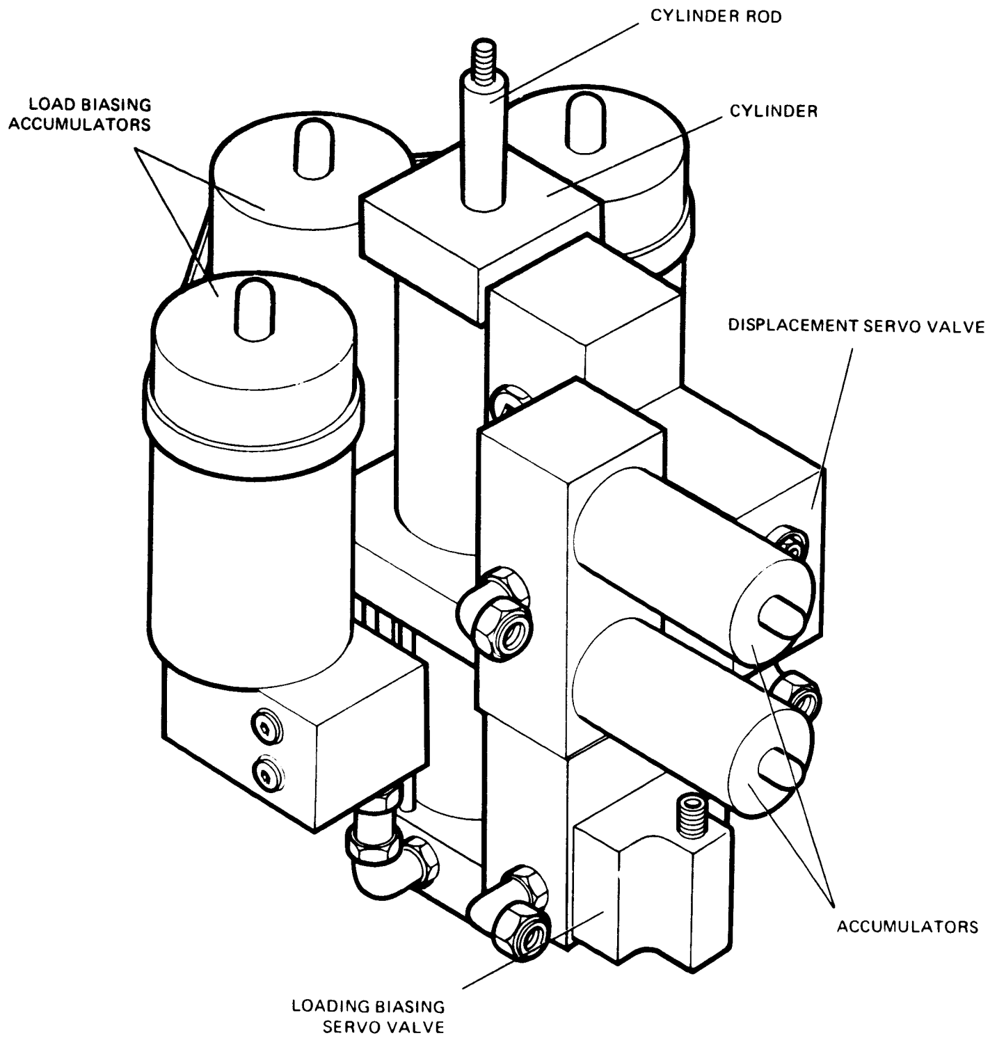
Figure 2 HYDRAULIC ACTUATOR
