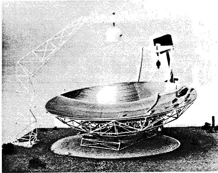
Fig. 7. Solar tracker assembly, stow position
