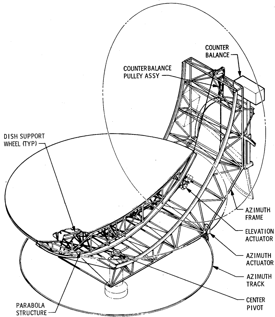
Fig. 4. Solar tracker assembly
