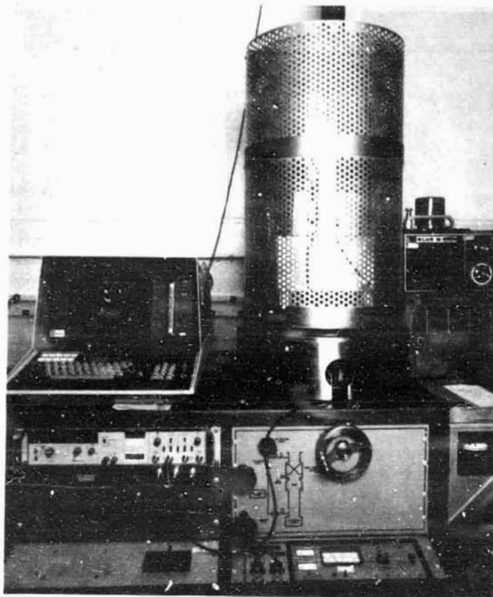
Fig. 3—Test System 3
