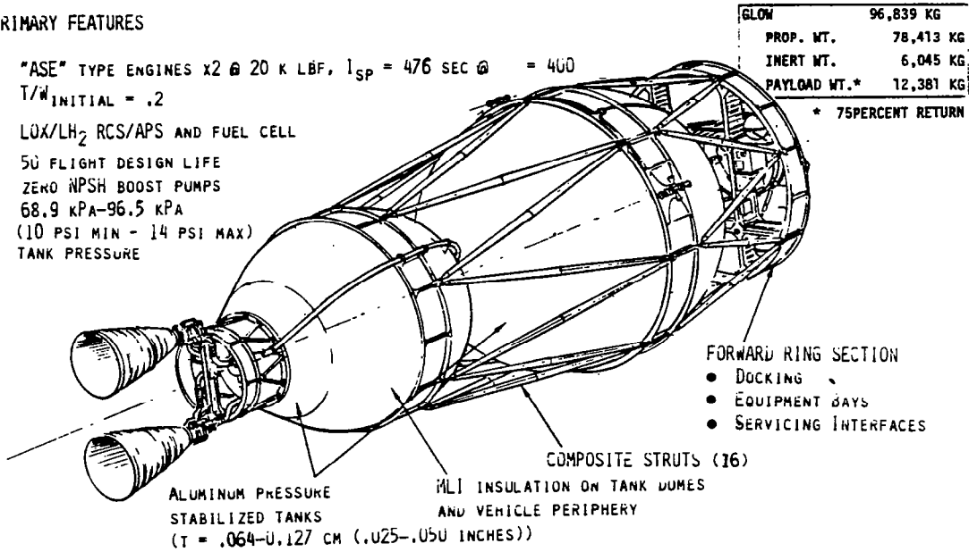
Figure 6.—POTV Design Concept
