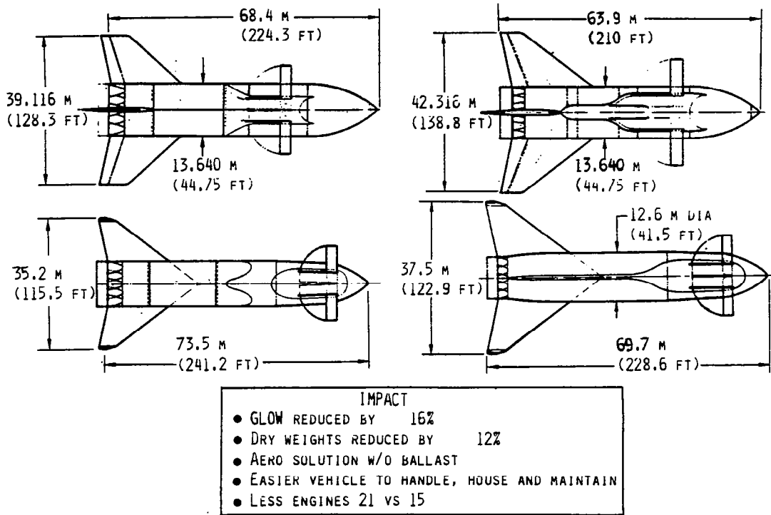
Figure 12.—Accelerated Technology Impact on HLLV
