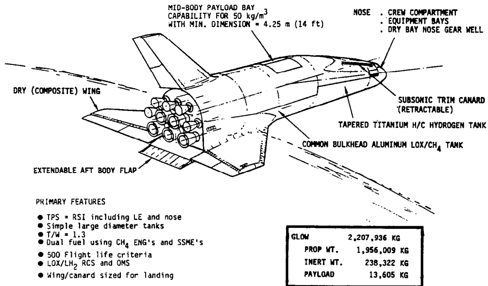
Figure 4.—SSTO Design Concept
