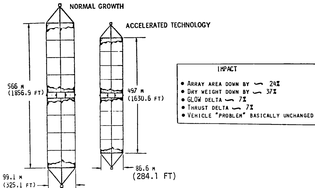
Figure 14.—Accelerated Technology Impact on LCOTV
