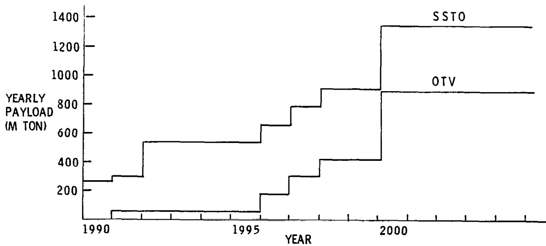
Figure 2.—Priority Payload Delivery Requirement
