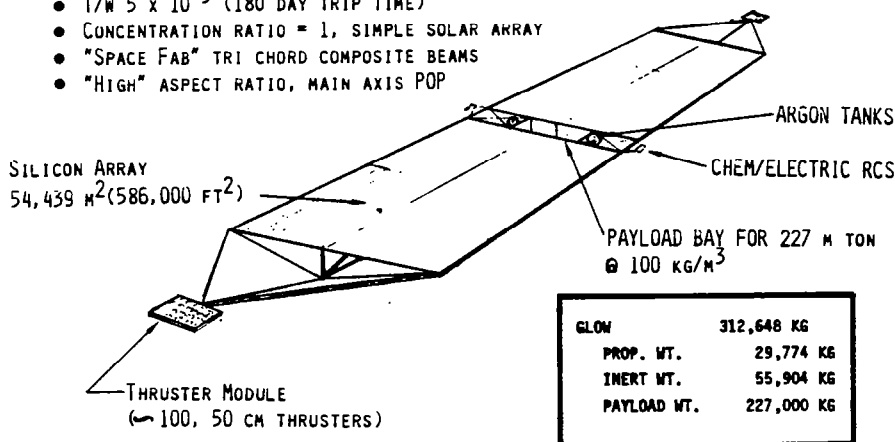
Figure 7.—LCOTV Design Concept
