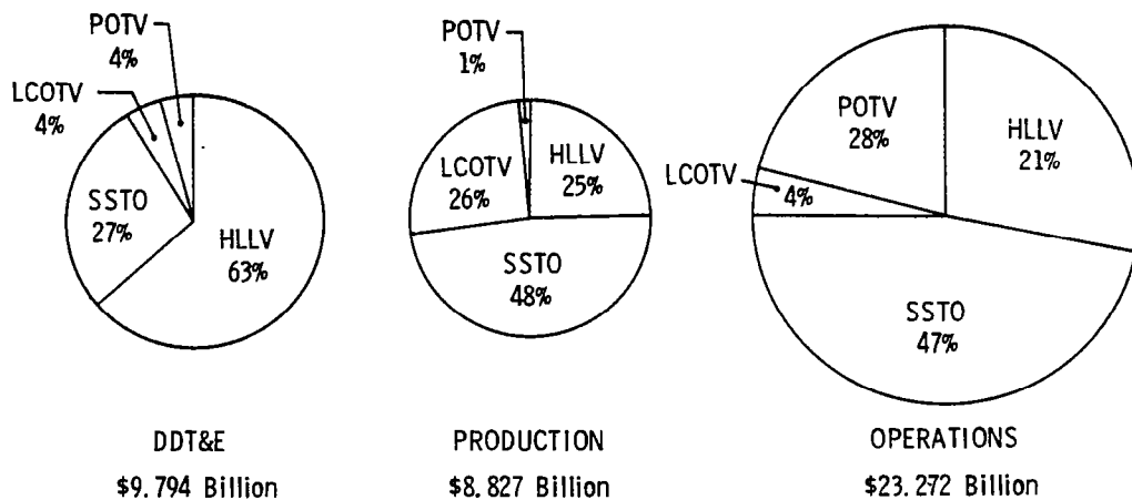
Figure 8. System Costs
