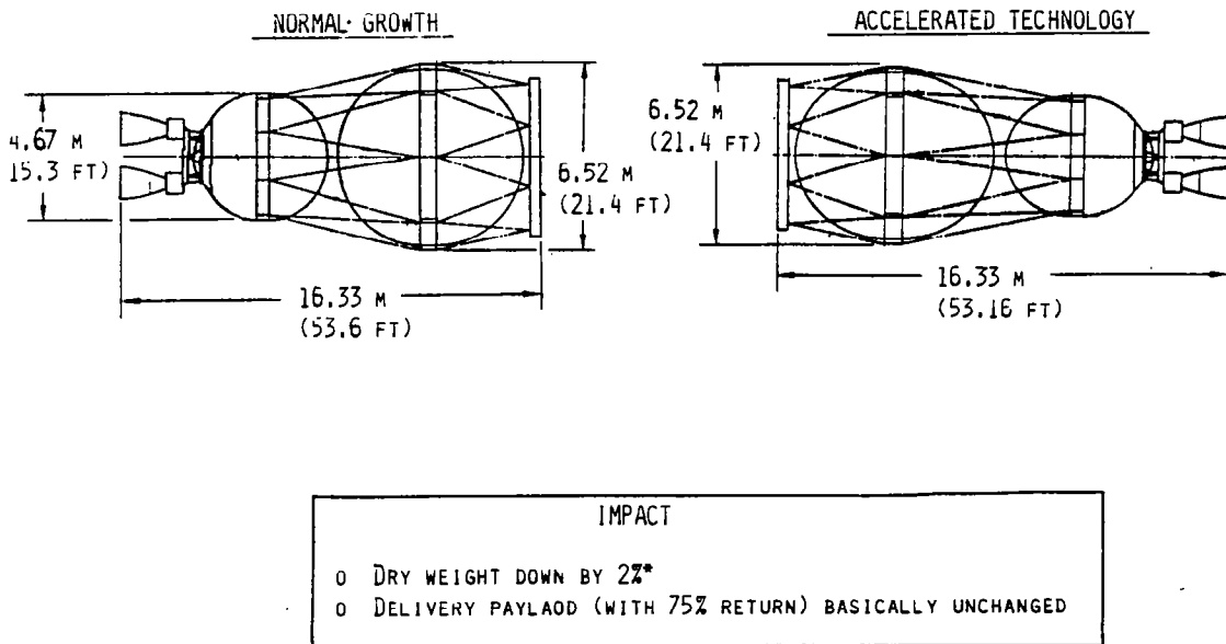
Figure 13.—Accelerated Technology Impact on POTV
