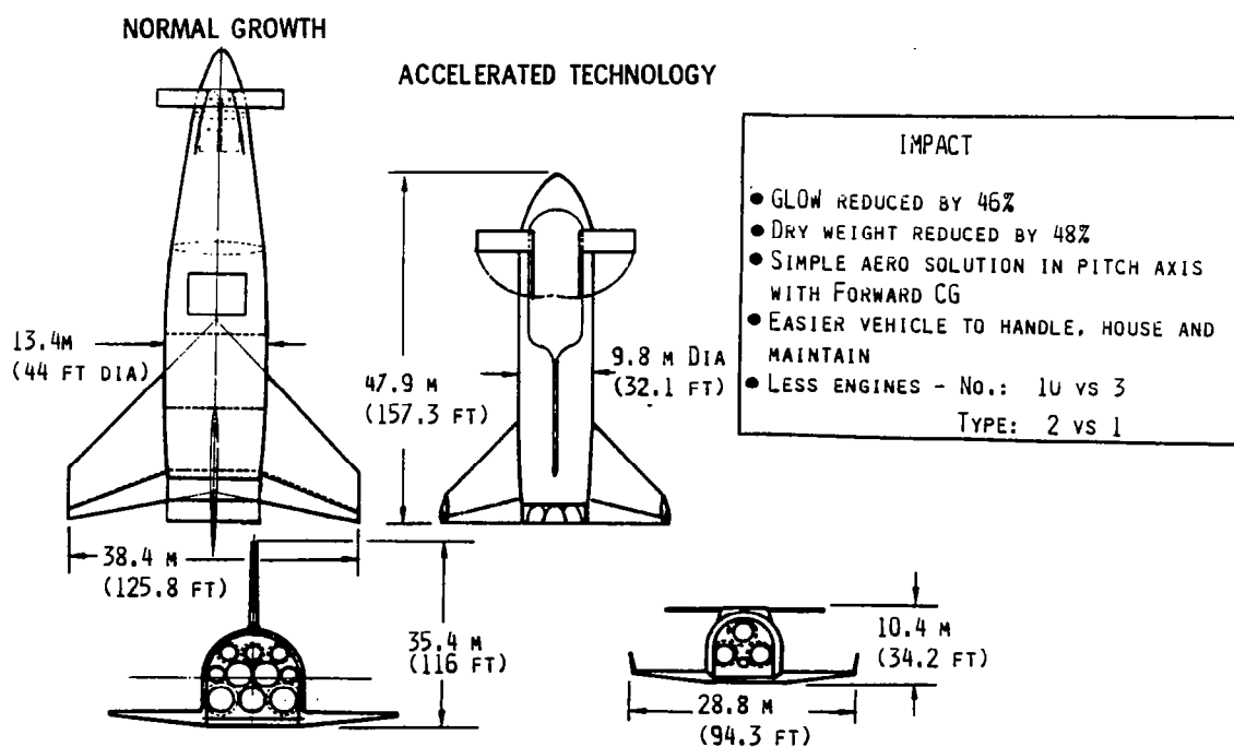
Figure 11.—Accelerated Technology Impact on SSTO
