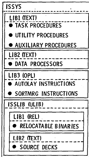
Figure 7.- ISSYS Library organization using CDC NOS utilities.
