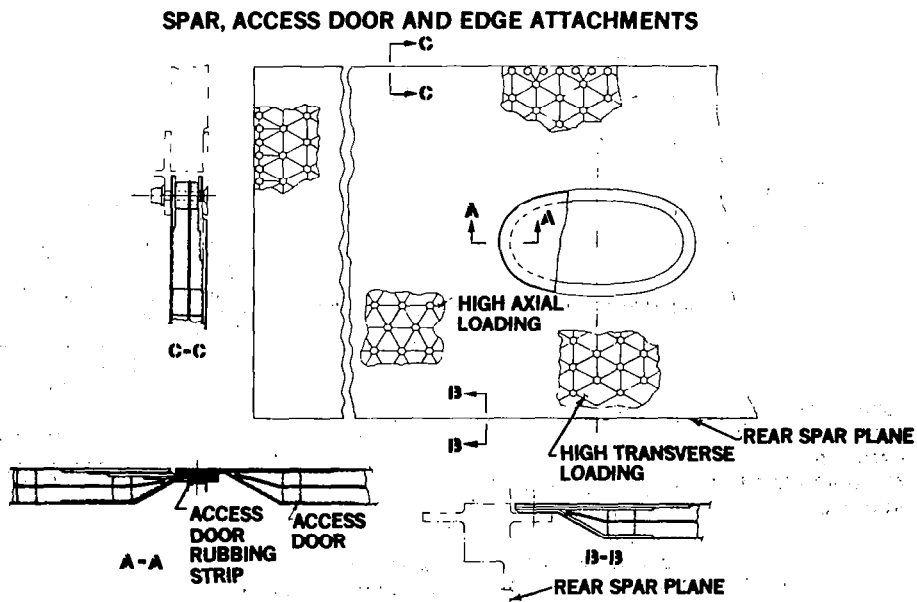
Figure 22.- SPF/DB isogrid panel design concept.
