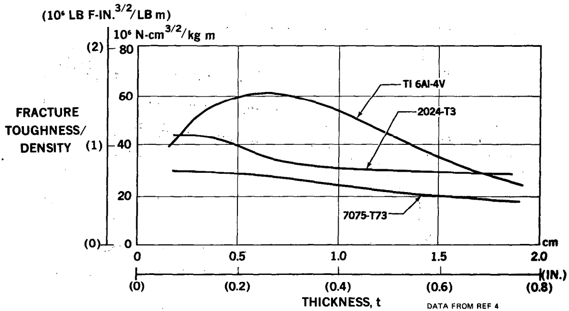
Figure 4.- Fracture toughness.
