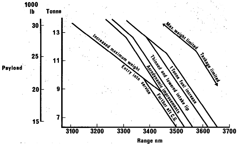
Figure 16.- Concorde payload/range characteristics.
