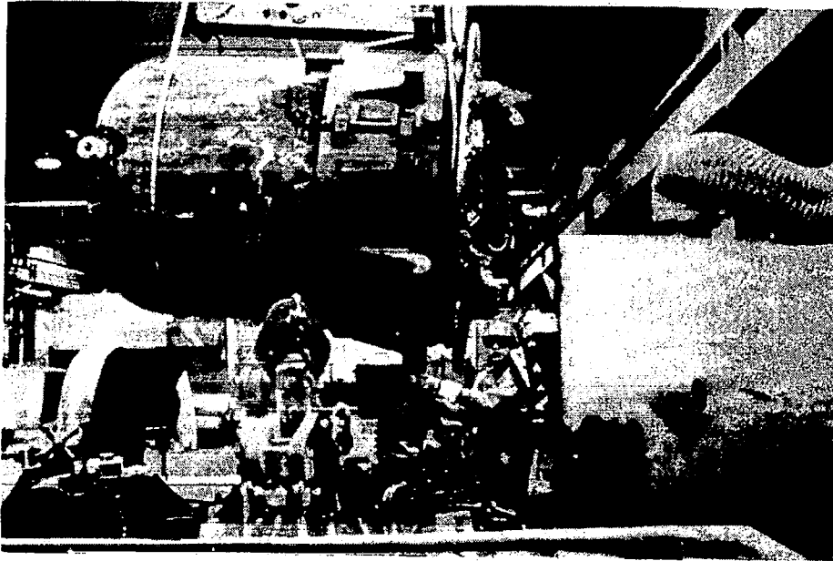
(d) Titanium sponge in reactor (after reduction of TiCl_4 with magnesium).
