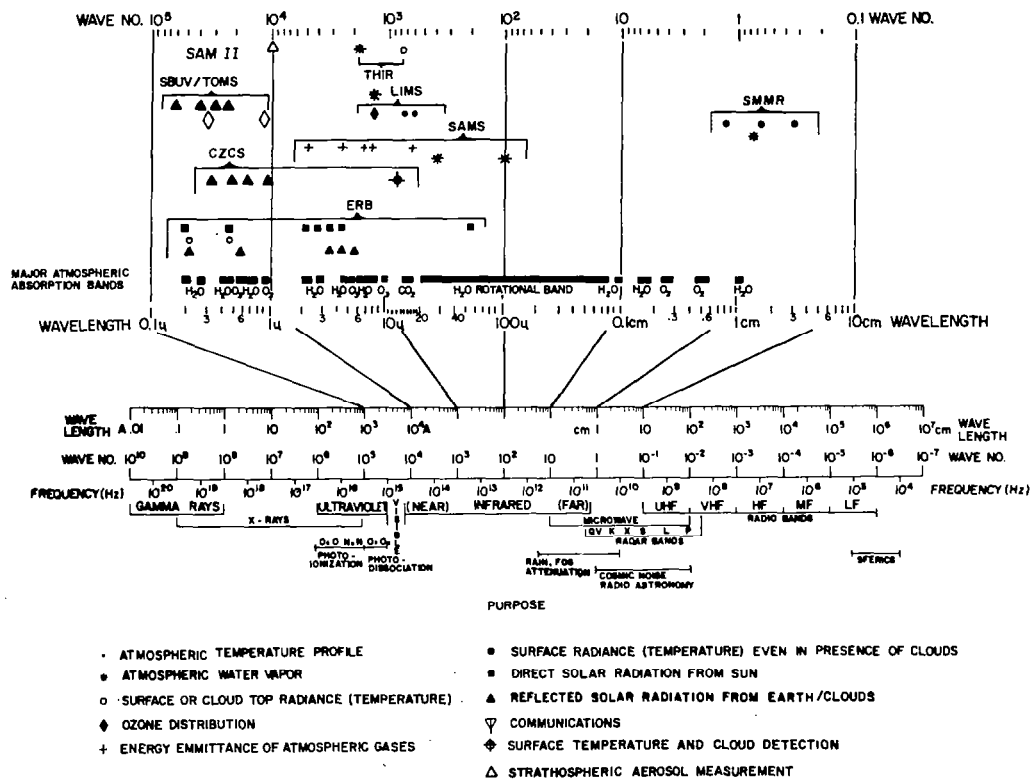
Figure 13. Relation of Nimbus 7 Experiments to the Electromagnetic Spectrum
