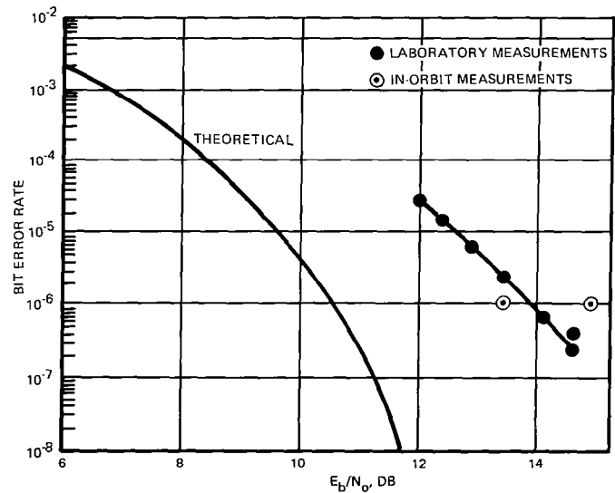
Figure 4. VAS Bit Error Rate Link Performance
