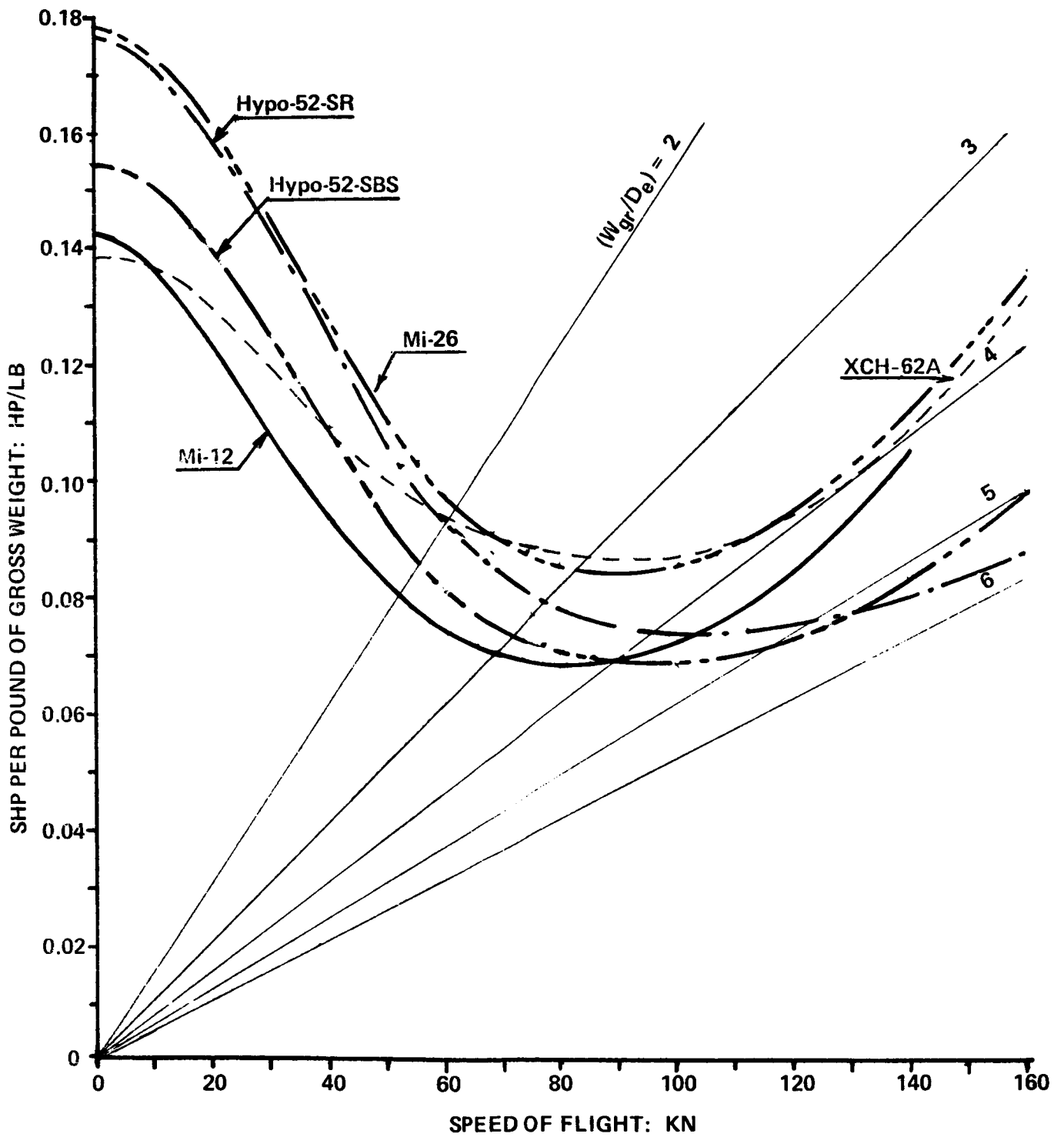
Figure 6.14 Comparison of shaft horsepower per pound of gross weight vs speed of level flight at SL/ISA of Soviet and Western helicopters of the over 100,000-lb gross weight class.
