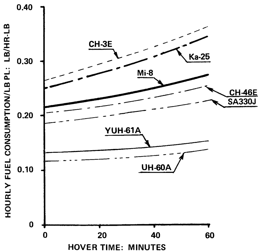
Figure 4.16 Variation with time of hourly fuel consumption per pound of maximum payload in hover OGE, SL, ISA for Soviet and Western helicopters of the 12,000 to 30,000-lb gross weight class.
