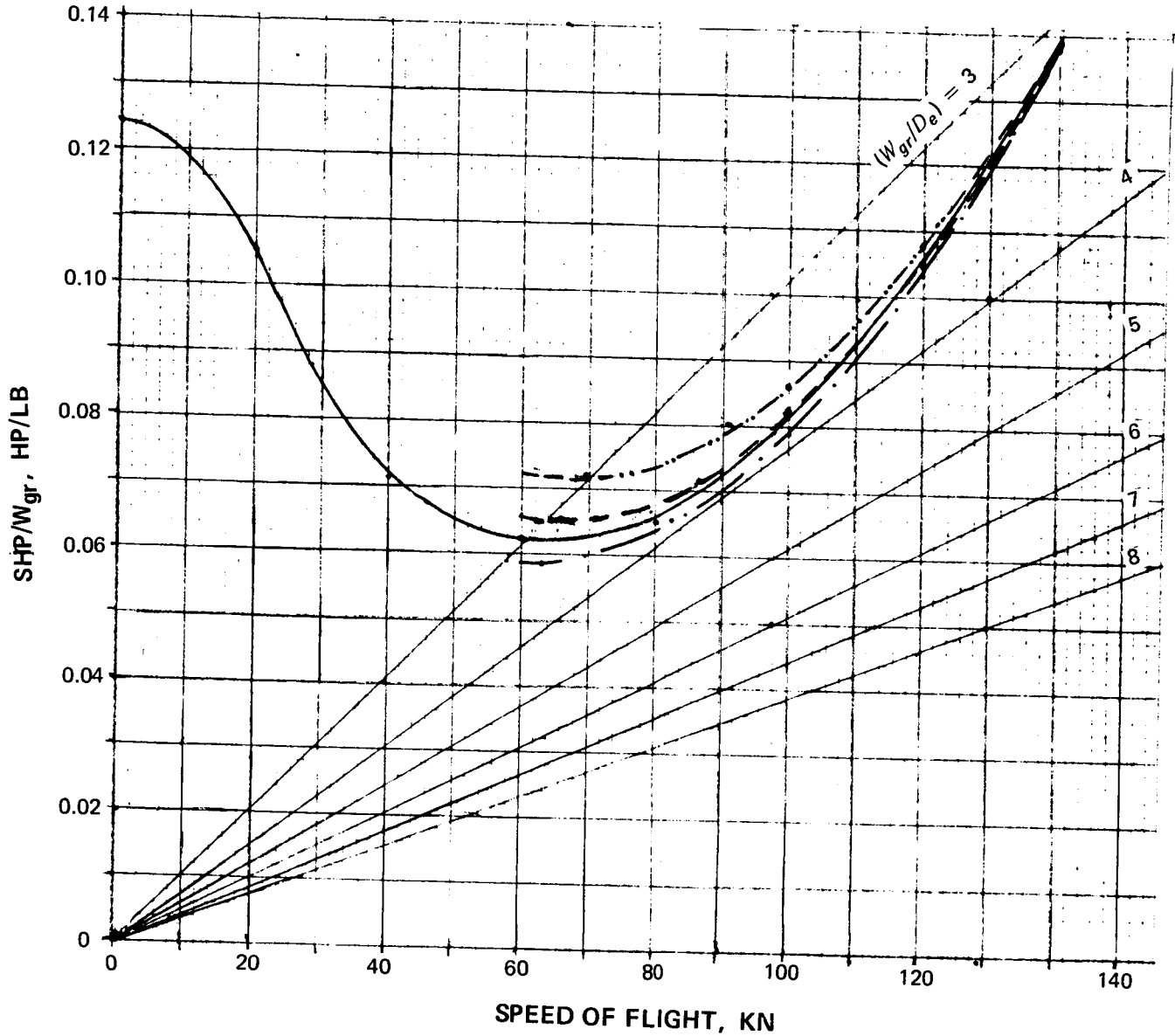
Figure 1.6 Example of approximating a given (SHP/W_{gr}) = f(V) curve through the single-point approach and various assumed values of \eta_{oa} ; k_{ind} and \bar{c}_d/\bar{c}_l
