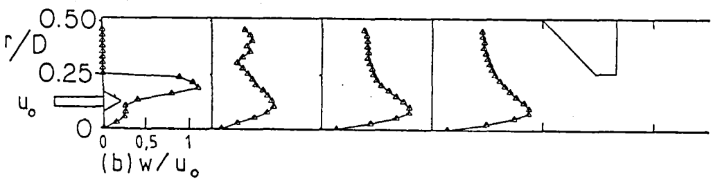
(b) L/D = 2.0
