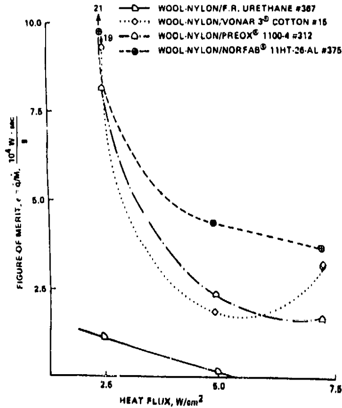
Figure 3: THERMAL EFFICIENCY COMPARISON OF HEAT BLOCKING LAYERS FOR NF URETHANE AS A FUNCTION OF HEAT FLUX AT 2 MINUTES ELAPSED TIME
