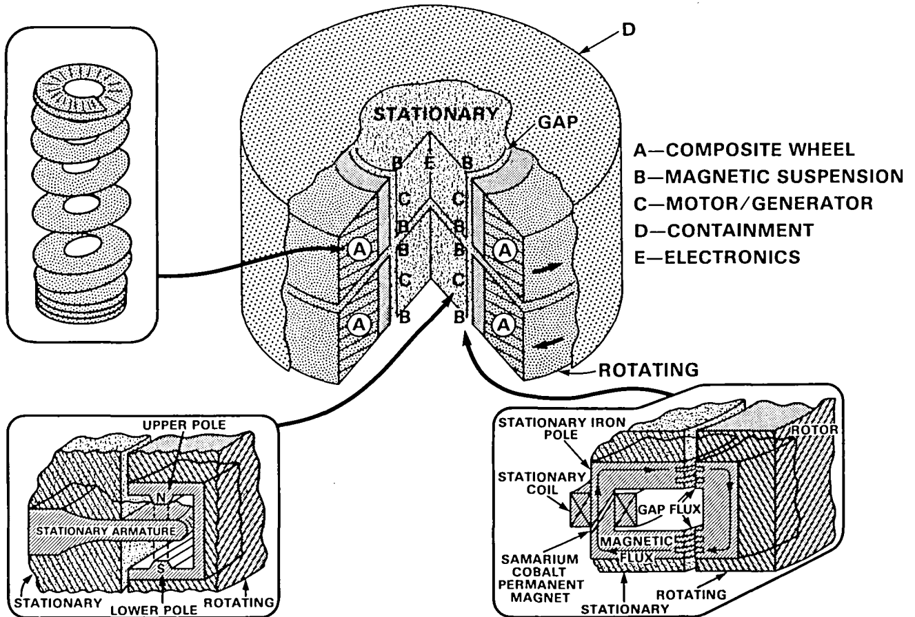
Figure 1.- Spacecraft flywheel power system: conceptual flywheel design.
