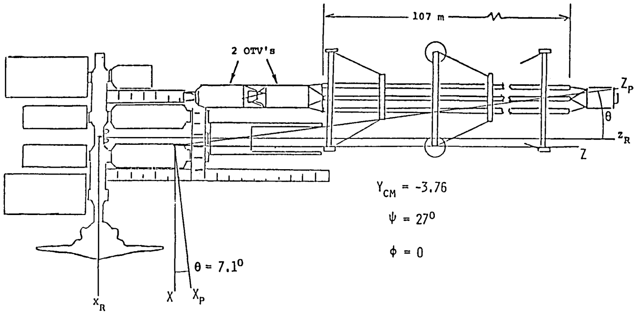
BOEING PHASE "A" STUDY CONFIGURATION III (GIANT)
