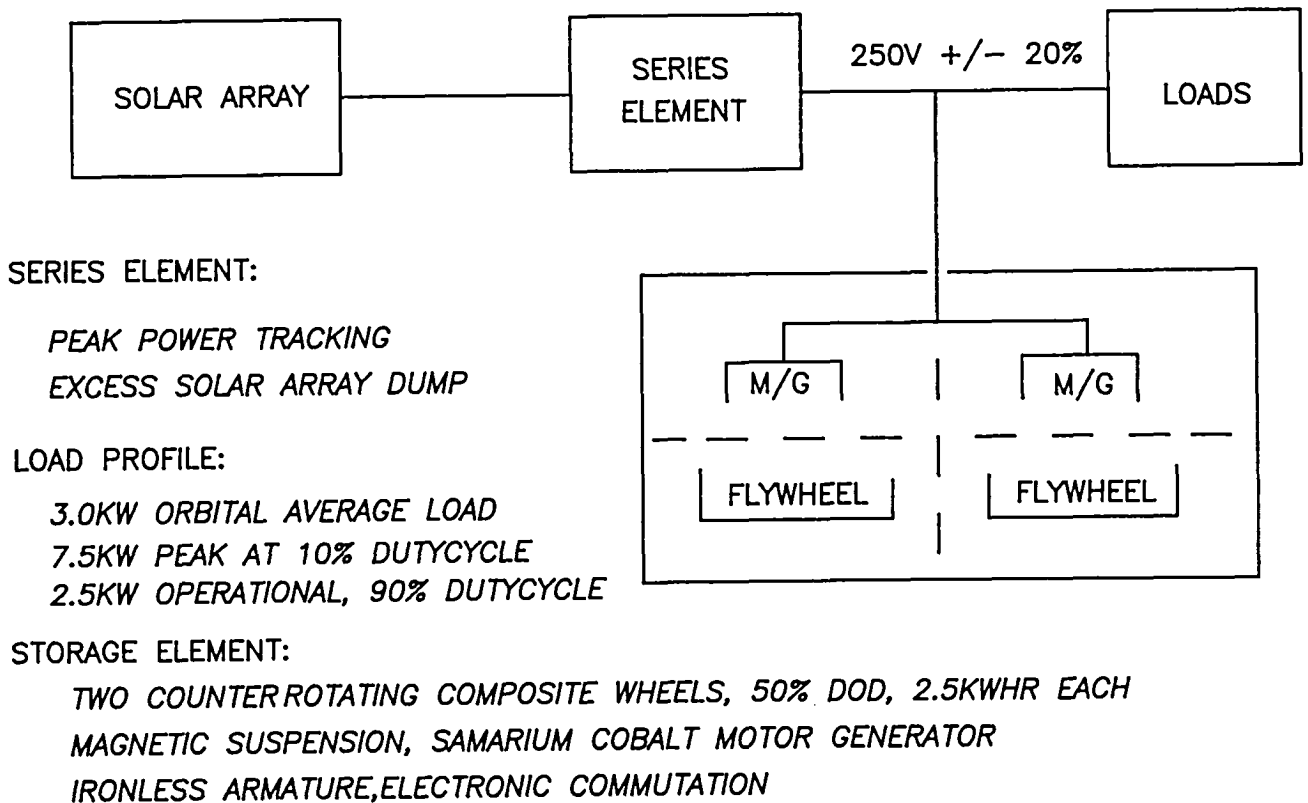
Figure 3.- Spacecraft flywheel power system: baseline definition.
