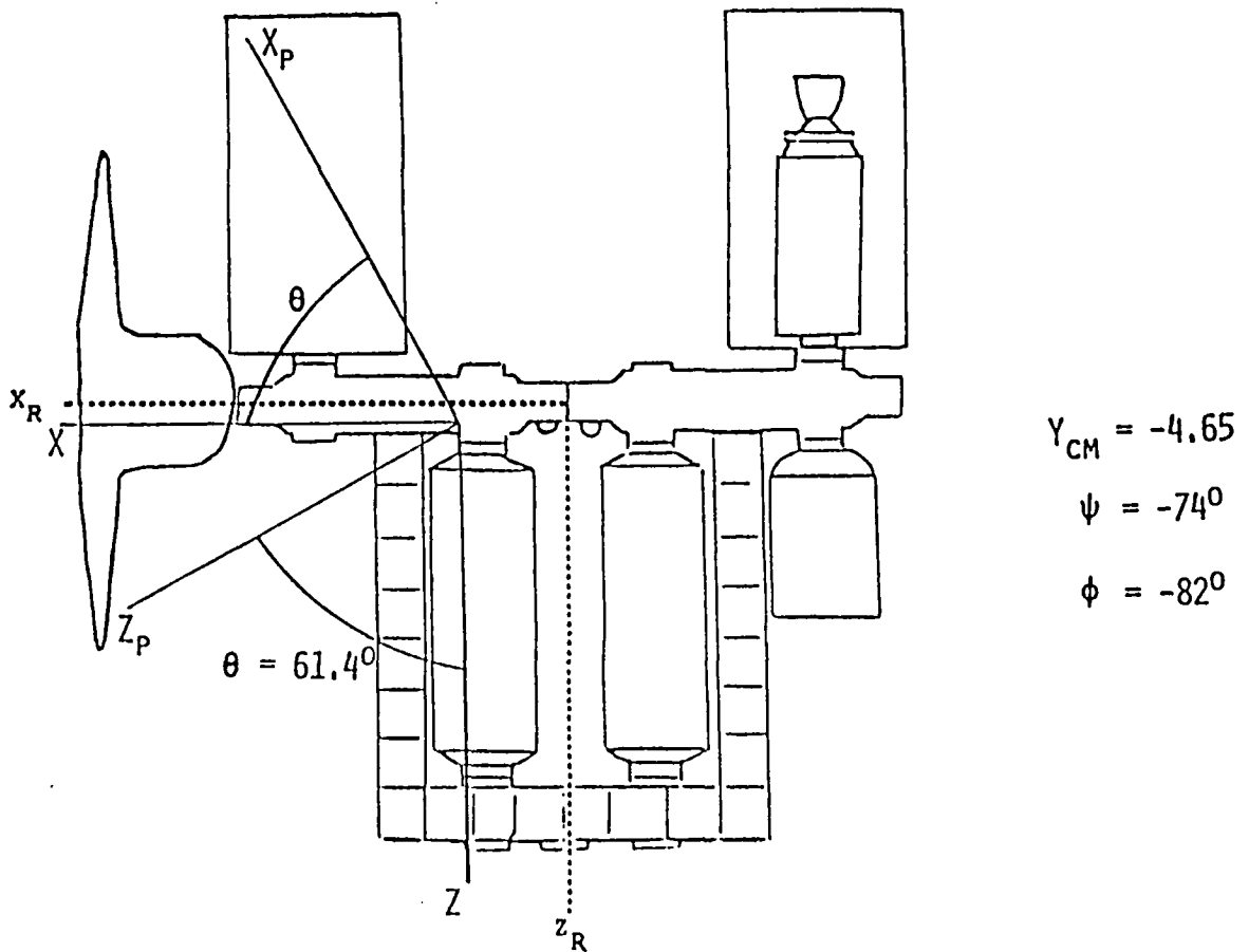
BOEING PHASE "A" STUDY CONFIGURATION II
