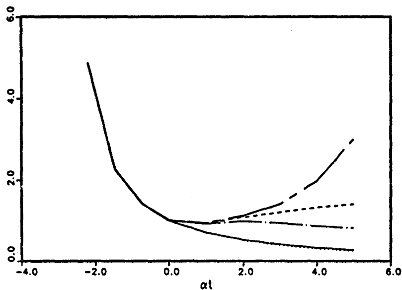
Fig. 9.7a. Time history of the dissipation rate of turbulence, nondimensionalized by the dissipation rate at \alpha t = 0 , of the turbulent flows shown in Fig. 9.1a.
