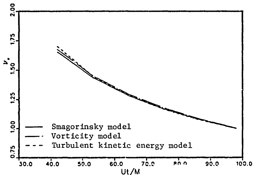
Fig. 6.7a. Decay of the spatially averaged eddy viscosity in homogeneous isotropic turbulence. Large eddy simulation as described in caption of Fig. 4.1; Smagorinsky model constant c_s = 0.21 ; vorticity model constant, c_v = 0.21 ; TKE model constant, c_q = 0.16 .
