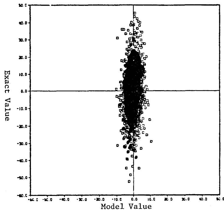
Fig. 6.1b. Smagorinsky model. "Exact" vs. model values of the divergence of the subgrid-scale Reynolds stress \partial\tau_{1j}/\partial x_j in homogeneous isotropic turbulence. R_\lambda = 38 and R_{SGS} = 180 .
