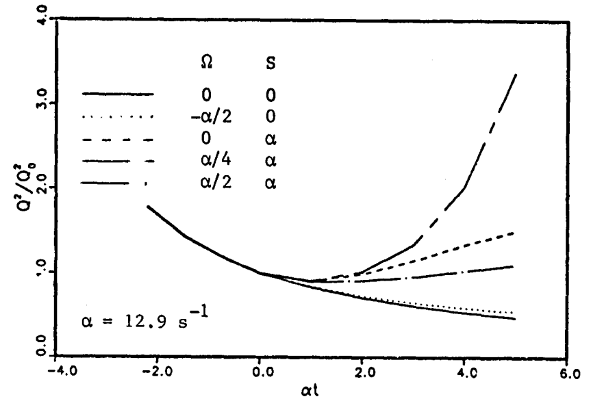
Fig. 9.1b. Time history of the turbulence intensity of homogeneous shear turbulent flows in the presence of system rotation. Large eddy simulation, pseudo-spectral method, Smagorinsky and scale similarity model, c_s = 0.16 and c_r = 1.1 .
