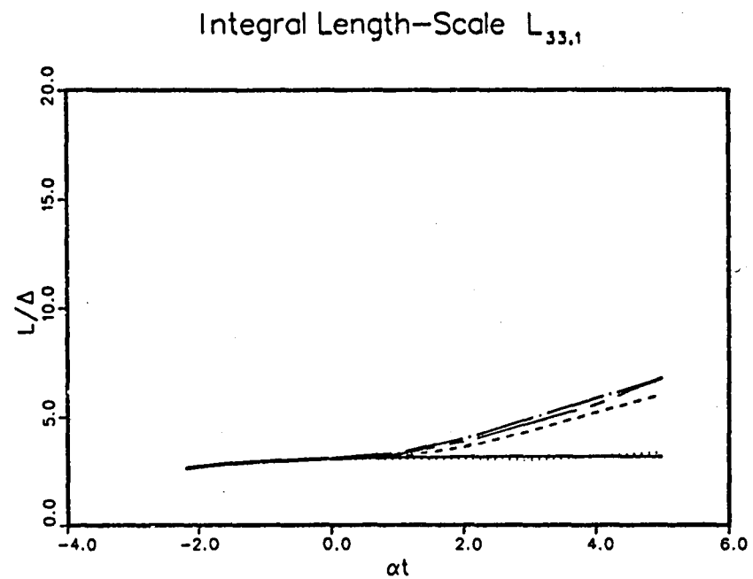
Fig. 9.21b. Time history of the integral length scale, L_{33,1} , of the turbulent flows shown in Fig. 9.1b.
