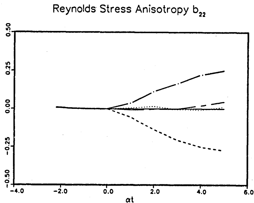
Fig. 9.4a. Time history of the component b_{22} of the Reynolds stress anisotropy tensor of the turbulent flows shown in Fig. 9.1a.
