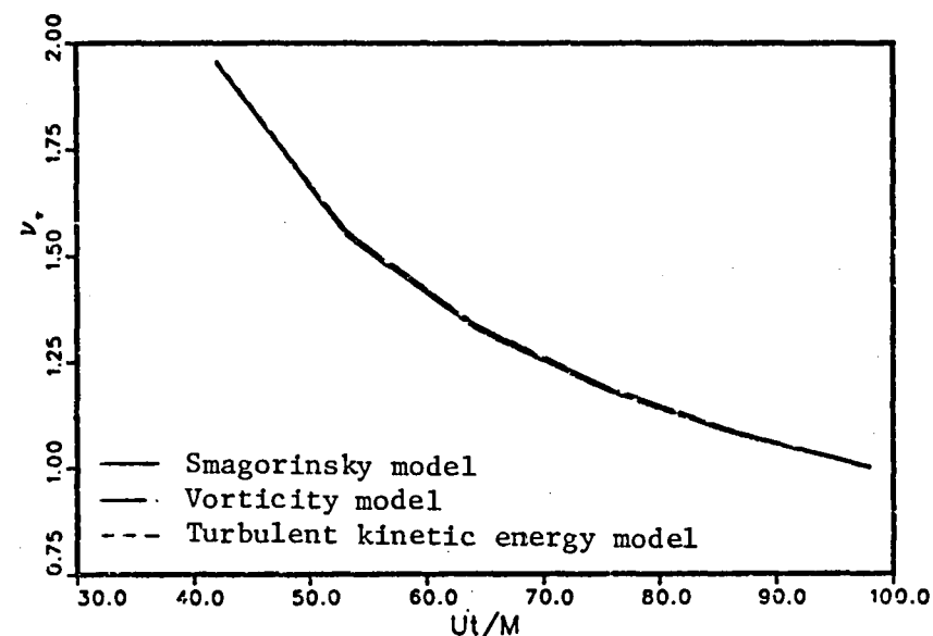
Fig. 6.7b. Decay of the spatially averaged eddy viscosity in homogeneous isotropic turbulence (see caption of Fig. 4.1). Large eddy simulation with pseudospectral method. Smagorinsky model constant, c_s = 0.19 ; vorticity model constant, c_v = 0.19 ; TKE model constant, c_q = 0.145 .
