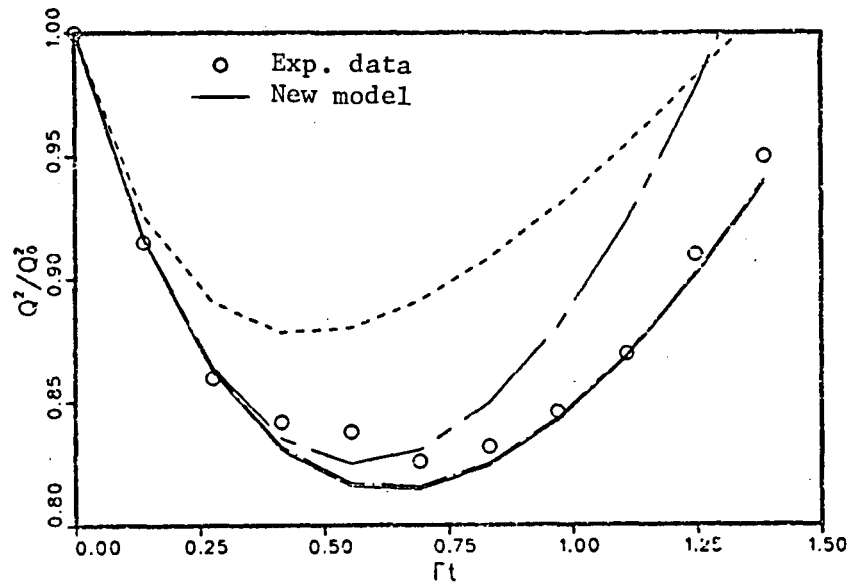
Fig. 8.8a. Time-averaged Reynolds stress model prediction of the turbulence intensity of the experimental results of Gence and Matheiu (1979) on homogeneous turbulence subject to a mean axisymmetric strain rate; \Gamma = 32.23 \text{ s}^{-1} . See Fig. 8.7 for symbols.
