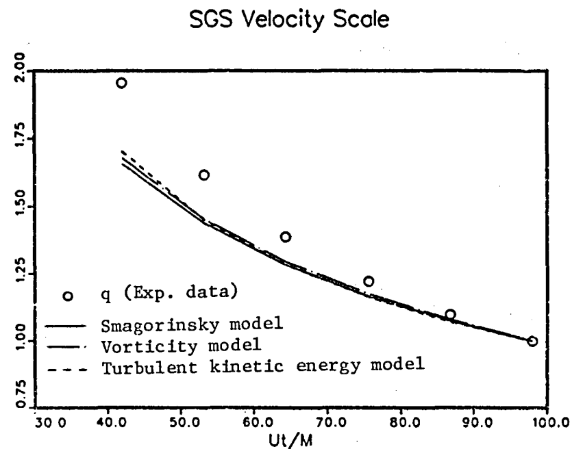
Fig. 4.4. Comparison of the time history of the r.m.s. of the subgrid-velocity scale q and eddy viscosity . Both variables are nondimensionalized with their respective values at U_t/M = 98 .
