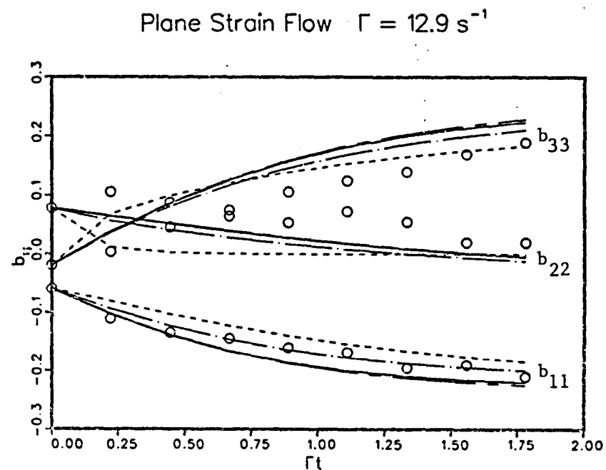
Fig. 8.7b. Time-averaged Reynolds stress model prediction of the components of the Reynolds stress anisotropy tensor of the flow of Fig. 8.7a; the lines are as in the previous figure.
