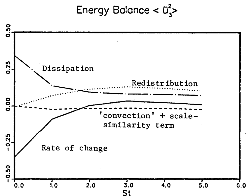
Fig. 8.6b. Time history of each spatially averaged term of the \langle \bar{u}_j^2 \rangle equation of the filtered flow field shown in Fig. 8.1b.
