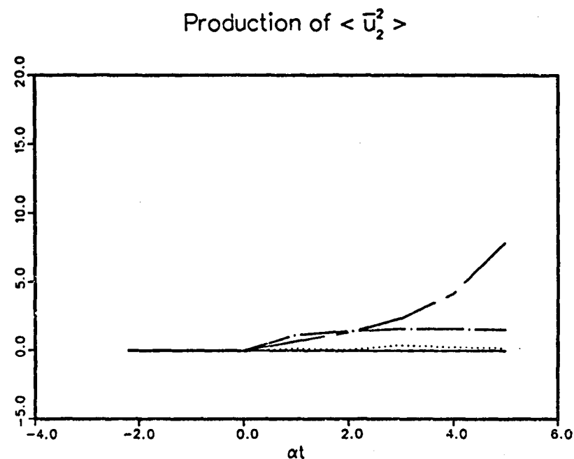
Fig. 9.9b. Time history of the component P_{22} of the production rate of turbulence, nondimensionalized by the dissipation rate at \alpha t = 0 , of the turbulent flows shown in Fig. 9.1b.
