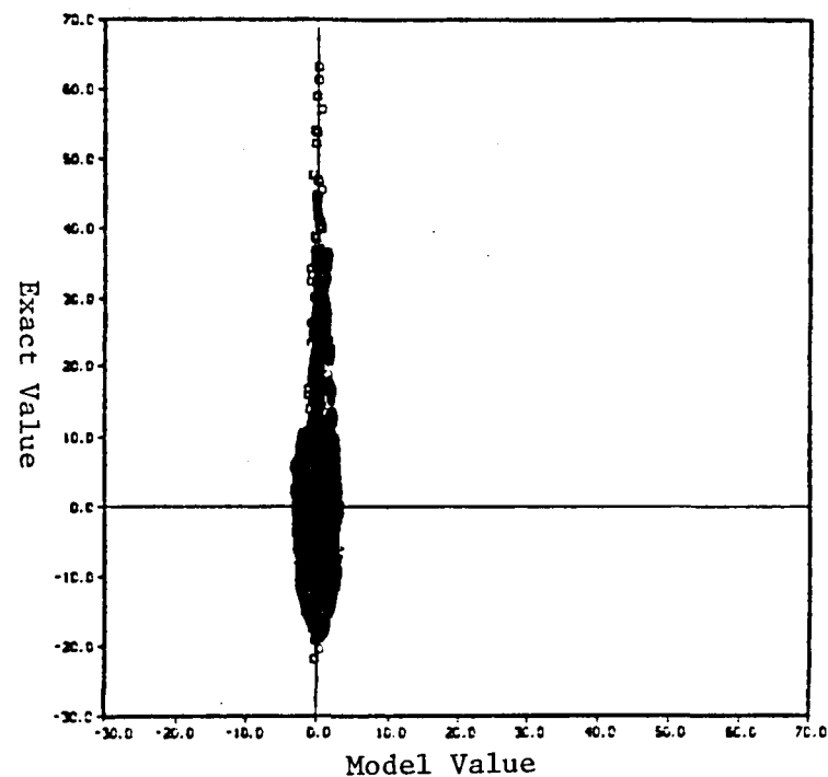
Fig. 6.2a. Smagorinsky model. "Exact" vs. model values of the subgrid-scale Reynolds stress \tau_{12} in homogeneous sheared turbulence. S = 34 and R_{SGS} = 204 .
