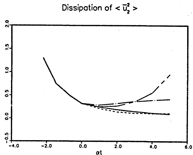
Fig. 9.11b. Time history of the component \varepsilon_{22} of the dissipation rate of turbulence, nondimensionalized by the dissipation rate at \alpha t = 0 , of the turbulent flows shown in Fig. 9.1b.
