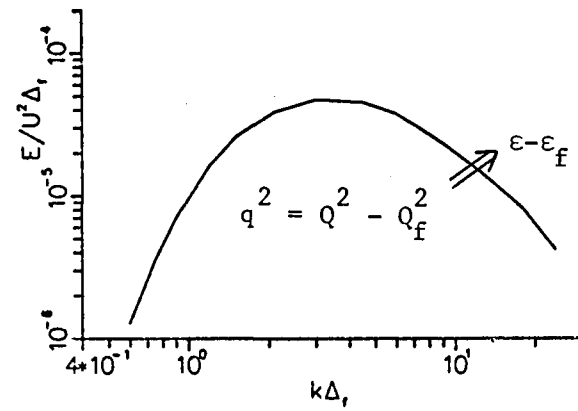
3-D SGS Energy Spectrum
