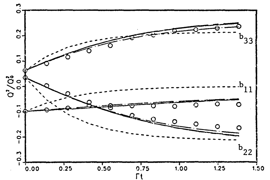
Fig. 8.8b. Time-averaged Reynolds stress model prediction of the components of the Reynolds stress anisotropy tensor of the flow of Fig. 8.8a.
