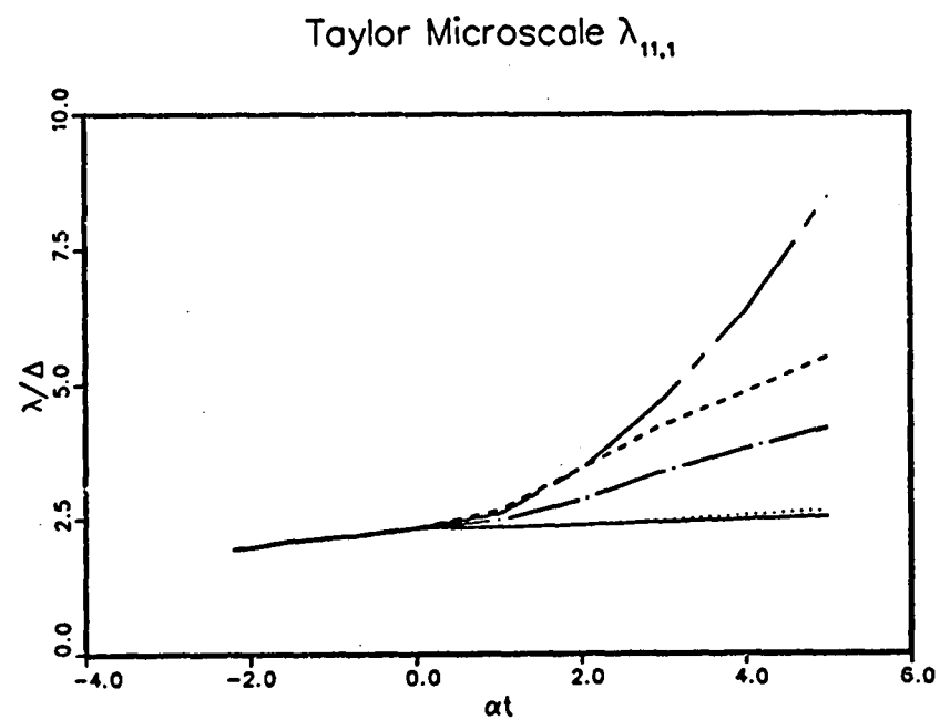
Fig. 9.16b. Time history of the Taylor microscale \lambda_{11,1} , of the turbulent flows shown in Fig. 9.1b.
