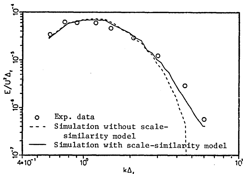
Fig. 6.10. Three-dimensional energy spectrum of the filtered flow field in homogeneous isotropic turbulence at U_t/M = 98 of Fig. 6.9.
