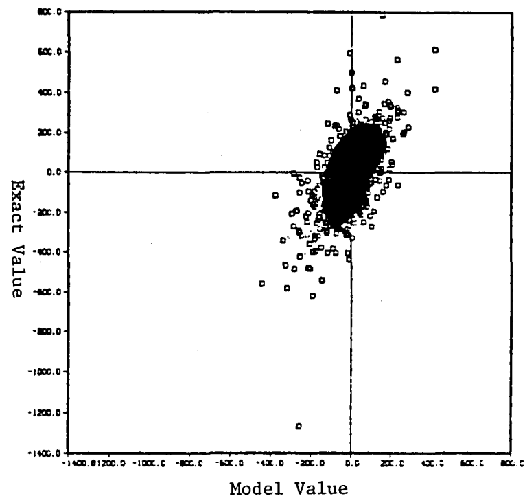
Fig. 6.6c. Scale similarity and Smagorinsky model. "Exact" vs. model values of the dissipation due to the subgrid-scale Reynolds stress \bar{u}_i \partial \tau_{ij} / \partial x_j in homogeneous sheared tur- bulence. S = 34 and R_{SGS} = 204 .
