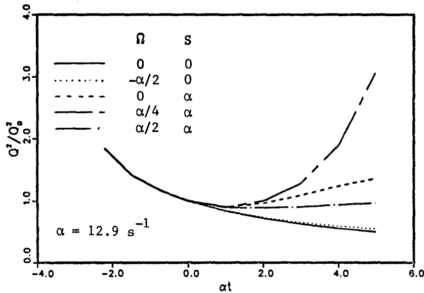
Fig. 9.1a. Time history of the turbulence intensity of homogeneous shear turbulent flows in the presence of system rotation. Large eddy simulation, pseudo-spectral method, Smagorinsky model, c_s = 0.19 .
