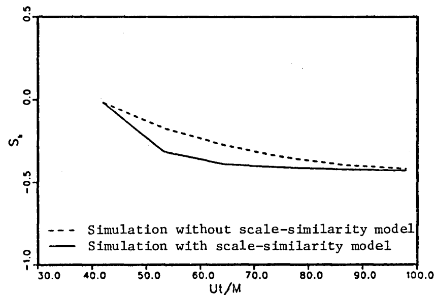
Fig. 6.11. Time history of the velocity-derivative skewness of the filtered flow field in the homogeneous isotropic turbulence flow of Fig. 6.9.
