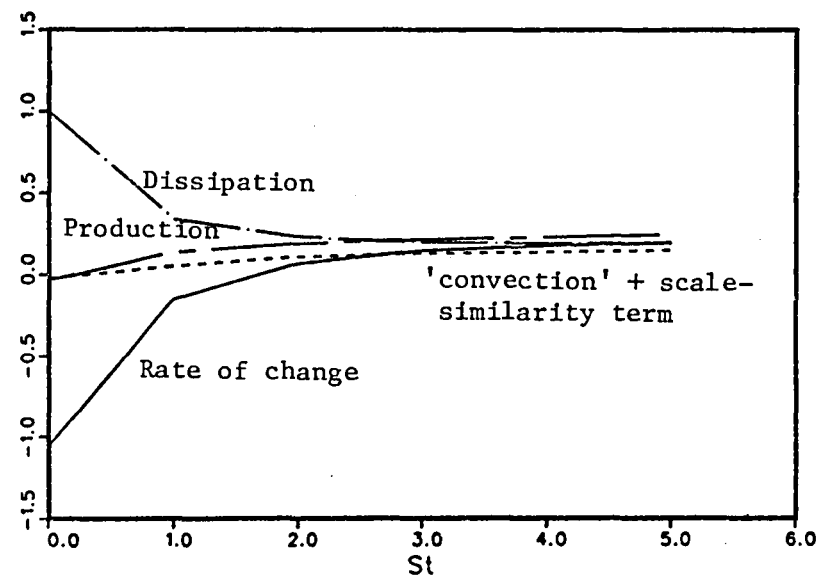
Fig. 8.3b. Time history of each spatially averaged term of the turbulent kinetic energy equation of the filtered flow field shown in Fig. 8.1b.
