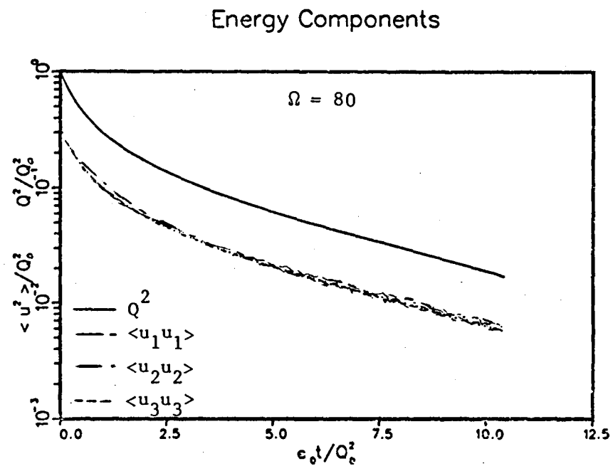
Fig. 7.5. Time history of the components of the turbulence intensity in the \Omega = 80 \text{ s}^{-1} case of Fig. 7.4.
