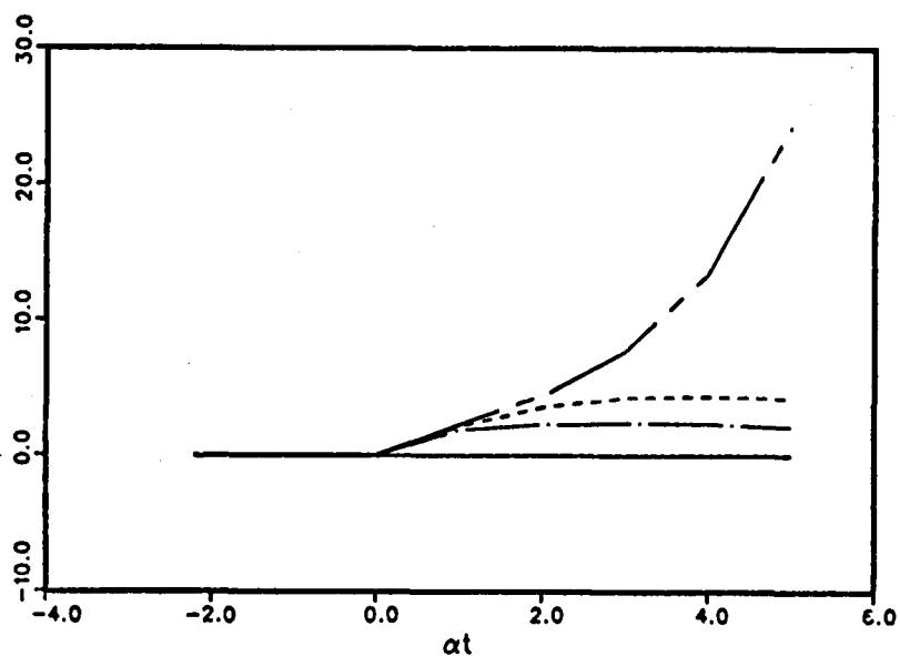
Fig. 9.6a. Time history of the production rate of turbulence, nondimensionalized by the dissipation rate at \alpha t = 0 , of the turbulent flows shown in Fig. 9.1a.
