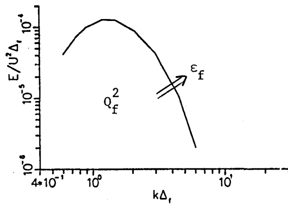
3-D Filtered Energy Spectrum
