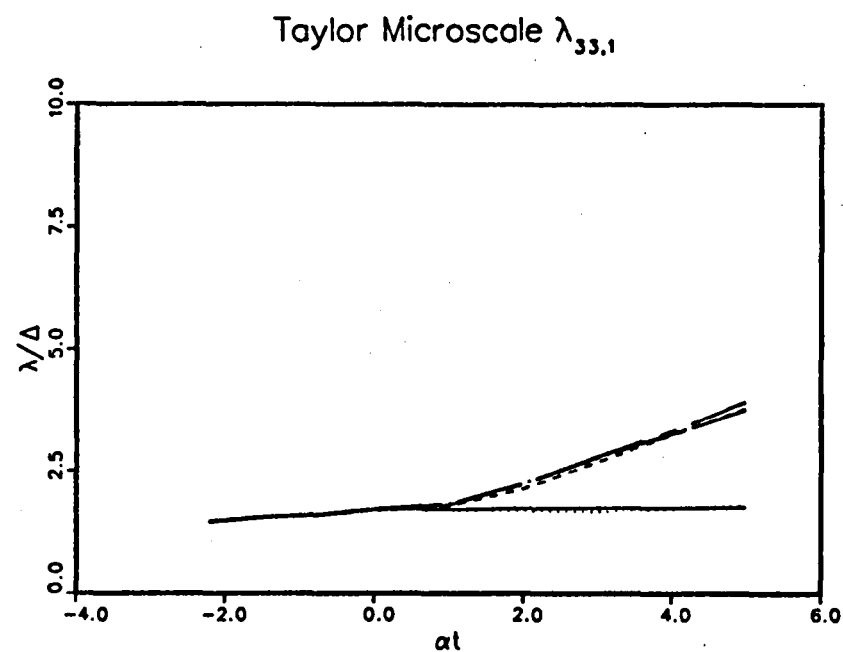
Fig. 9.18b. Time history of the Taylor microscale, \lambda_{33,1} , of the turbulent flows shown in Fig. 9.1b.
