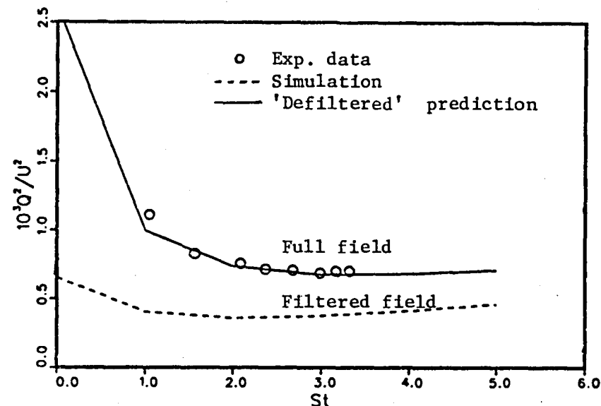
Fig. 8.1b. Time history of full and filtered turbulence intensities of homogeneous shear turbulent flow with U = 12.4 m/s and S = 12.9 \text{ s}^{-1} . Comparison of experimental results of Champagne, Harris, and Corrsin (1970) and large eddy simulation with pseudospectral method and Smagorinsky and scale similarity models, c_s = 0.19 and c_r = 1.1 .
