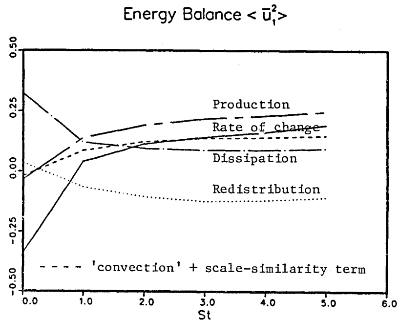
Fig. 8.4b. Time history of each spatially averaged term of the \langle \bar{u}_1^2 \rangle equation of the filtered flow field shown in Fig. 8.1b.
