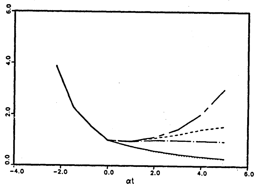
Fig. 9.7b. Time history of the dissipation rate of turbulence, nondimensionalized by the dissipation rate at \alpha t = 0 , of the turbulent flows shown in Fig. 9.1b.
