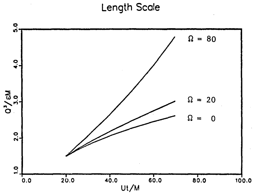
Fig. 7.3. Growth of the average length scale in the homogeneous rotating flows of Fig. 7.2.
