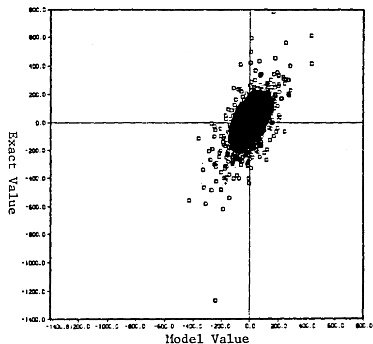
Fig. 6.4c. Scale similarity model. "Exact" vs. model values of the dissipation due to the subgrid-scale Reynolds stress \overline{u_i} \partial \tau_{ij} / \partial x_j in homogeneous sheared turbulence. S = 34 and R_{SGS} = 204 .
