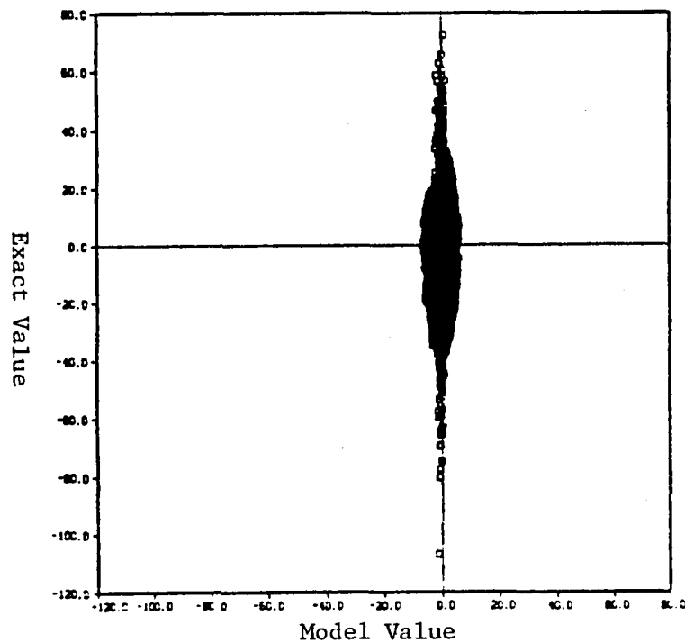
Fig. 6.2b. Smagorinsky model. "Exact" vs. model values of the divergence of the subgrid-scale Reynolds stress \partial \tau_{ij} / \partial x_j in homogeneous sheared turbulence. S = 34 and R_{SGS} = 204 .
