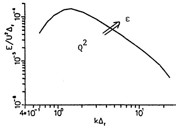
3-D Energy Spectrum
