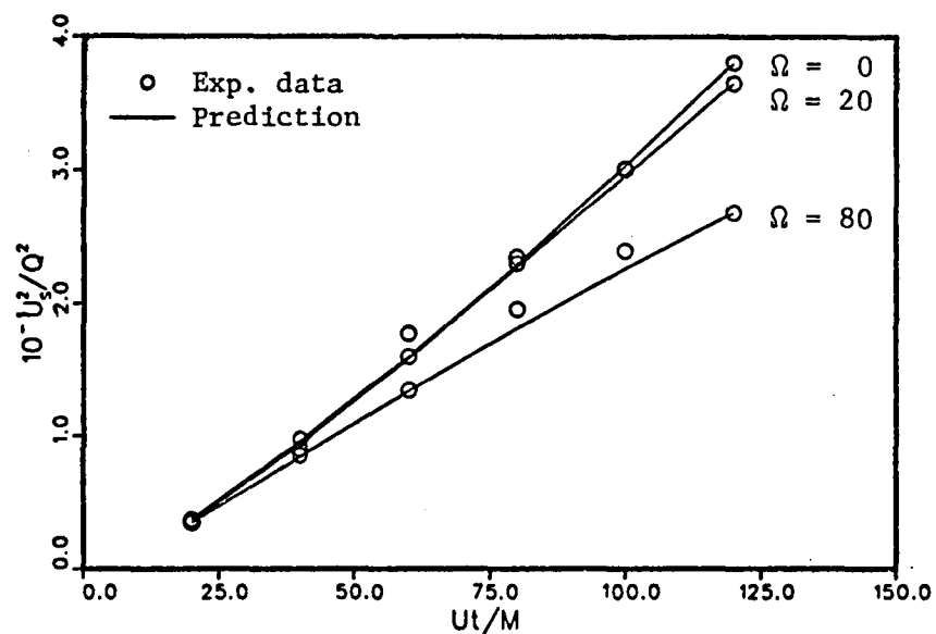
Fig. 7.7a. Two-equation model prediction of Wigeland and Nagib's (1978) experimental results on the decay of homogeneous rotating turbulence. Case A of Table 7.3.
