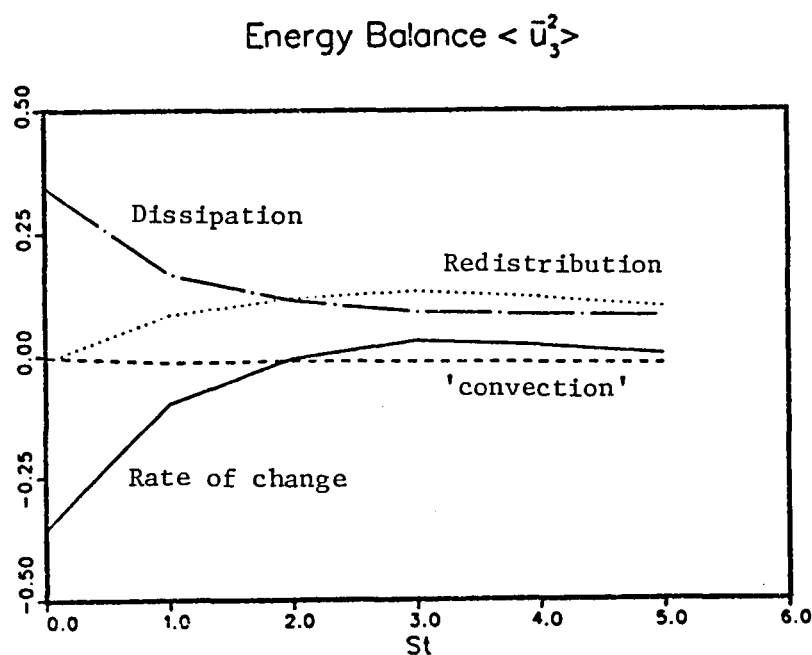
Fig. 8.6a. Time history of each spatially averaged term of the \langle \bar{u}_j^2 \rangle equation of the filtered flow field shown in Fig. 8.1a.
