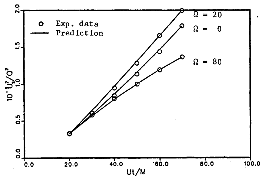
Fig. 7.7b. Two-equation model prediction of Wigeland and Nagib's (1978) experimental results on the decay of homogeneous rotating turbulence. Case B of Table 7.3.
