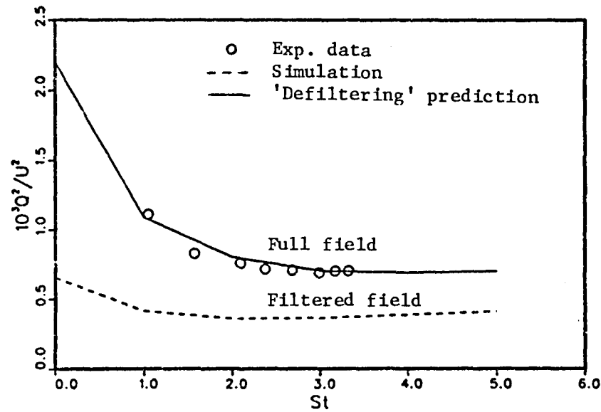
Fig. 5.6. Prediction of the full turbulence intensity of the experimental results of Champagne, Harris and Corrsin (1970) on homogeneous sheared turbulence with U = 12.4 m/s and shear rate S = 12.9 \text{ s}^{-1} . Large eddy simulation as described in caption of Fig. 4.1a.
