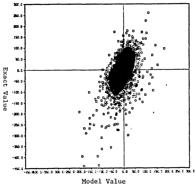
Fig. 6.3c. Scale similarity model. "Exact" vs. model values of the dissipation due to the subgrid-scale Reynolds stress \bar{u}_i \partial \tau_{ij} / \partial x_j in homogeneous isotropic turbulence. R_\lambda = 38 and R_{SGS} = 180 .
