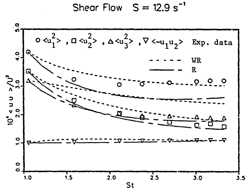
Fig. 8.9b. Time-averaged Reynolds stress model prediction of the components of the turbulence intensity and shear stress of the experiment of Fig. 8.9a.
