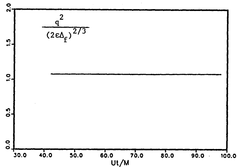
SGS Scaling
