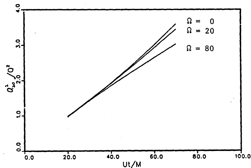
Turbulence Intensity
