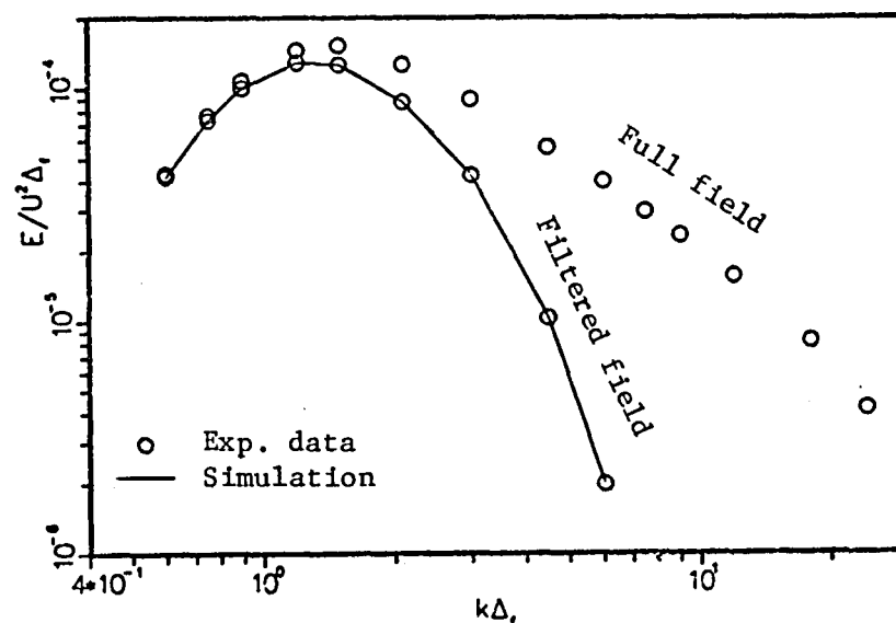
3-D Initial Energy Spectrum
