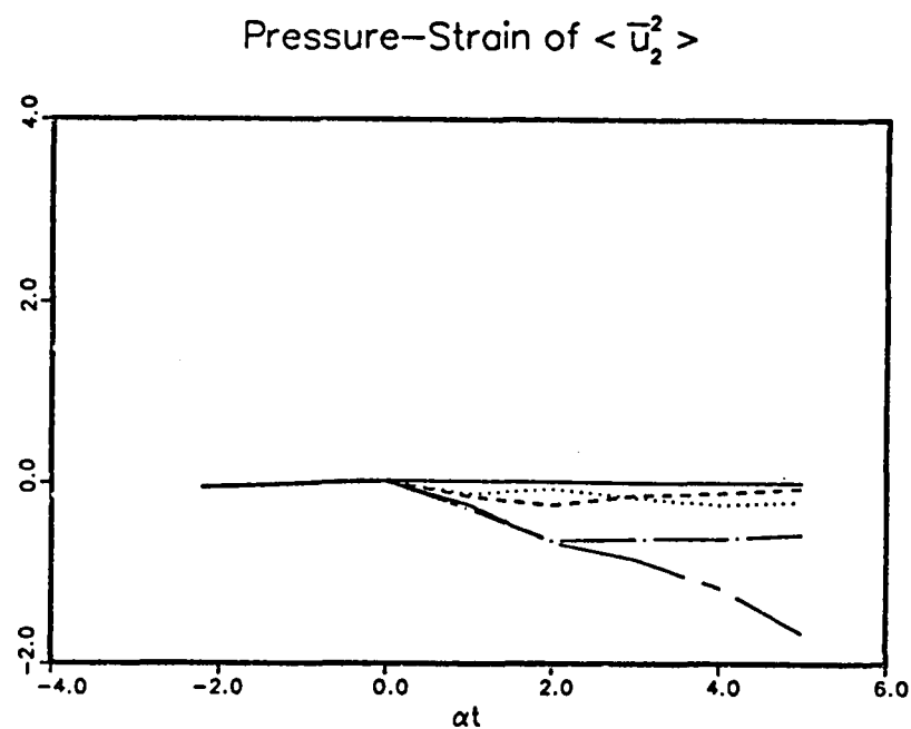
Fig. 9.14b. Time history of the component \phi_{22} of the pressure strain rate of turbulence, nondimensionalized by the dissipation rate at \alpha t = 0 , of the turbulent flows shown in Fig. 9.1b.
