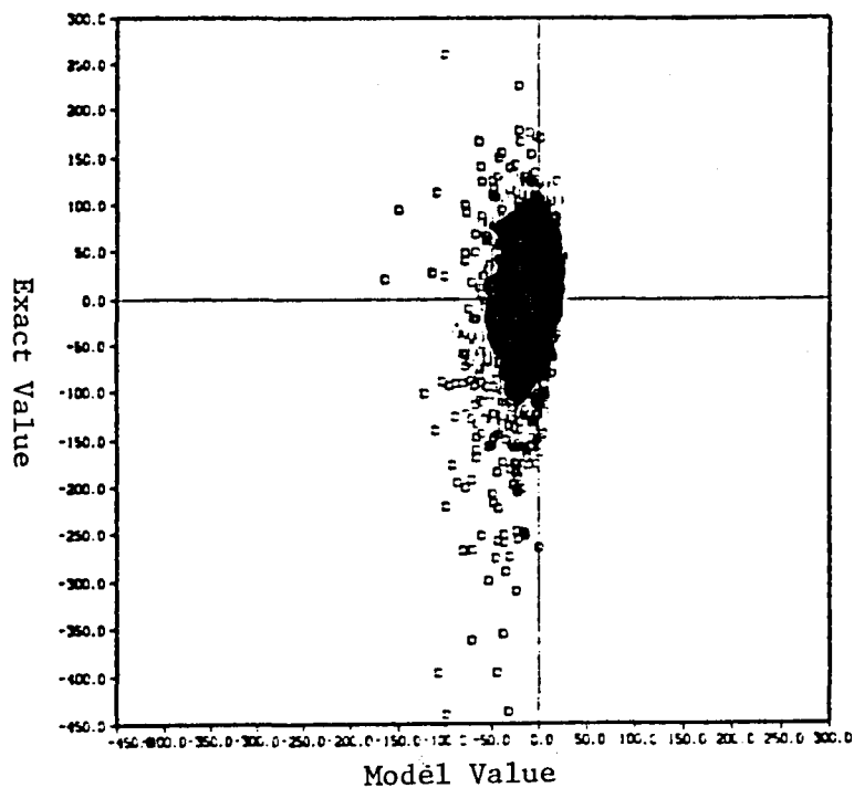
Fig. 6.1c. Smagorinsky model. "Exact" models of the dissipation caused by the subgrid-scale Reynolds stress \bar{u}_i \partial \tau_{ij} / \partial x_j in homogeneous isotropic turbulence. R_\lambda = 38 and R_{SGS} = 180 .
