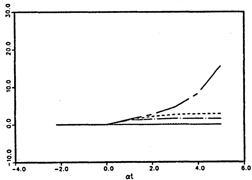
Fig. 9.6b. Time history of the production rate of turbulence, nondimensionalized by the dissipation rate at \alpha t = 0 , of the turbulent flows shown in Fig. 9.1b.
