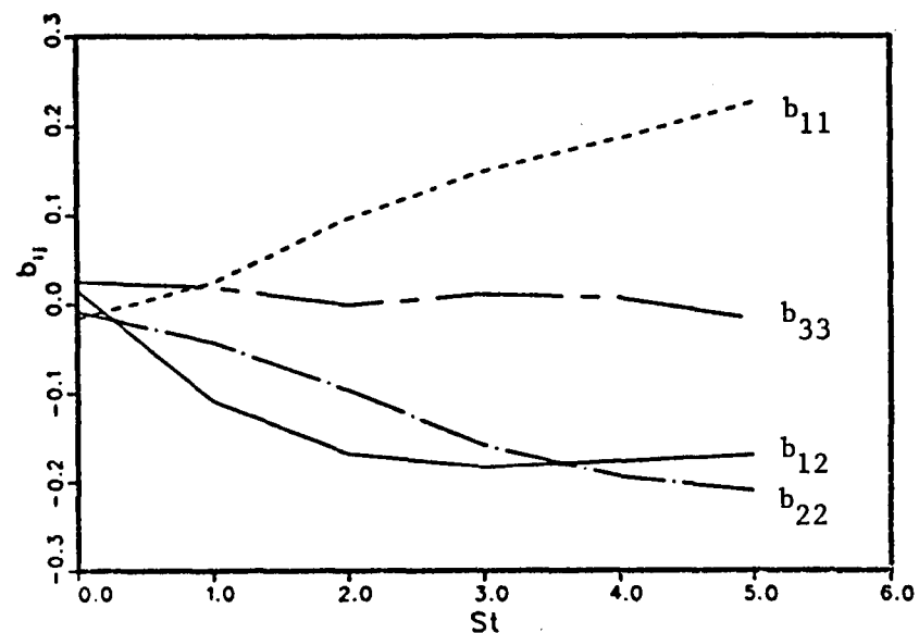
Fig. 8.2b. Time history of the components of the Reynolds stress anisotropy tensor of the filtered flow field shown in Fig. 8.1b.
