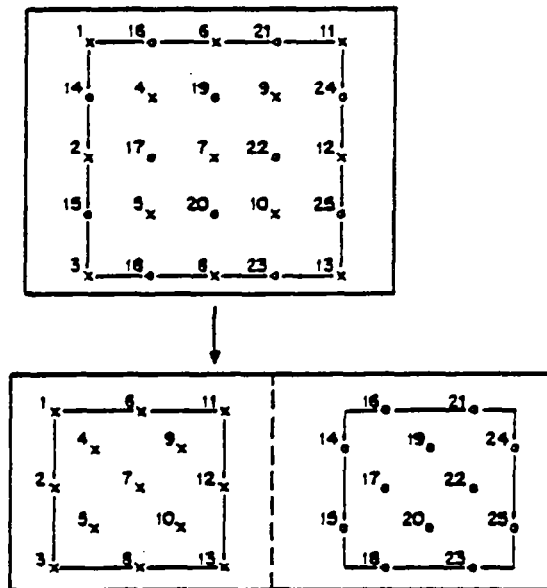
Figure 1. Mapping of the Lexicographic into the "Red-Black" Ordering. The dotted line indicates the separations of the grid points into two vectors.
