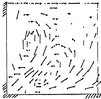
EXPERIMENT (MELLING & WHITELAW, x/D = 37 )
