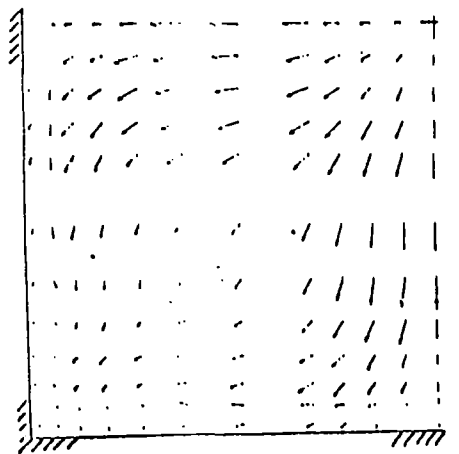
1ST-ORDER REYNOLDS STRESS ( x/D = 30 )
