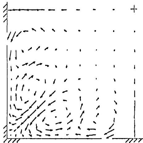
2ND-ORDER REYNOLDS STRESS ( x/D = 30 )
