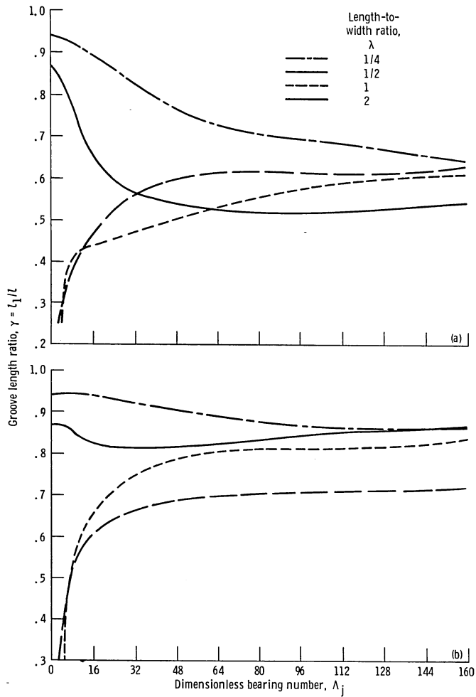
Figure 2.4-12.—Chart for determining optimal groove length ratio. (From Hamrock and Fleming, 1971.)
