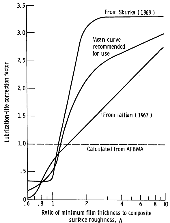
Figure 3.6-23.—Chart for determining lubrication-life correction factor. (From Bamberger, et al., 1971.)
