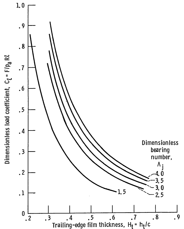
Figure 2.4-7.—Chart for determining load coefficient. Angular extent of pad, \alpha_p , 94.5^\circ ; ratio of angle between pad leading edge and pivot to \alpha_p , \varphi_p/\alpha_p , 2/3 ; length-to-width ratio, \lambda , 1.0. (From Gunter et al., 1964.)
