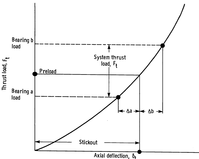
Figure 3.6-18.—Thrust load-axial deflection curve for a typical ball bearing. (From Hamrock and Anderson, 1983.)
