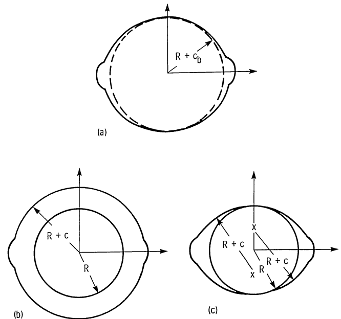
(a) Largest shaft that fits in bearing. (b) m = 0 , largest shaft = R + c , bearing clearance c_b = c . (c) m = 1.0 , largest shaft = R , bearing clearance c_b = 0 .
