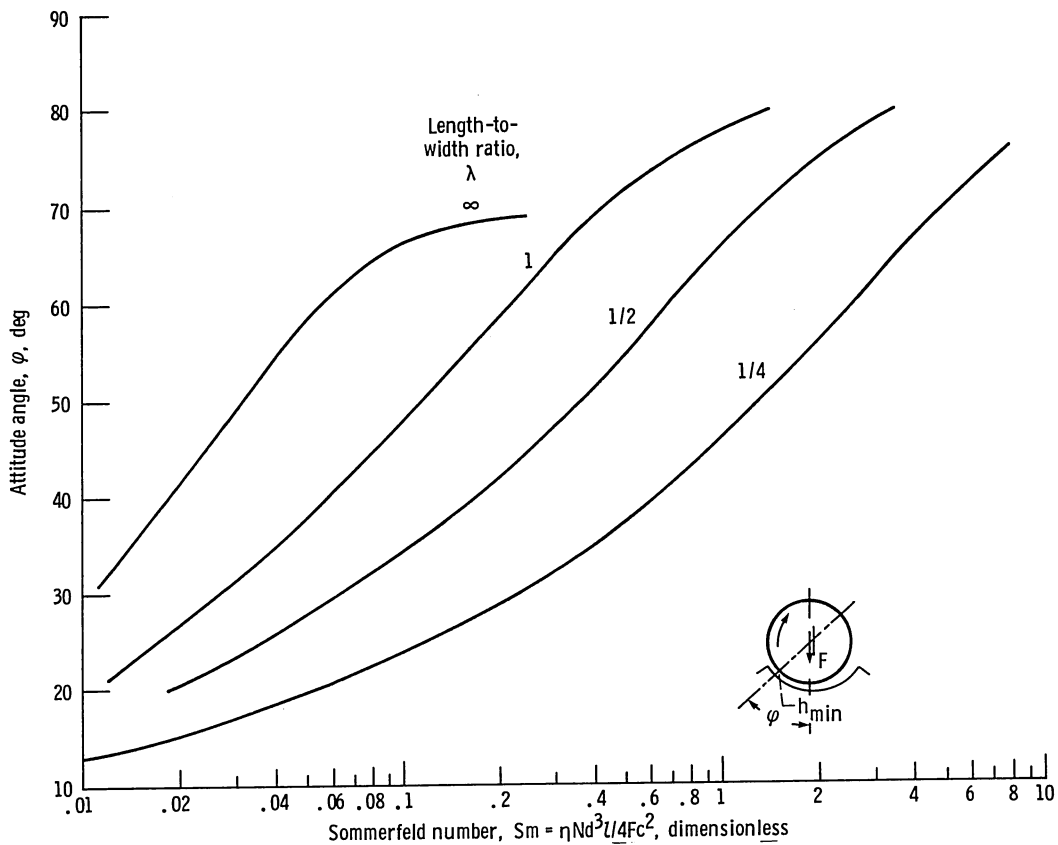
Figure 2.1-5.—Design figure showing attitude angle (position of minimum film thickness) and Sommerfeld number for full journal bearings, centrally loaded. (Adapted from Raimondi and Boyd, 1958.)
