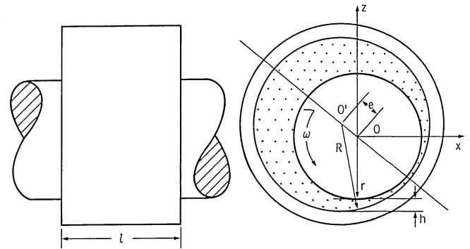
Figure 2.1-1.—Journal bearing.
