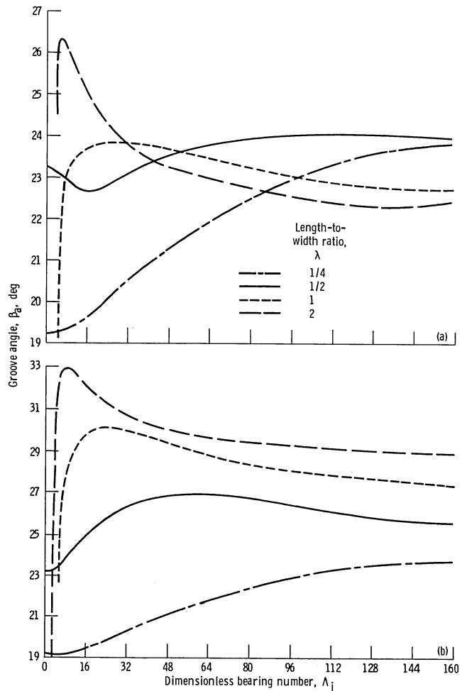
Figure 2.4-13.—Chart for determining optimal groove angle. (From Hamrock and Fleming, 1971.)
