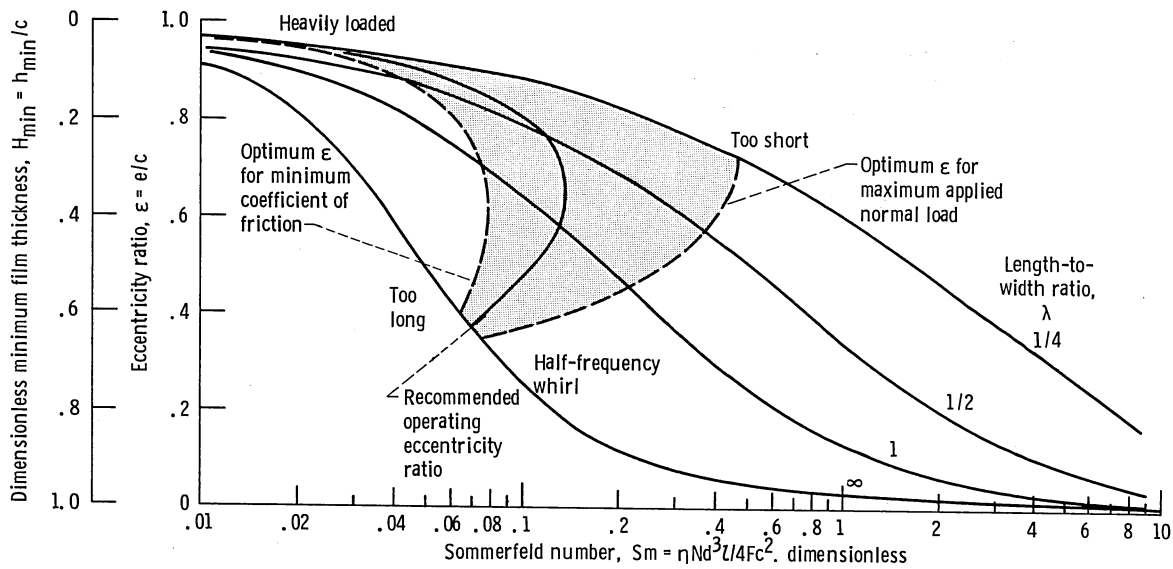
Figure 2.1-2.—Design figure showing eccentricity ratio, dimensionless minimum film thickness, and Sommerfeld number for full journal bearings. (Adapted from Raimondi and Boyd, 1958.)
