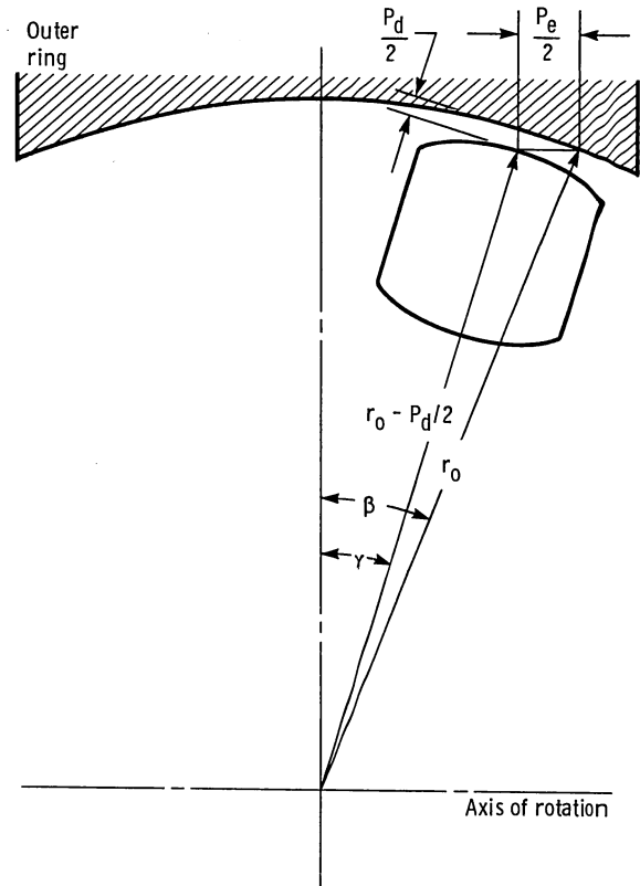
Figure 3.6-9.—Schematic diagram of spherical roller bearing, showing diametral play and endplay. (From Hamrock and Anderson, 1983.)
