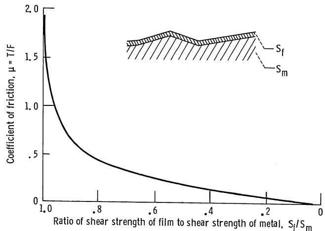
Figure 4.2-2.—Chart for determining friction as function of shear strength ratio. (From Godfrey, 1968.)
