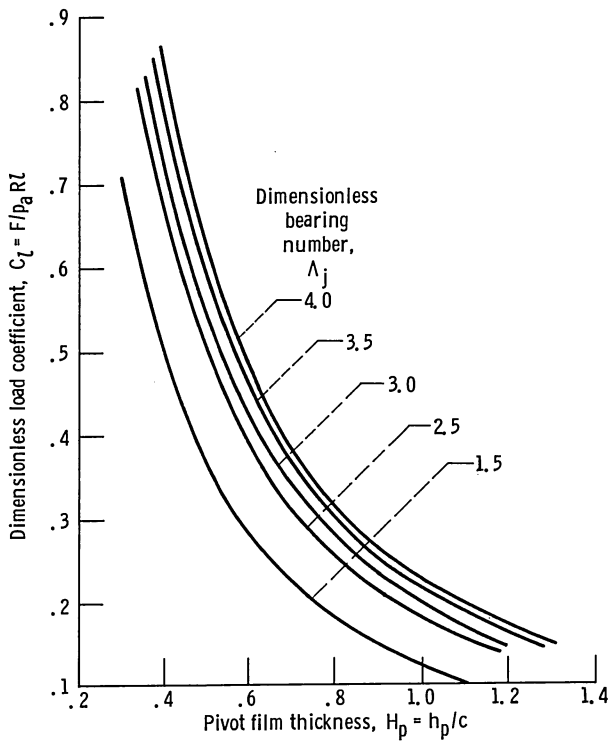
Figure 2.4-6.—Chart for determining load coefficient. Angular extent of pad, \alpha_p , 94.5^\circ ; ratio of angle between pad leading edge and pivot to \alpha_p , \varphi_p/\alpha_p , 2/3 ; length-to-width ratio, \lambda , 1.0. (From Gunter et al., 1964.)
