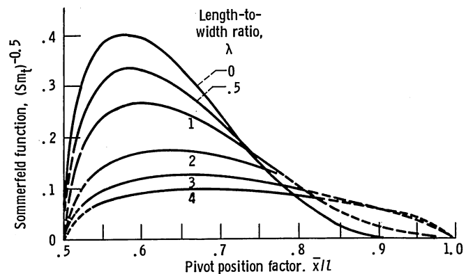
Figure 2.2-11.—Chart for determining outlet film thickness for pivoted-pad thrust bearings. (From Raimondi and Boyd, 1955.)
