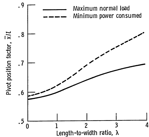
Figure 2.2-10.—Chart for determining pivot position corresponding to maximum load or minimum power loss for various pad proportions—pivoted-pad bearings. (From Raimondi and Boyd, 1955.)
