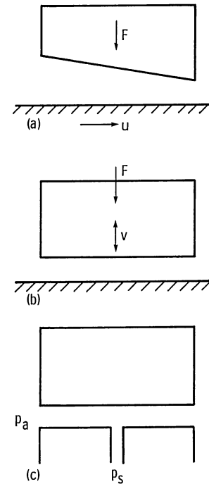
(a) Slider bearing. (b) Squeeze film bearing. (c) Externally pressurized bearing.
