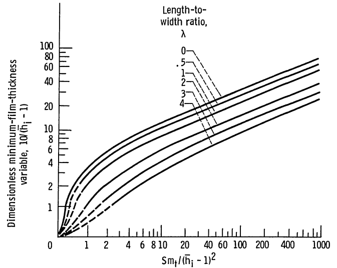
Figure 2.2-4.—Chart for determining minimum film thickness for fixed-incline-pad thrust bearings. (From Raimondi and Boyd, 1955.)
