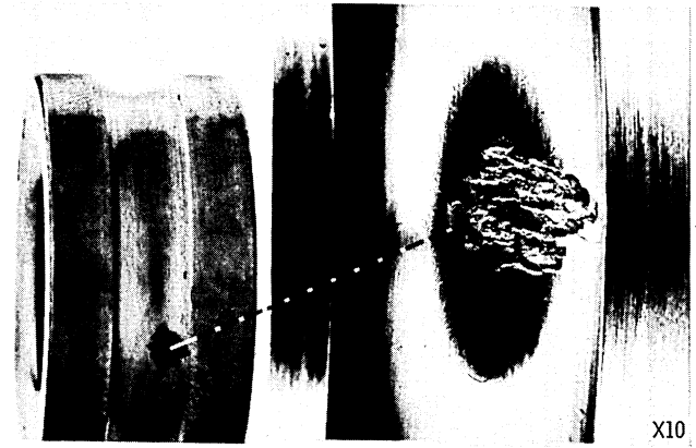
Figure 3.6-19.—Typical fatigue spall.
