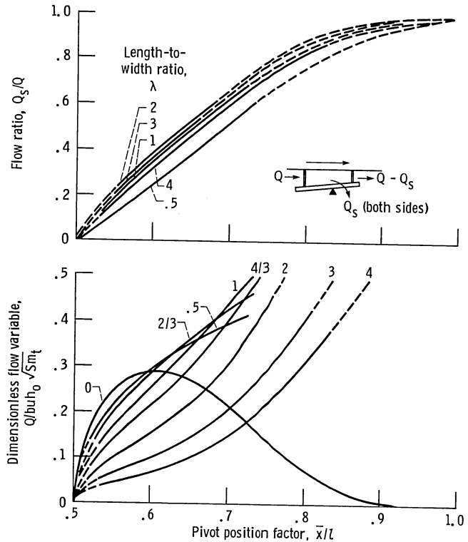
Figure 2.2-15.—Chart for determining lubricant flow for pivoted-pad thrust bearings. (From Raimondi and Boyd, 1955.)
