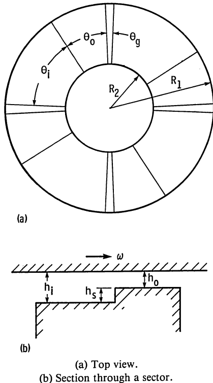
Figure 2.2-16.—Configuration of step-sector thrust bearing. (From Hamrock, 1983.)
