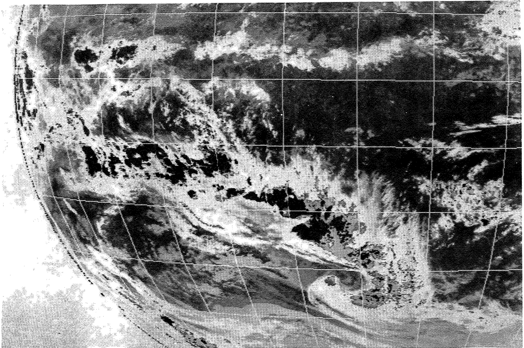
Figure 1. GOES West image at 1815Z 12 January 1979 showing the extent of the SPCZ cloud band. The image has been enhanced to emphasize the predominance of deep convection in the tropical portion and the existence of baroclinic waves at higher latitudes.
