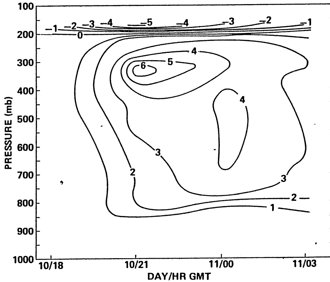
Figure 1. Convective diabatic heating rate in Deg/Day averaged over the SESAME network (1400 km on a side). Heating was diagnosed from a cumulus mass flux method using observed rainfall and cloud top heights determined from GOES data.
