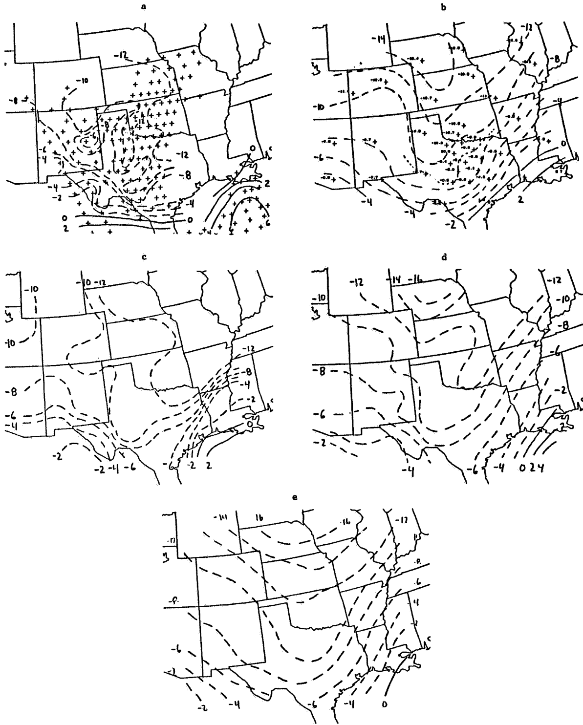
Figure 1. Subjective manual analysis of 700mb temperatures at 2045 GMT 6 March 1982 for VAS (a) and rawinsonde (b) data sets. Conventional two-pass objective analysis of VAS data (c), and the modified scheme gridded temperature field (d) produced substituting a LFM forecast field (e) for the first pass. Temperatures are in degrees C.
