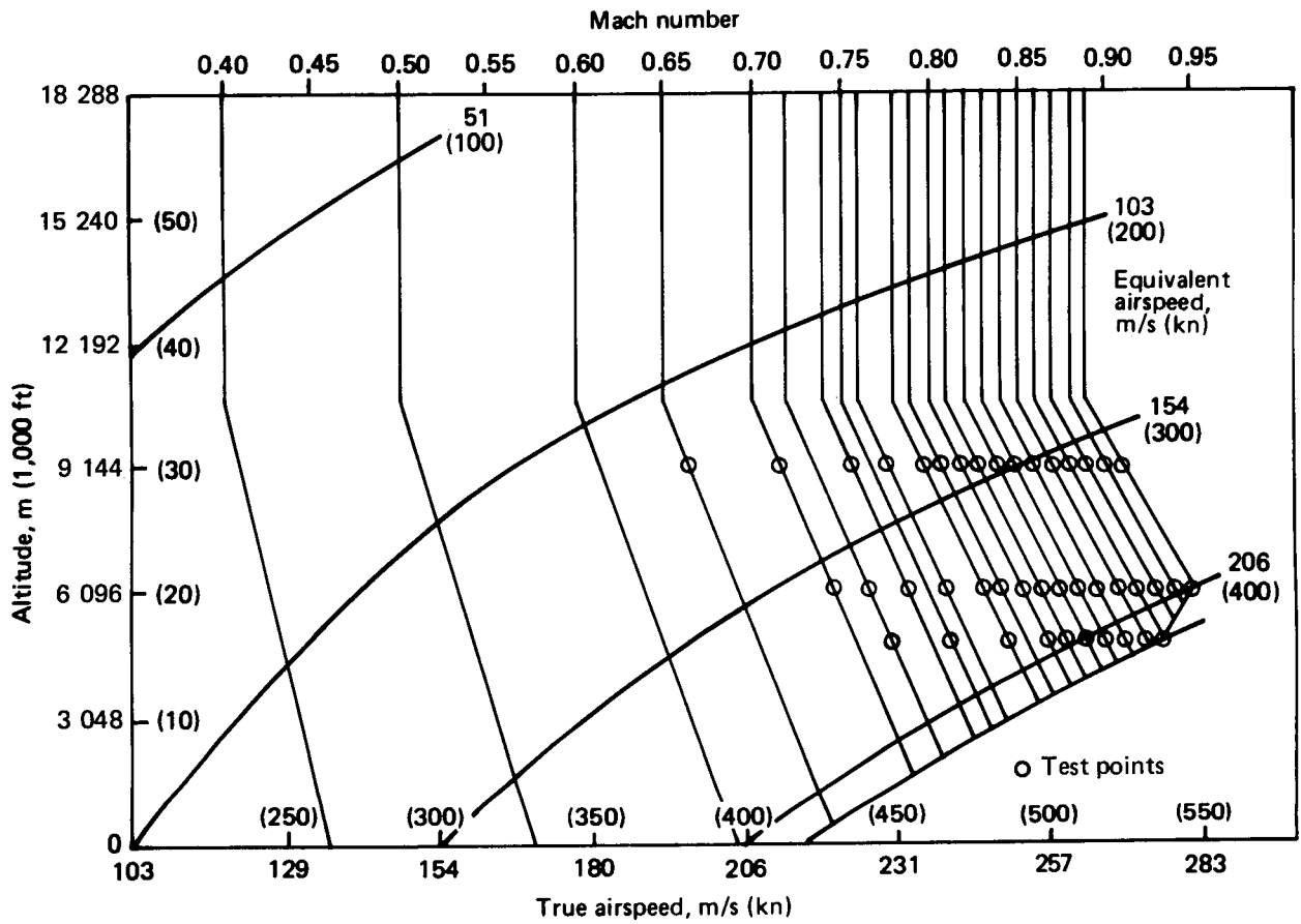
Figure 7. Speed and Altitude Test Points
