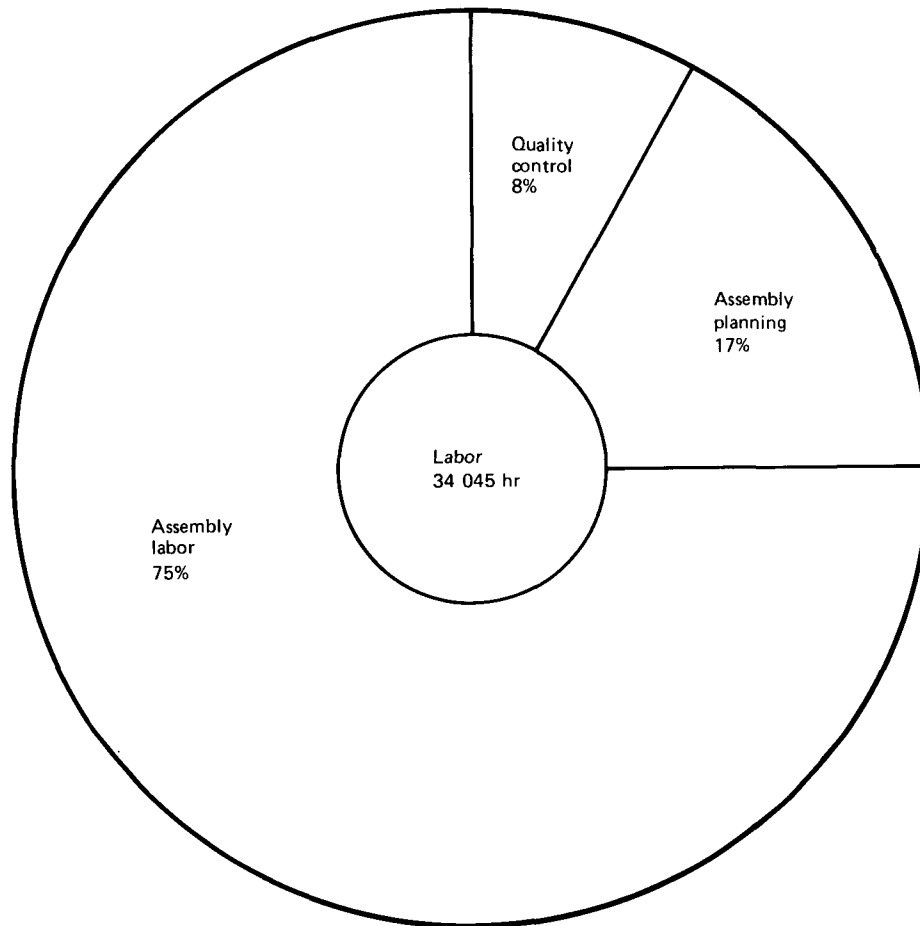
Figure 13. Total Recurring and Nonrecurring Assembly Labor Hours—5½ Shipsets
