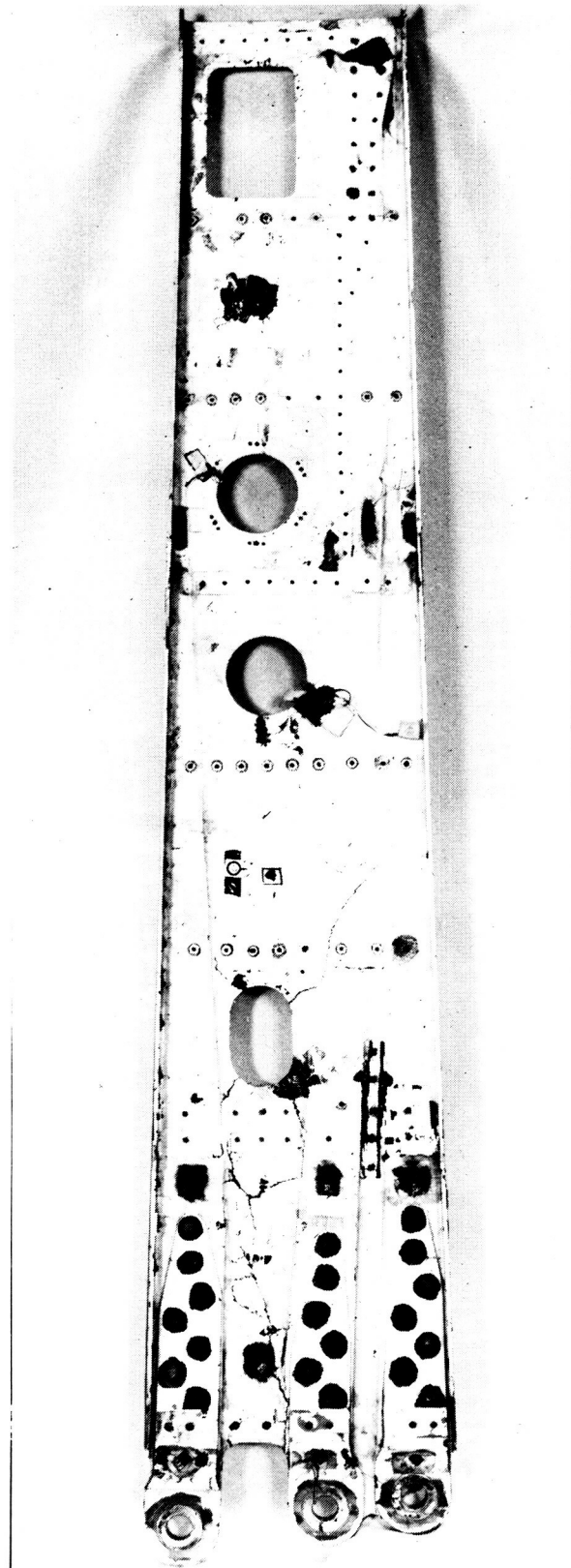
Figure 3. Rear-Spar Failure—Load Case 4010 With Upper Pin Removed
