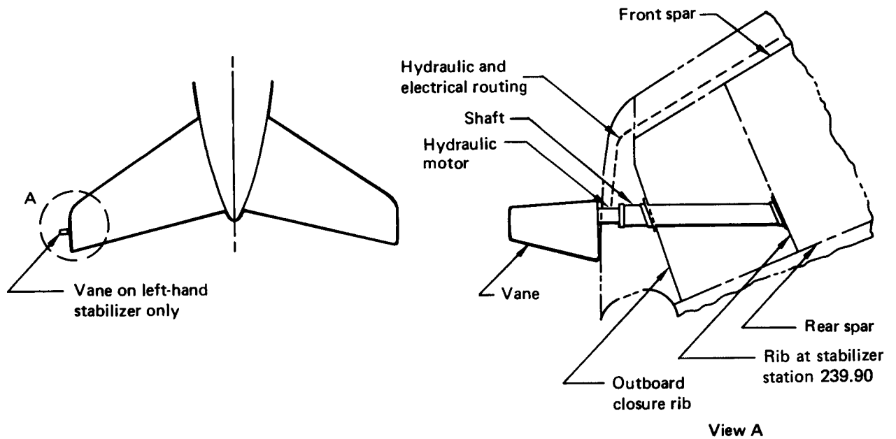
Figure 8. Flutter Vane Installation
