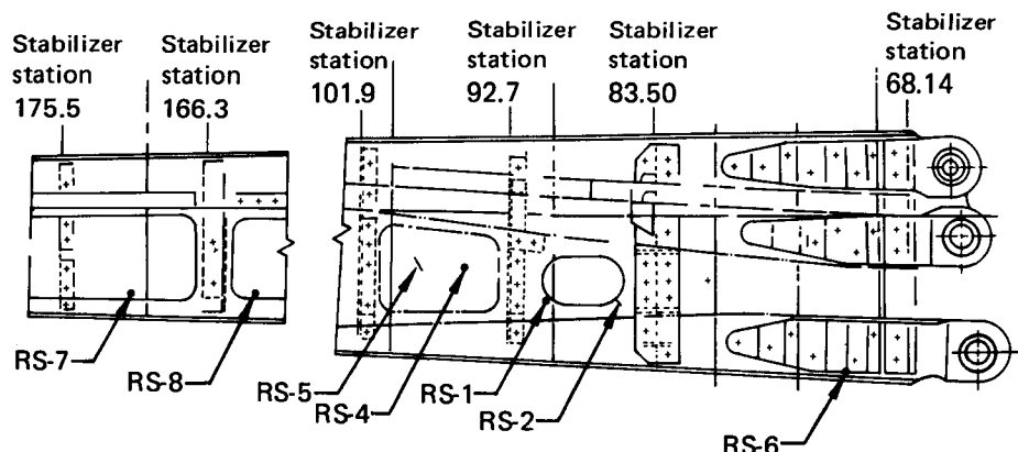
Rear Spar Damage Location
