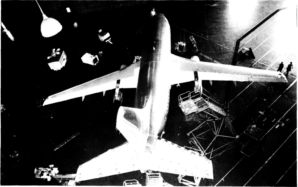
Figure 6. Ground Vibration Test Setup
