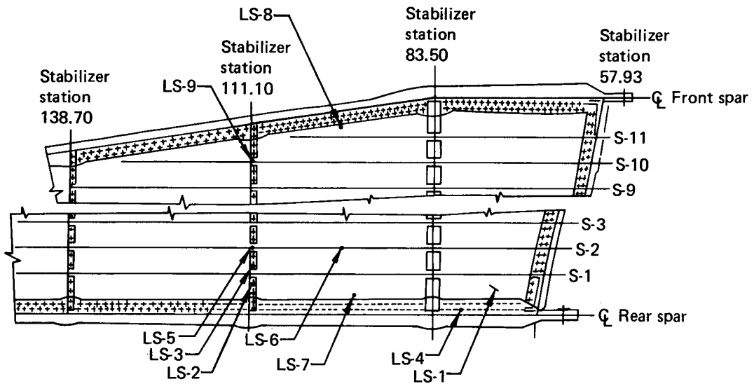
Lower Surface Damage Location
