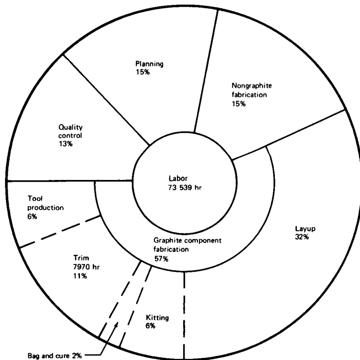
Figure 12. Total Recurring and Nonrecurring Fabrication Hours—5½ Shipsets
