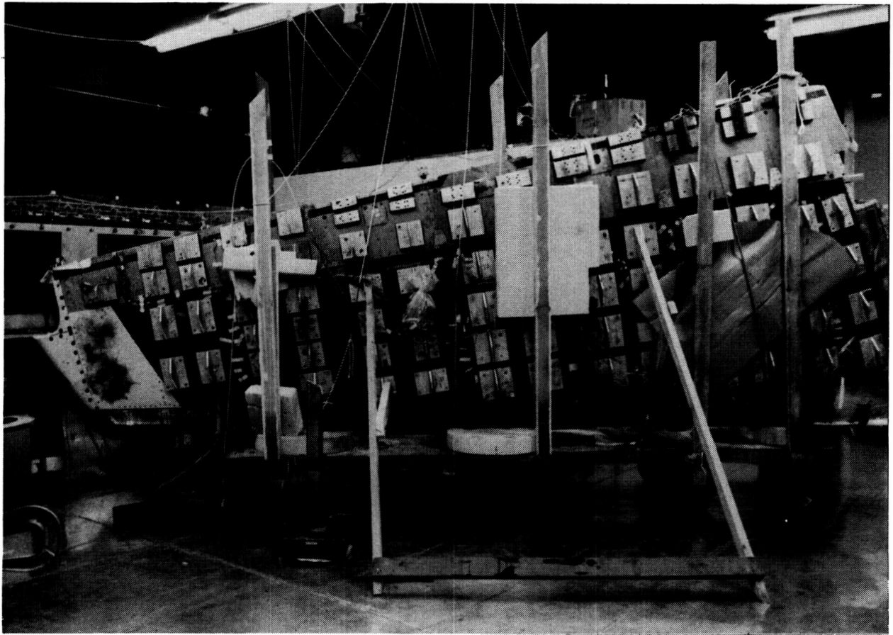
Figure 4. Lightning Strike Test
