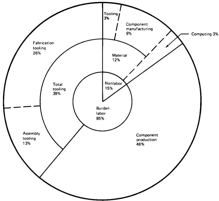
Figure 9. Total Recurring and Nonrecurring Production Costs by Major Element—5½ Shipsets
