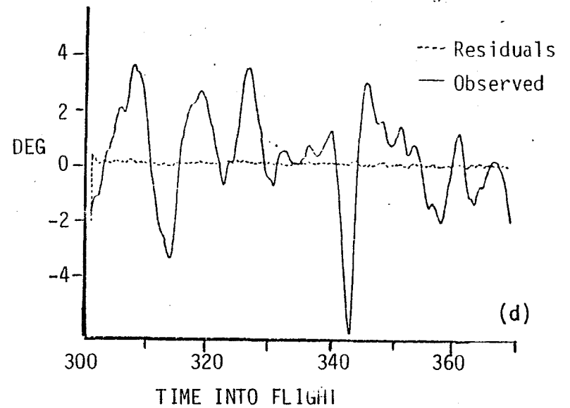
Time History: Model Residuals and Observed Roll Series
