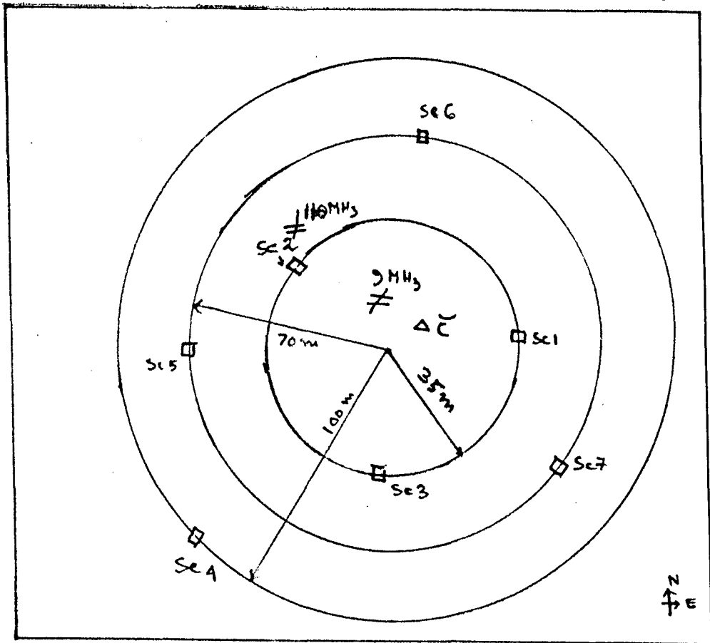
Fig 1. The array. Sc 1-Sc 7 - Positions of scintillators ≠ -positions of Antennas, \Delta -position of C detector.
