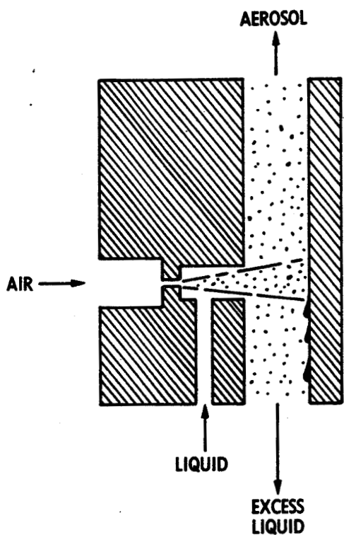
Figure 2. Collison Nebulizer
