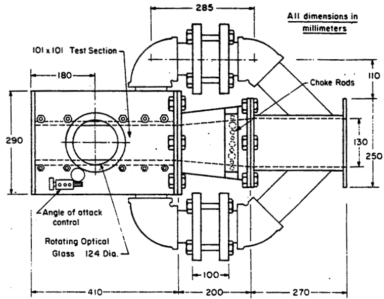
Figure 1. Schematic of the transonic tunnel test section.
