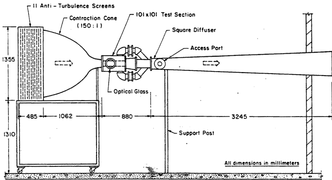
Figure 2. Schematic of the transonic tunnel.
