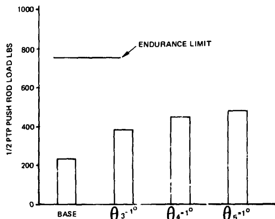
Figure 5. Increase in Pushrod Load due to 1^\circ HHC Input
