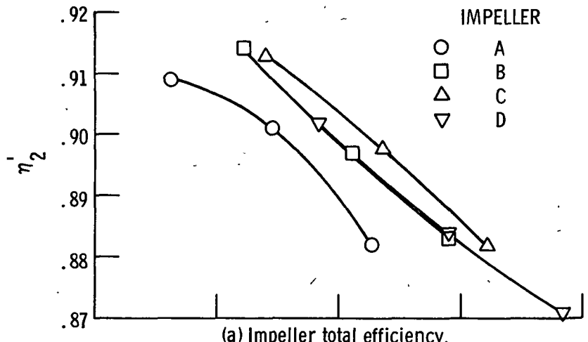
(a) Impeller total efficiency.
