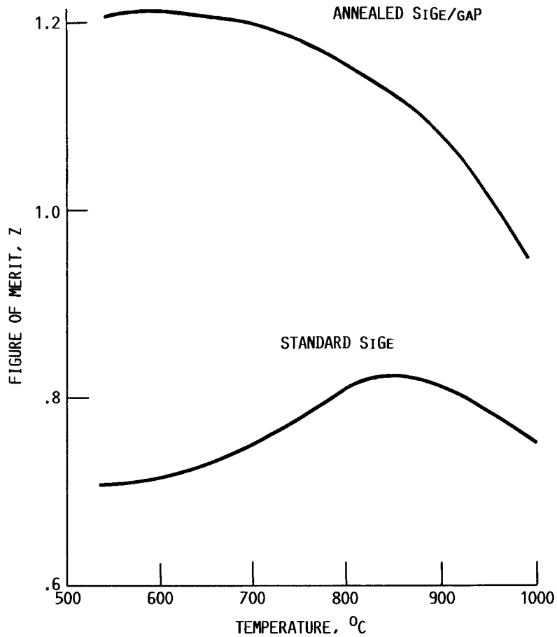
FIGURE 7. - PERFORMANCE IMPROVEMENT OF SiGe/GAP ALLOYS.
