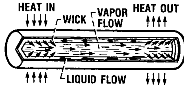
HEAT PIPE RADIATOR
