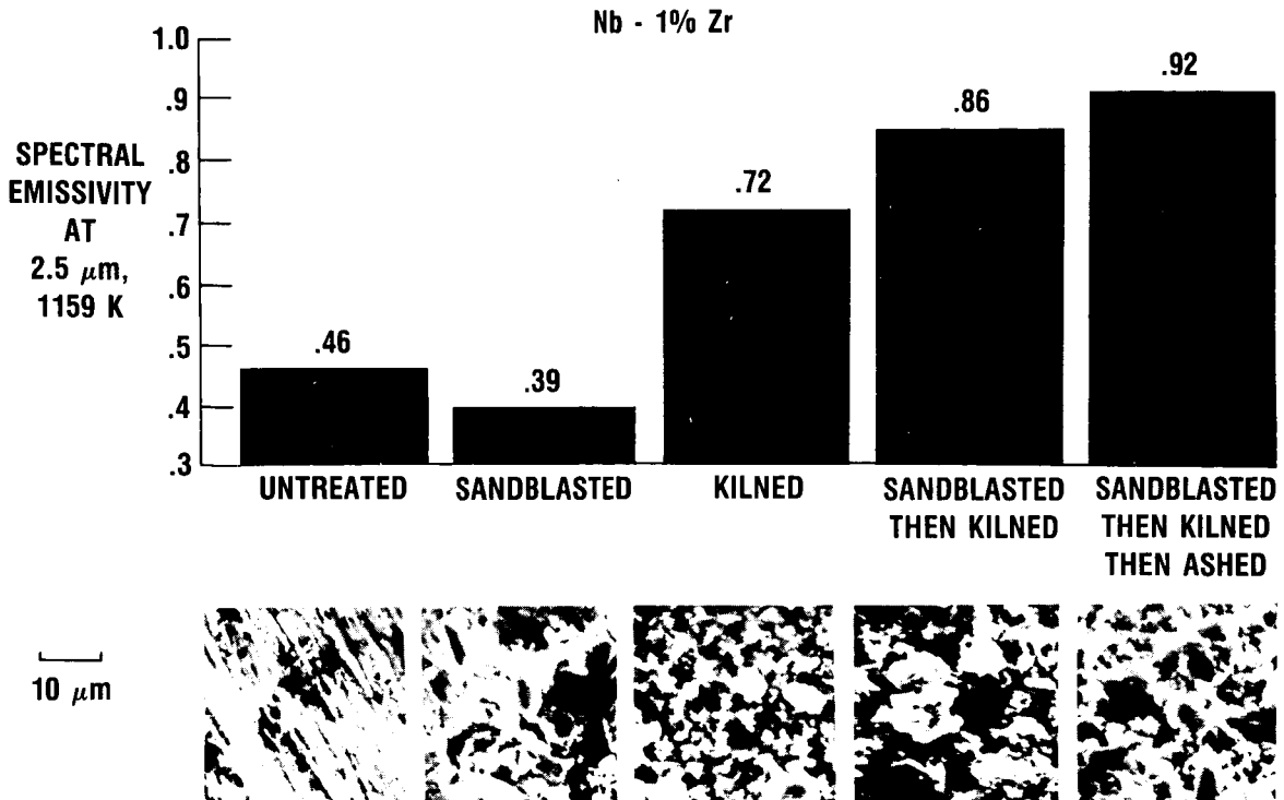
FIGURE 10. - RADIATOR SURFACE MODIFICATION FOR HIGH EMISSIVITY.
