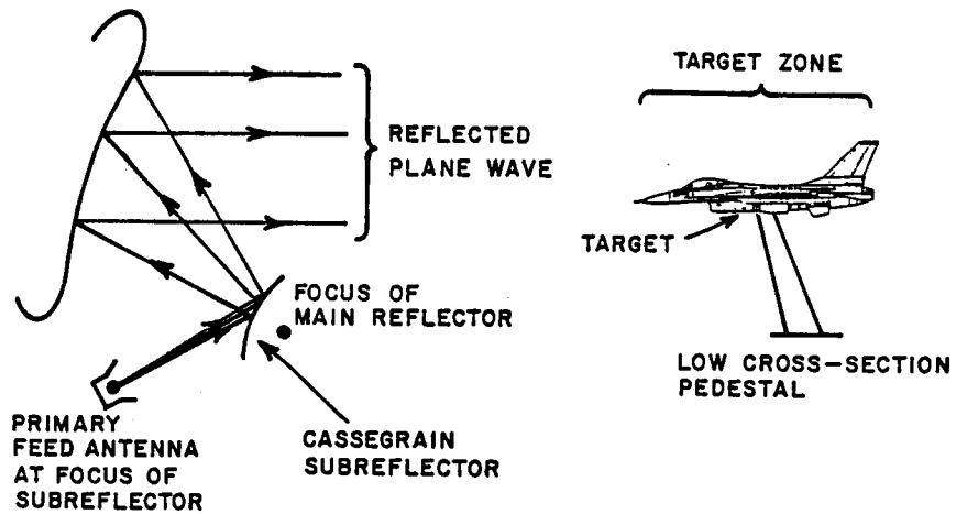
(c) CASSEGRAIN SUBREFLECTOR FED SYSTEM
