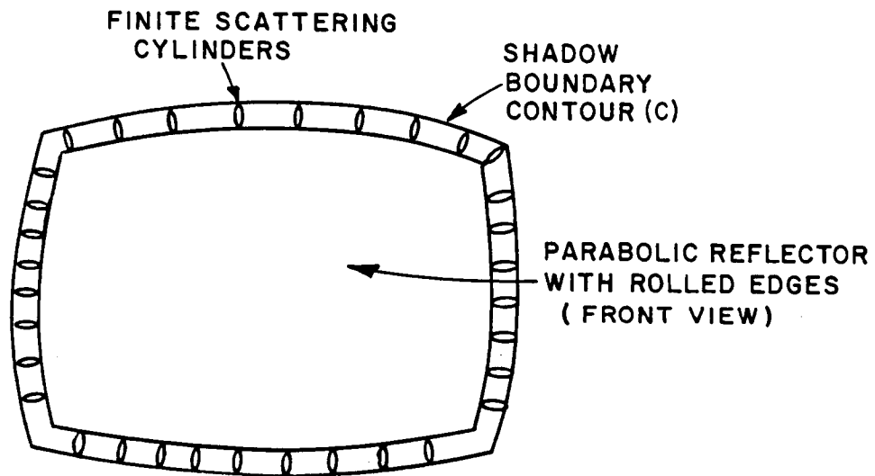
(b) Finite scattering cylinders along the entire shadow boundary contour of a blended rolled edge.
