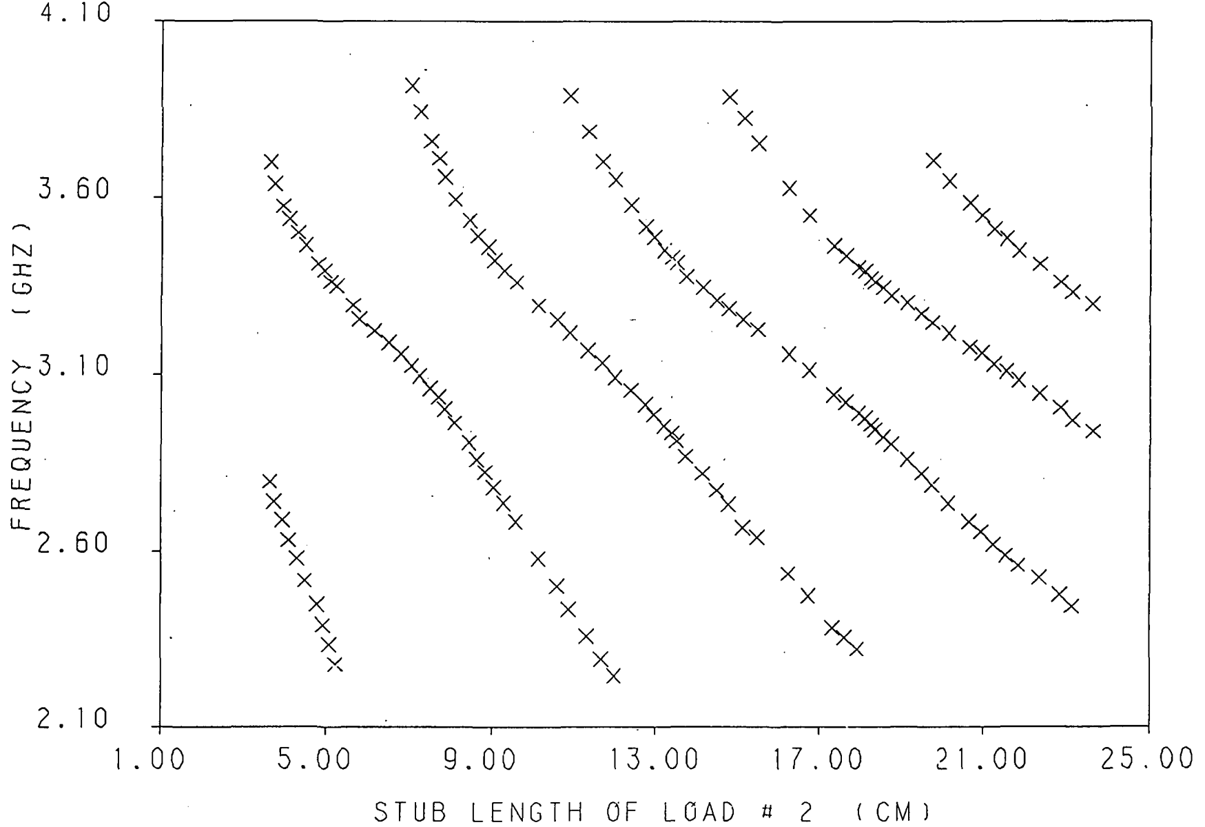
Fig. 3.42 Frequency of lower linearly polarized band ( the y-polarized band ) versus the short circuit stub length of load #2 for a loaded 2.96 by 2.96 cm square patch with a feed location of (.25, .25 cm ), and load insets of d = .11 cm .
