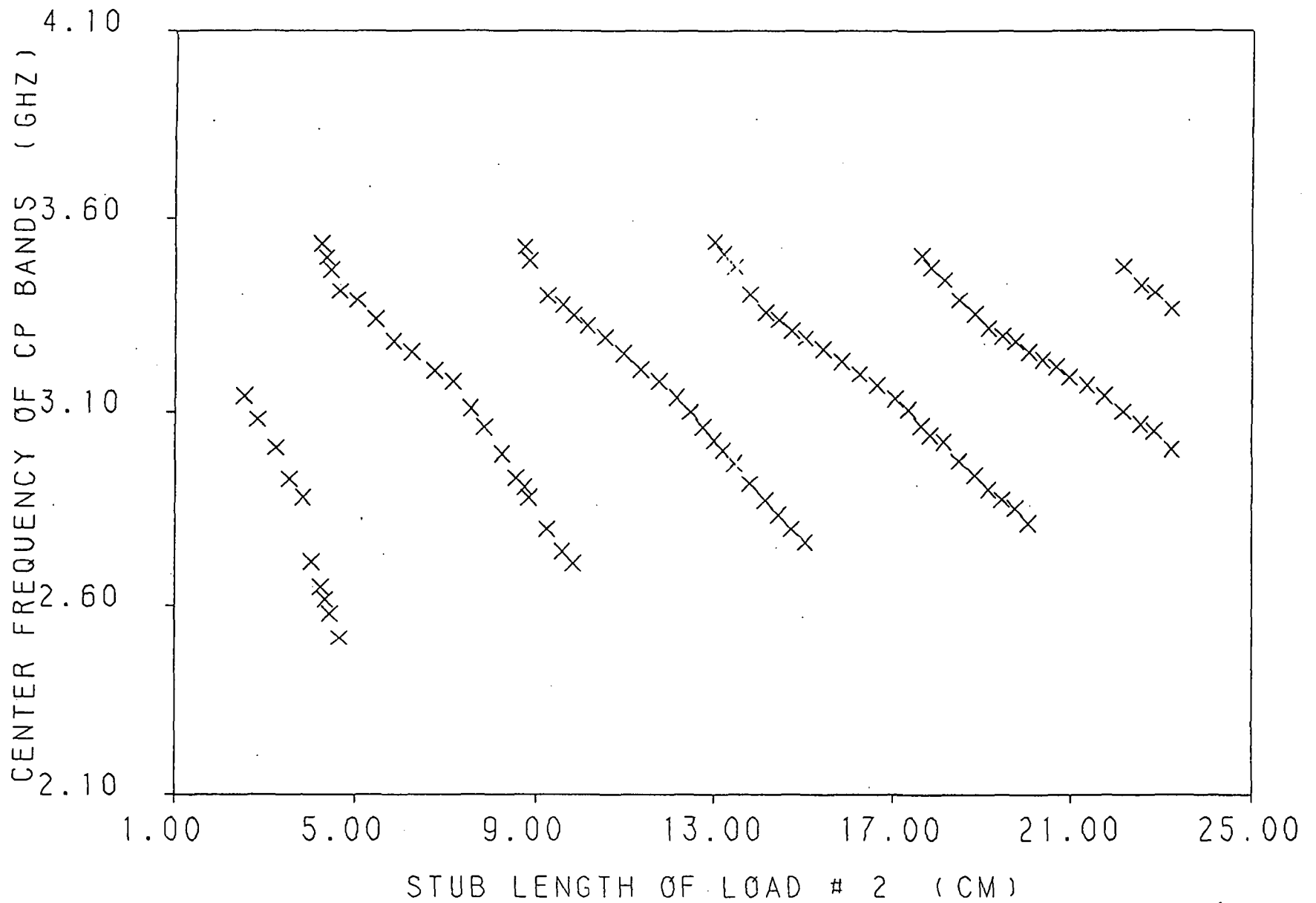
Fig. 3.97 Center frequency of cp bands versus the short circuit stub length of load # 2 for a loaded 2.96 by 2.96 cm square patch with a feed location of (1.05, .45 cm ), and load insets of d = .35 cm .
