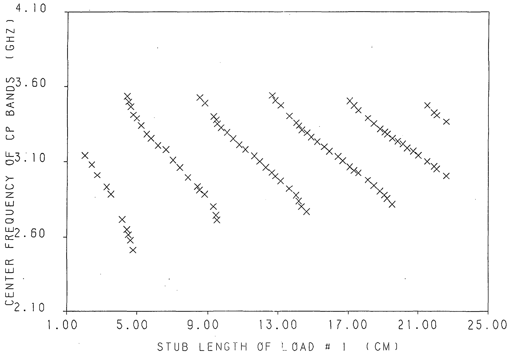
Fig. 3.96 Center frequency of cp bands versus the short circuit stub length of load # 1 for a loaded 2.96 by 2.96 cm square patch with a feed location of (1.05, .45 cm), and load insets of d = .35 cm.
