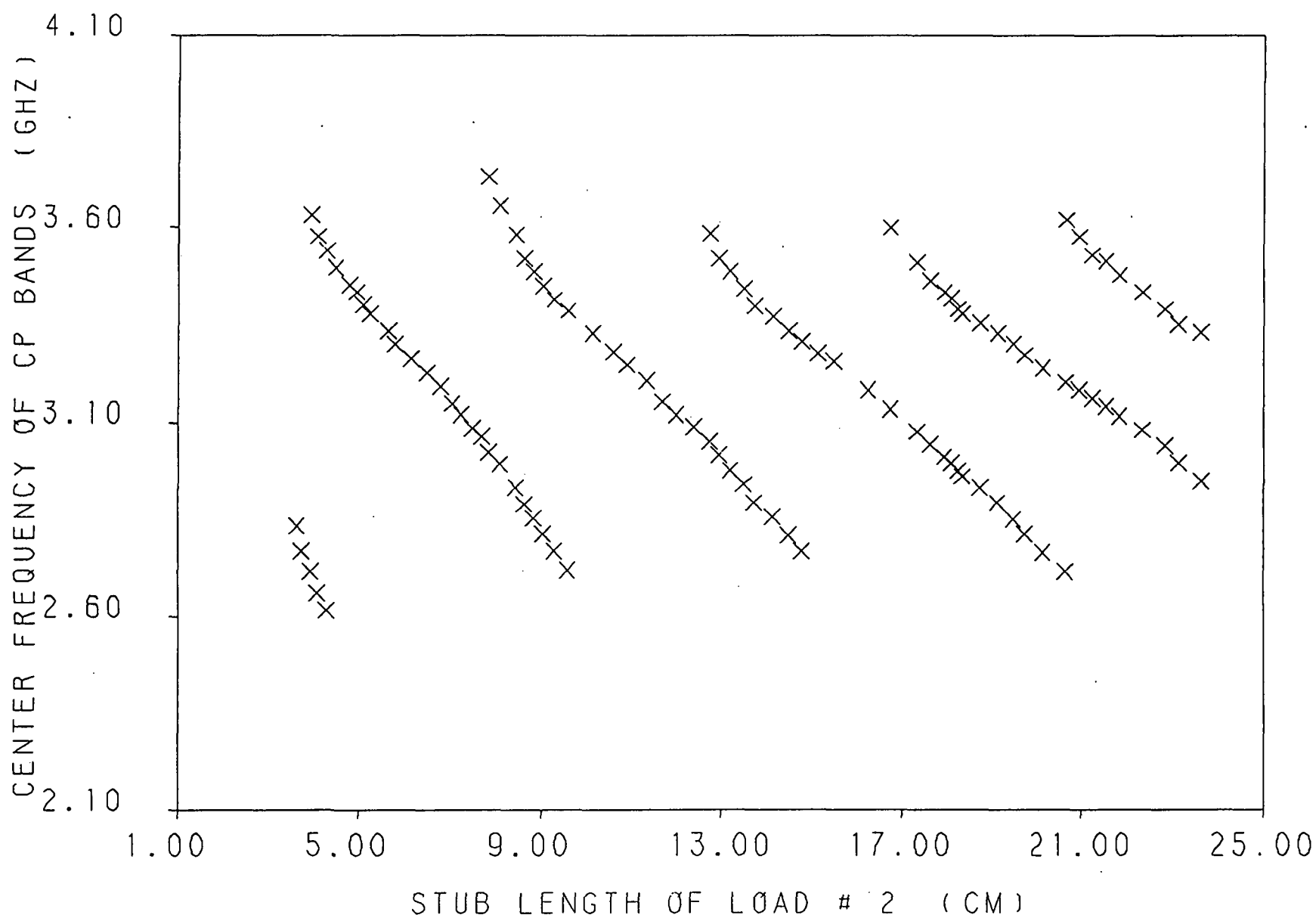
Fig. 3.46 Center frequency of cp bands versus the short circuit stub length of load # 2 for a loaded 2.96 by 2.96 cm square patch with a feed location of (.25, .25 cm), and load insets of d = .11 cm.
