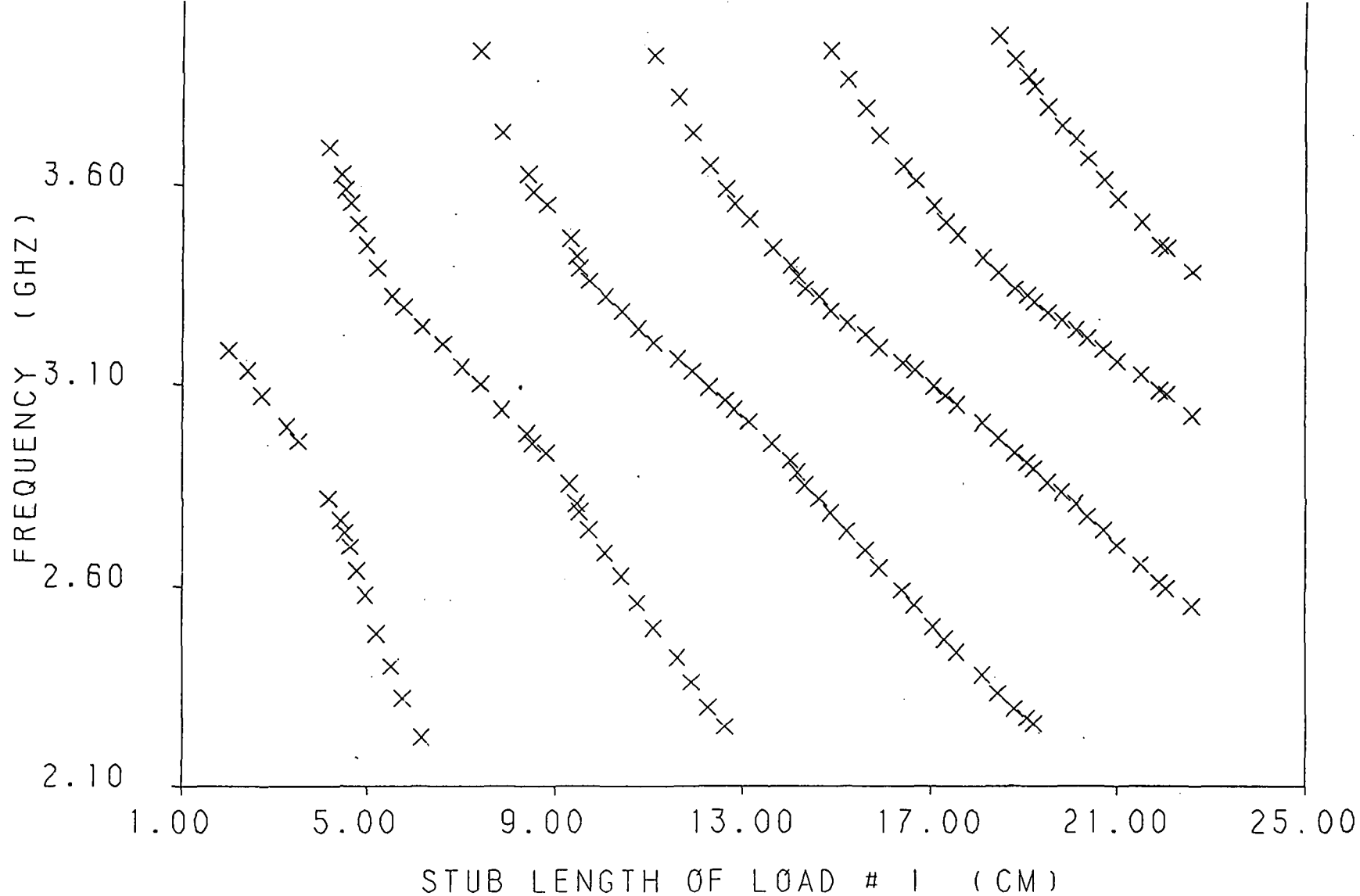
Fig. 3.92 Frequency of upper linearly polarized band ( the x -polarized band ) versus the short circuit stub length of load #1 for a loaded 2.96 by 2.96 cm square patch with a feed location of (1.05, .45 cm ), and load insets of d = .35 cm .
