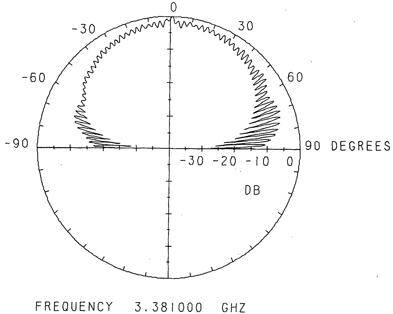
Fig. 3.52 Spinning linear pattern for the upper cp band of the fourth mode for a loaded 2.96 by 2.96 cm square patch with a feed location of (.25, .775 cm), load insets of d = .11 cm, and stub lengths of s_1 = 18.2 cm and s_2 = 18.53 cm.
