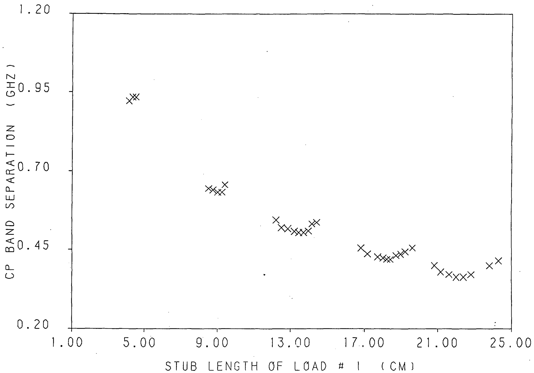
Fig. 3.75 Cp band separation versus the short circuit stub length of load # 1 for a loaded 2.96 by 2.96 cm square patch with a feed location of (1.05, .45 cm), and load insets of d = .11 cm.
