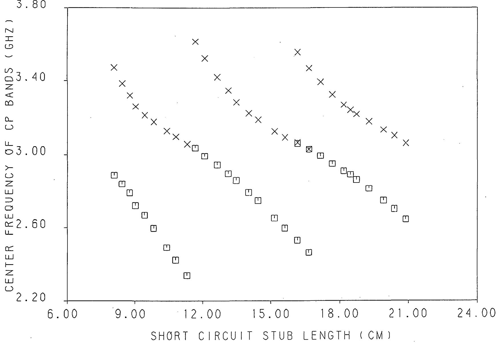
Fig. 3.26 Center frequency of cp bands versus the average short circuit stub length for a loaded 3.13 by 2.90 cm rectangular patch with a feed location of (.48, .52 cm), and load insets of d = .70 cm .
