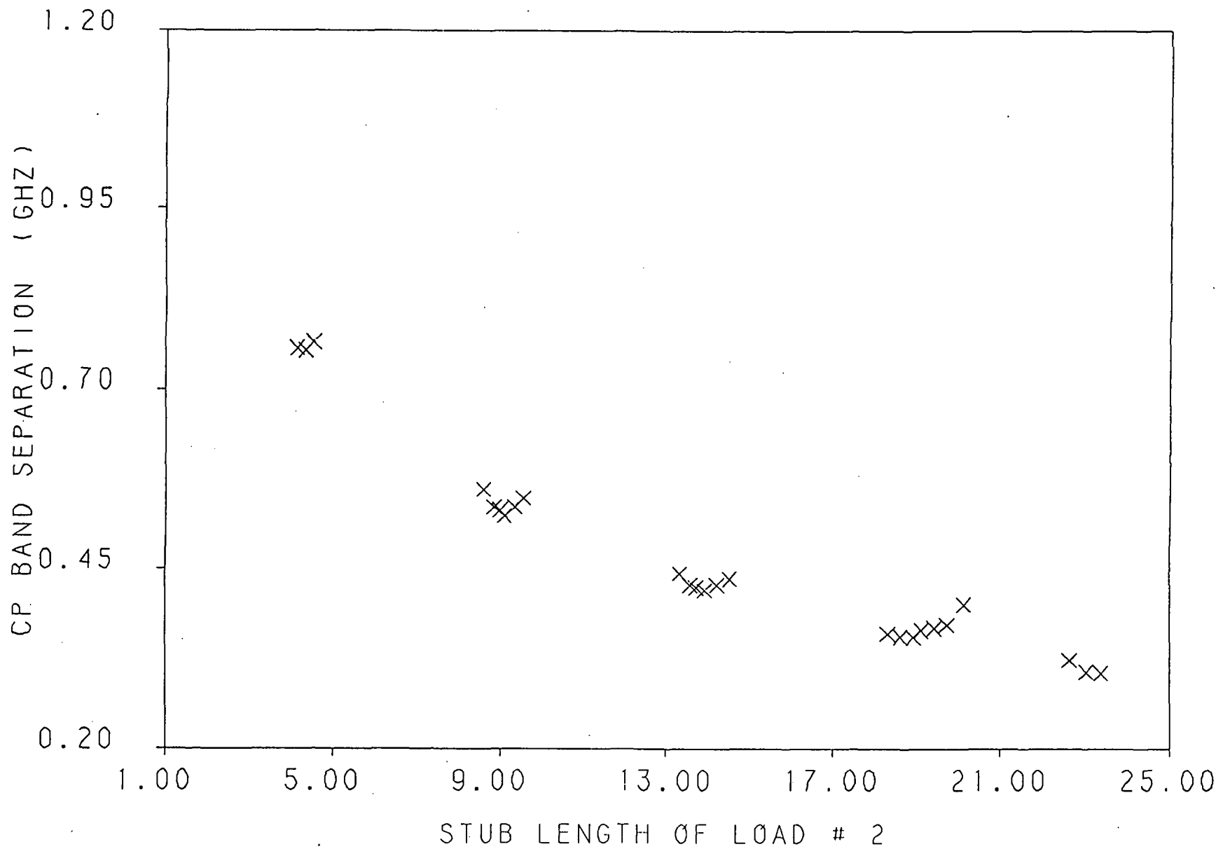
Fig. 3.122 Cp band separation versus the short circuit stub length of load # 2 for a loaded 2.96 by 2.96 cm square patch with a feed location of (.85, .45 cm ), and load insets of d = .60 cm .
