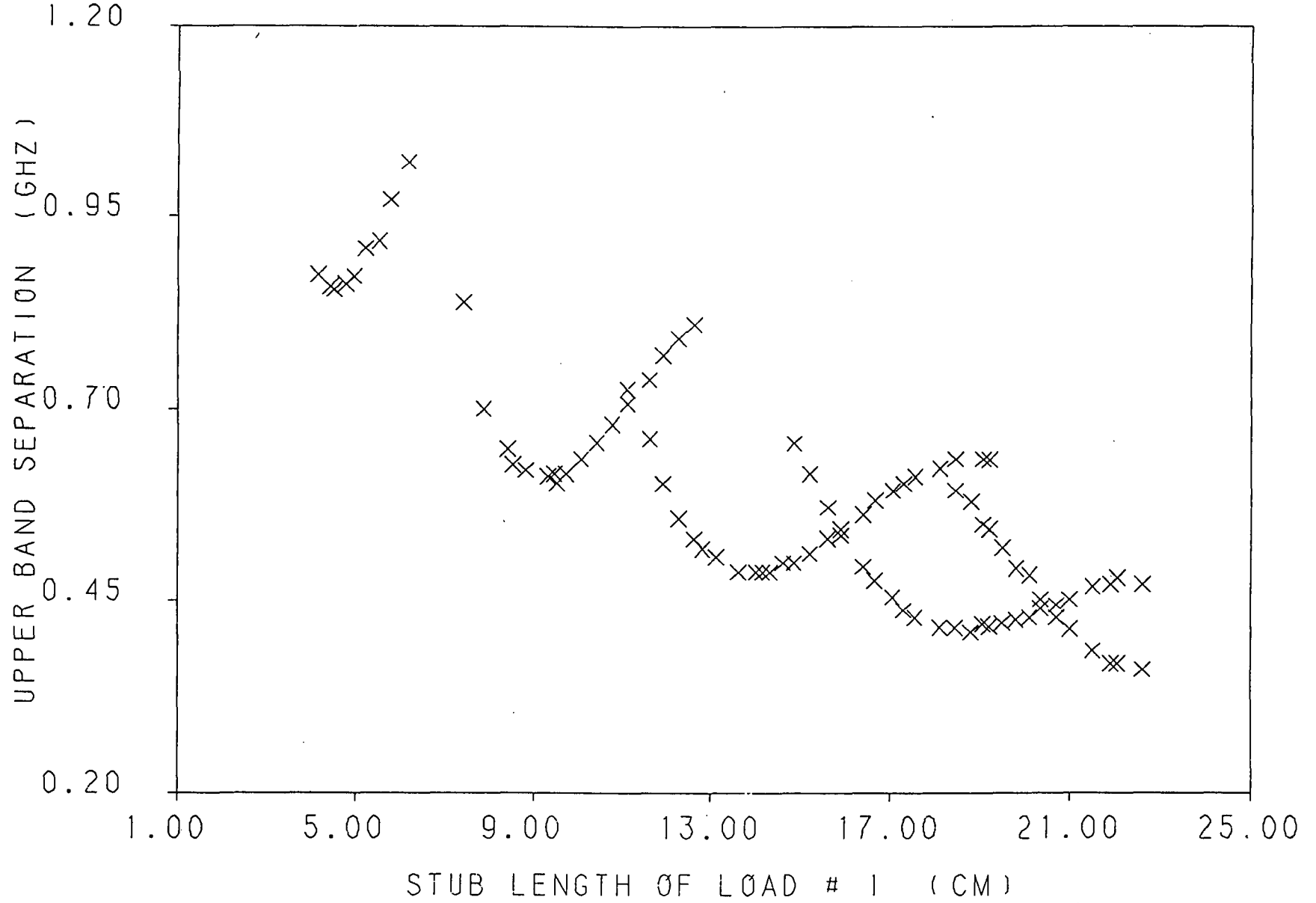
Fig. 3.94 Upper frequency band ( the x -polarized band ) separation verses the short circuit stub length of load #1 for a loaded 2.96 by 2.96 cm square patch with a feed location of (1.05, .45 cm ), and load insets of d = .35 cm .
