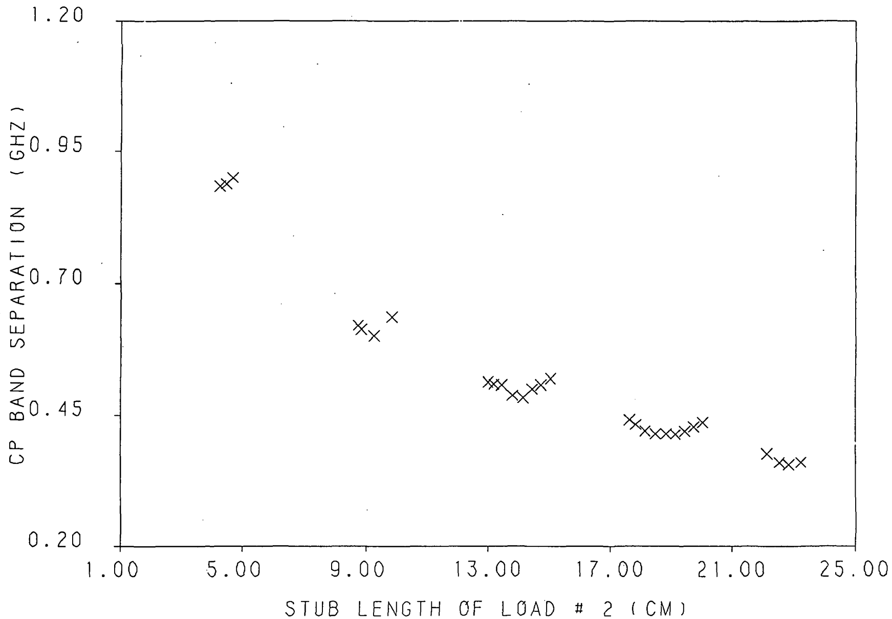
Fig. 3.99 Cp band separation versus the short circuit stub length of load # 2 for a loaded 2.96 by 2.96 cm square patch with a feed location of (1.05, .45 cm), and load insets of d = .35 cm.
