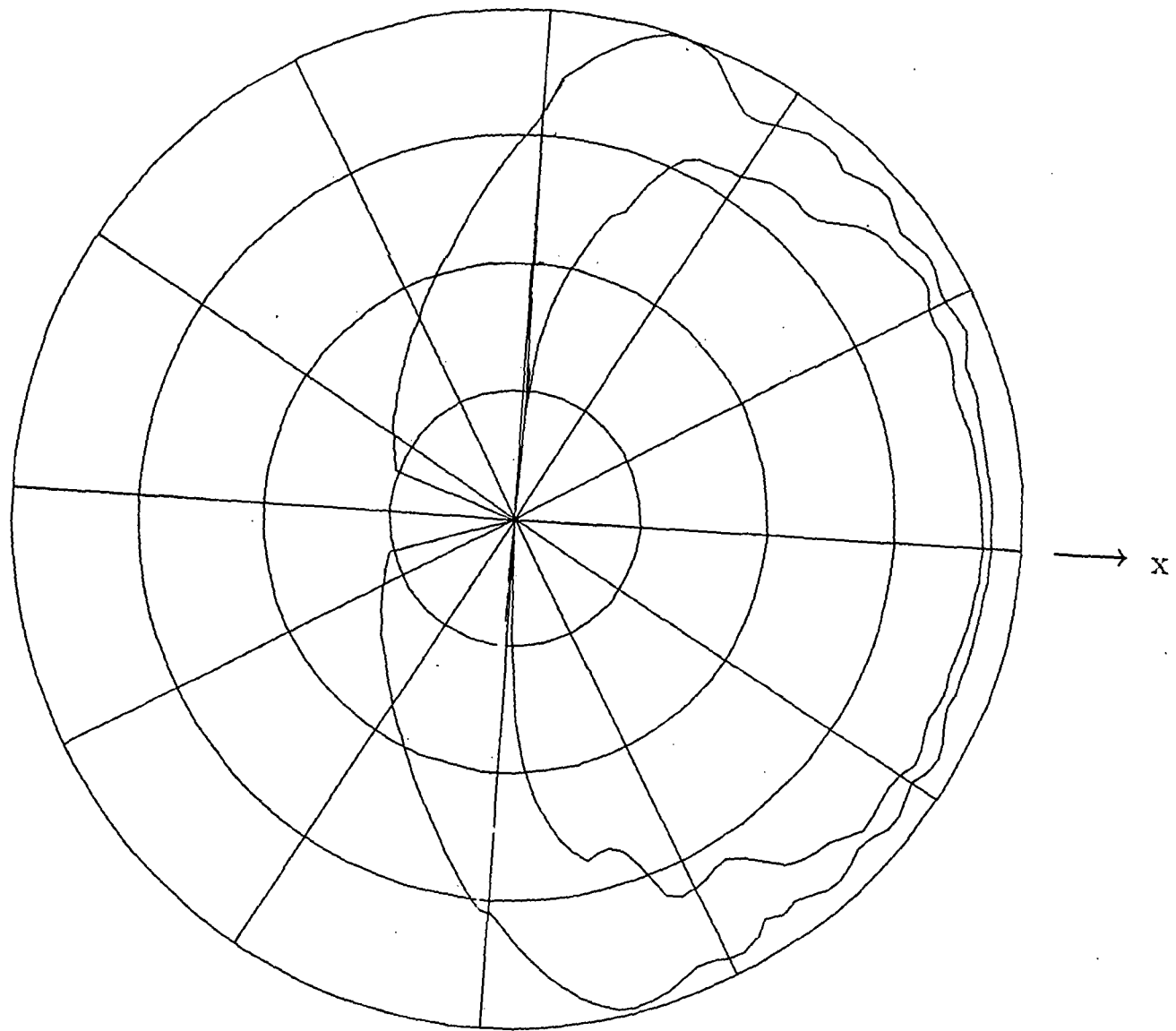
Fig 4.33 Far field radiation pattern of antenna at position 2 on backpack with astronaut ( \Theta = 90^\circ ).
