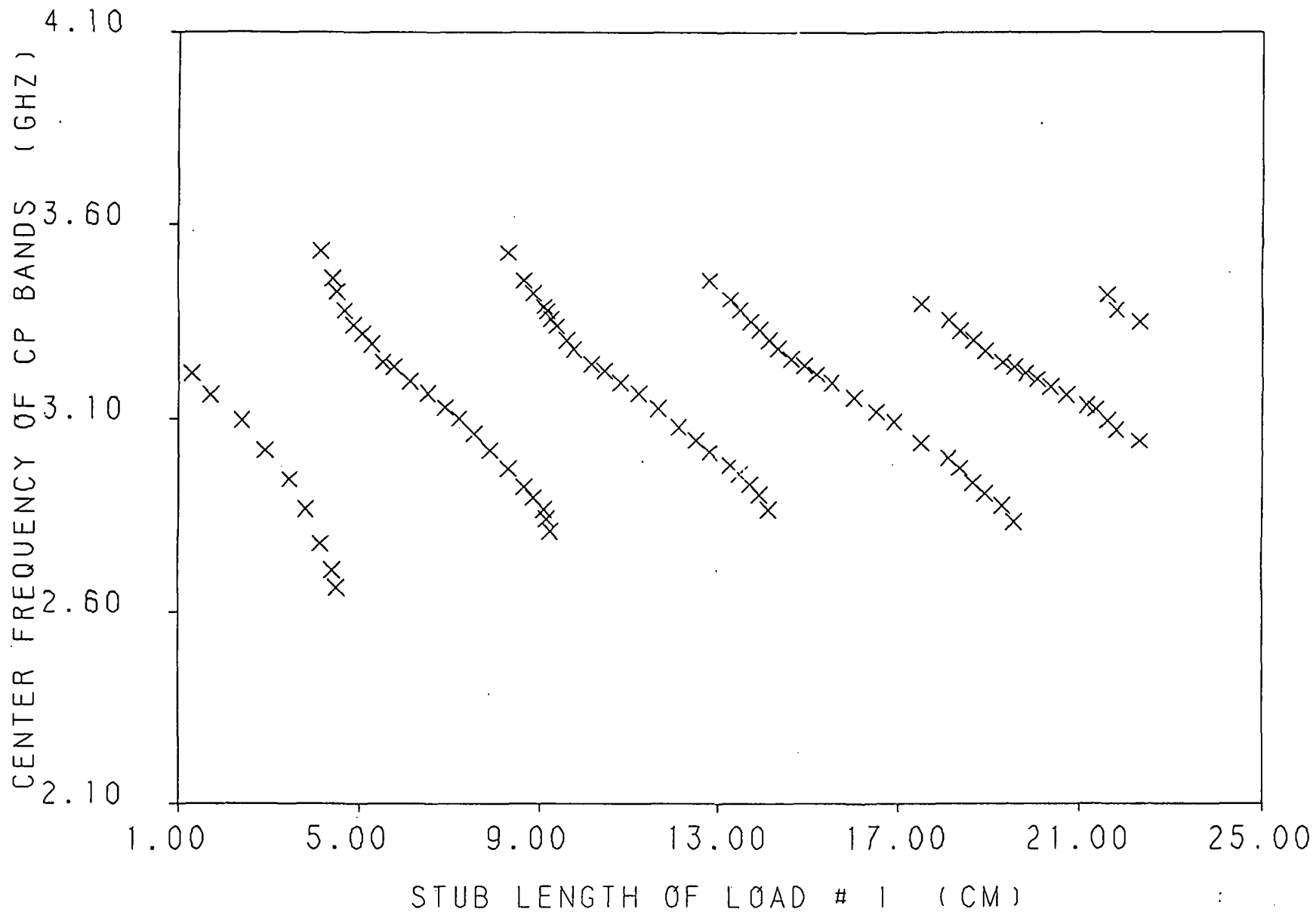
Fig. 3.119 Center frequency of cp bands versus the short circuit stub length of load # 1 for a loaded 2.96 by 2.96 cm square patch with a feed location of (.85, .45 cm), and load insets of d = .60 cm.
