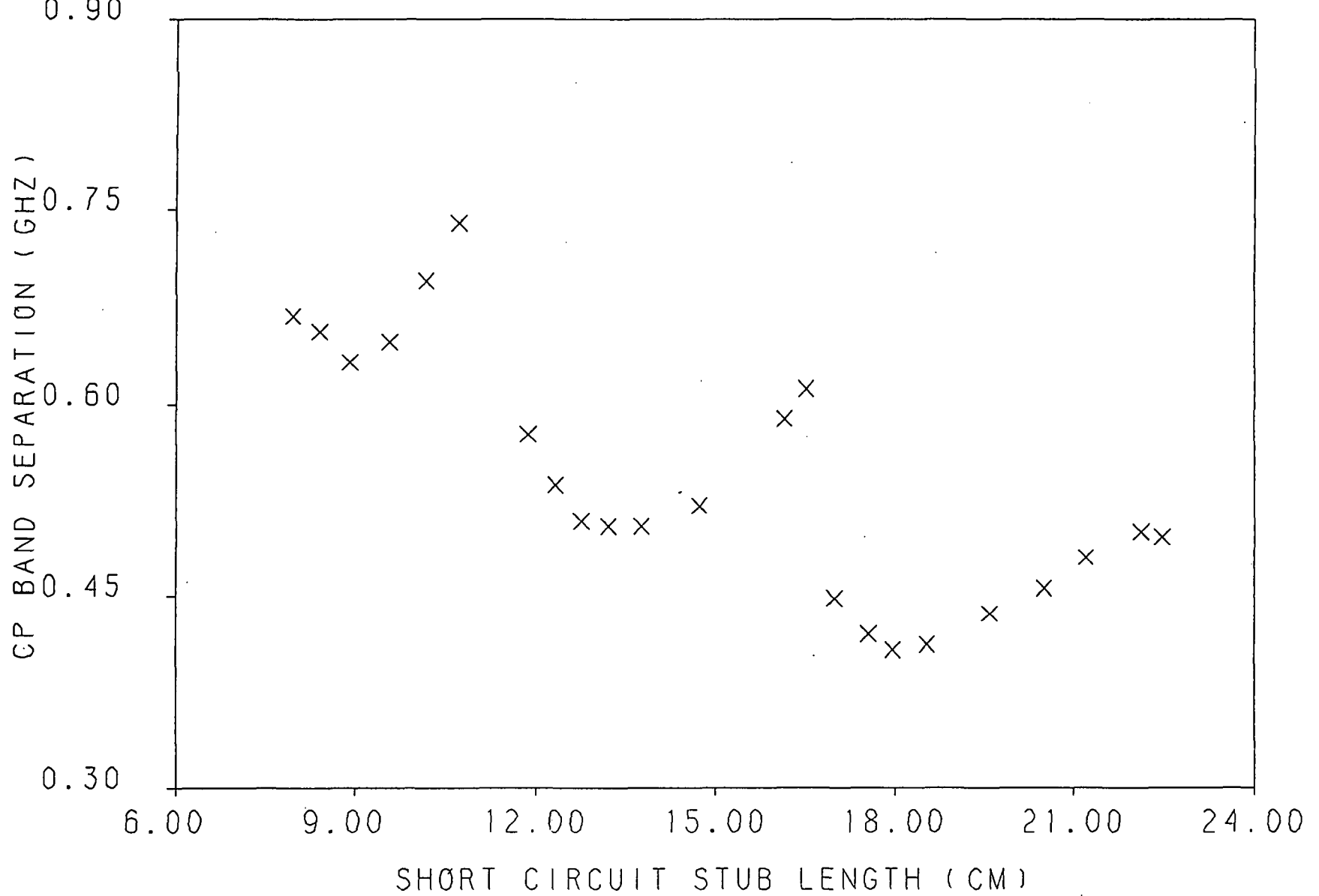
Fig. 3.25 Cp band separation versus the average short circuit stub length for a loaded 3.13 by 2.90 cm rectangular patch with a feed location of (.09, .09 cm), and load insets of d = .50 cm .
