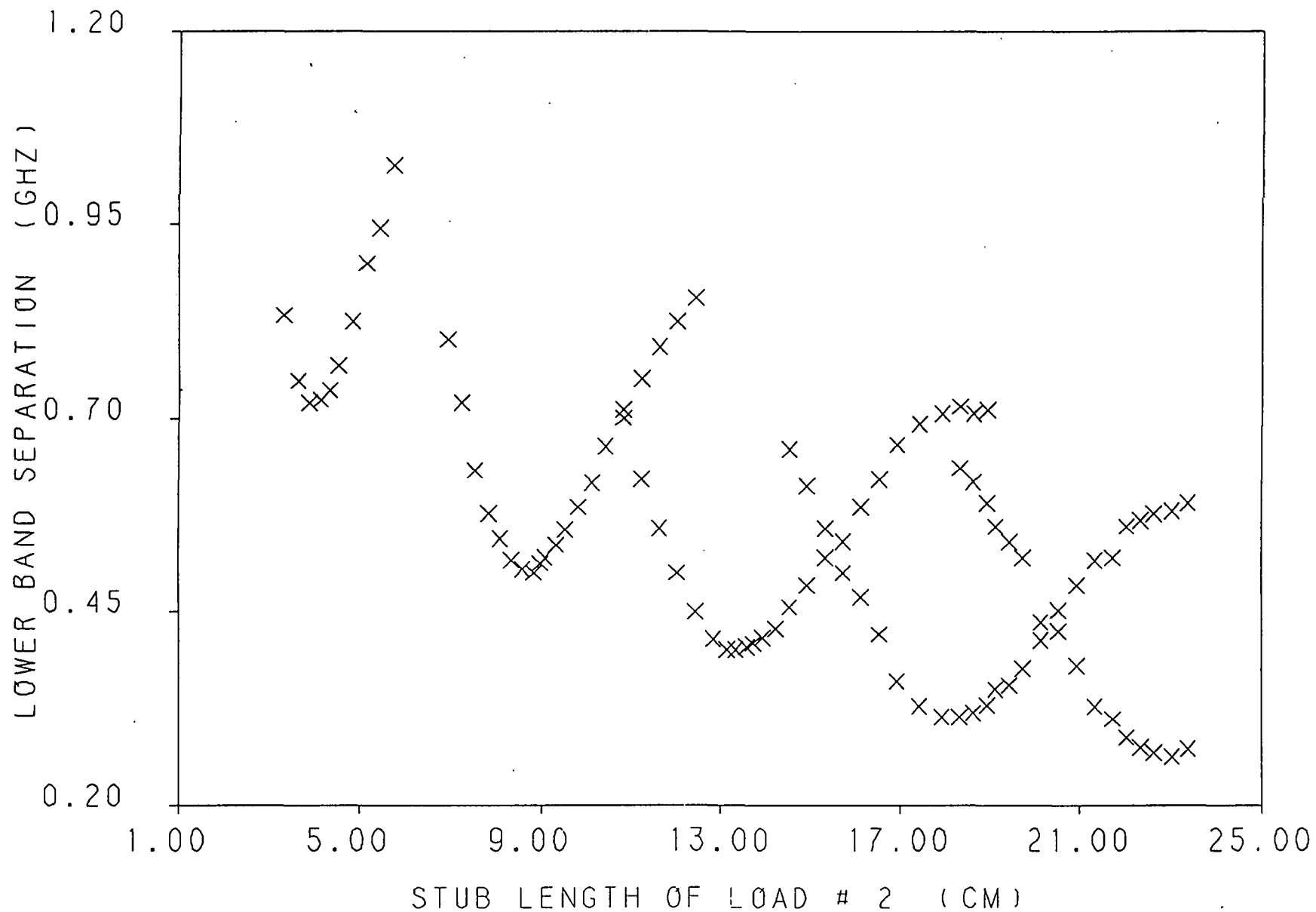
Fig. 3.118 Lower frequency band ( the y-polarized band ) separation versus the short circuit stub length of load #2 for a loaded 2.96 by 2.96 cm square patch with a feed location of (.85, .45 cm ), and load insets of d = .60 cm .
