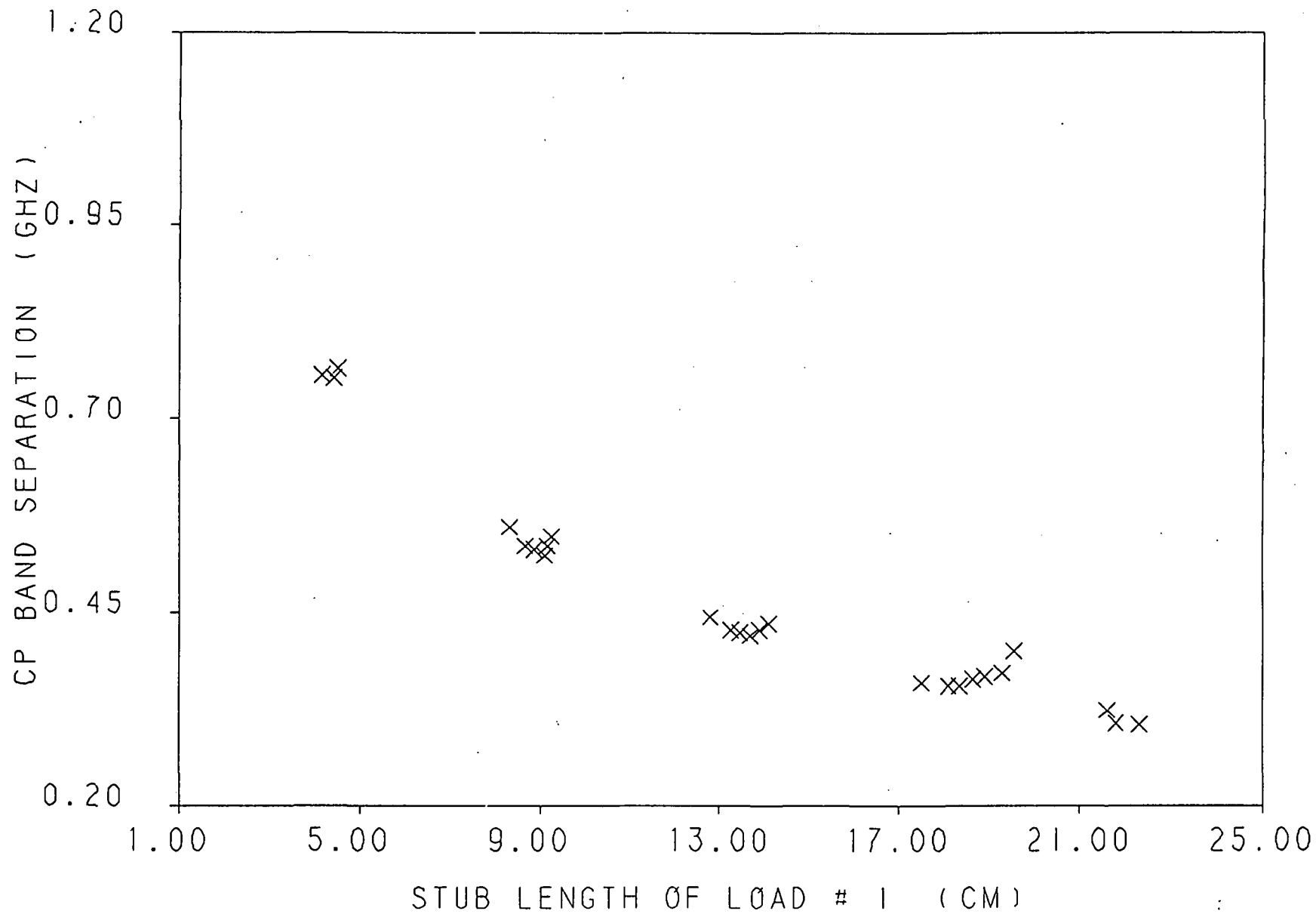
Fig. 3.121 Cp band separation versus the short circuit stub length of load # 1 for a loaded 2.96 by 2.96 cm square patch with a feed location of (.85, .45 cm), and load insets of d = .60 cm.
