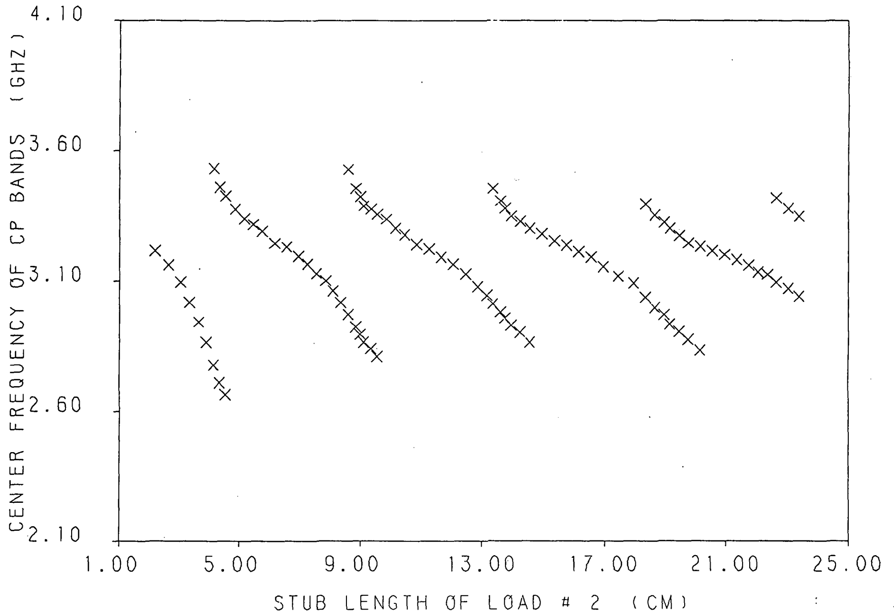
Fig. 3.120 Center frequency of cp bands versus the short circuit stub length of load # 2 for a loaded 2.96 by 2.96 cm square patch with a feed location of (.85, .45 cm), and load insets of d = .60 cm.
