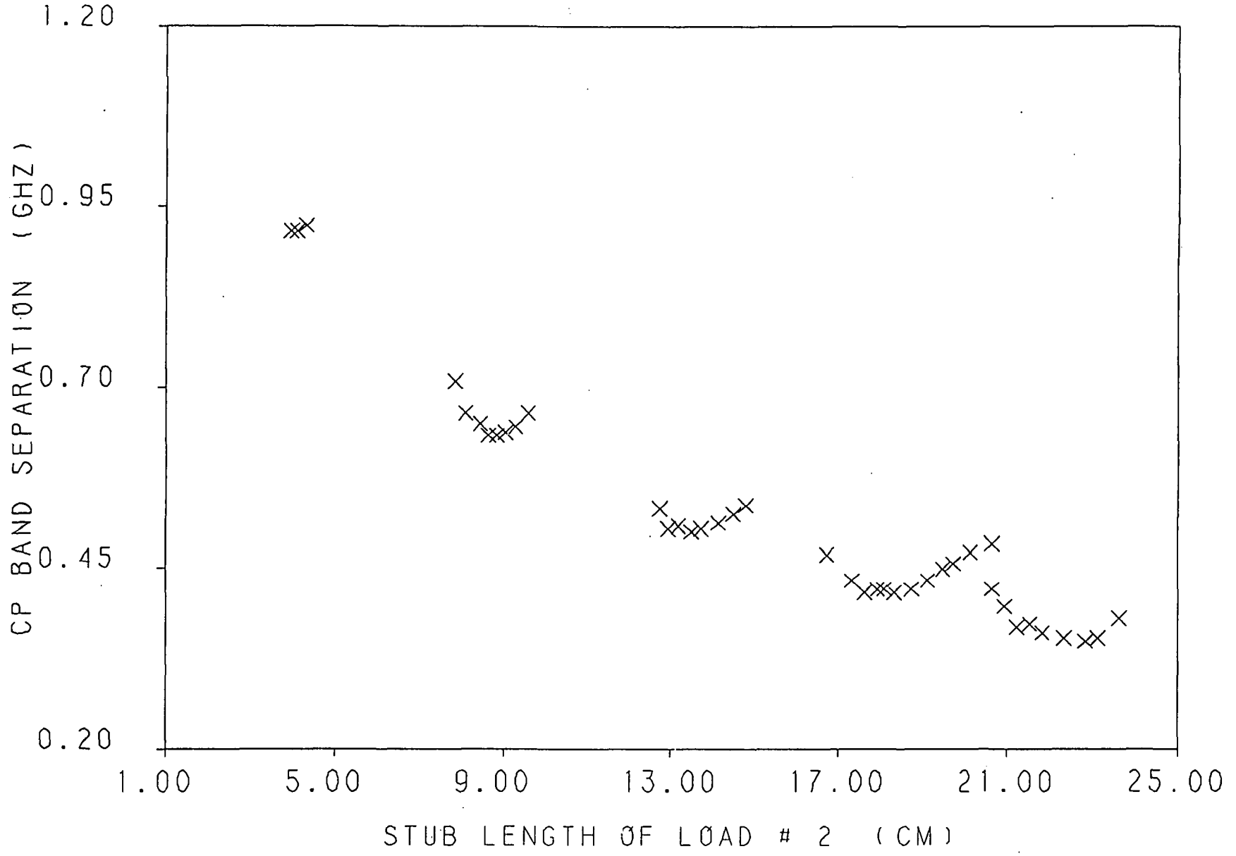
Fig. 3.48 Cp band separation versus the short circuit stub length of load # 2 for a loaded 2.96 by 2.96 cm square patch with a feed location of (.25, .25 cm ), and load insets of d = .11 cm .
