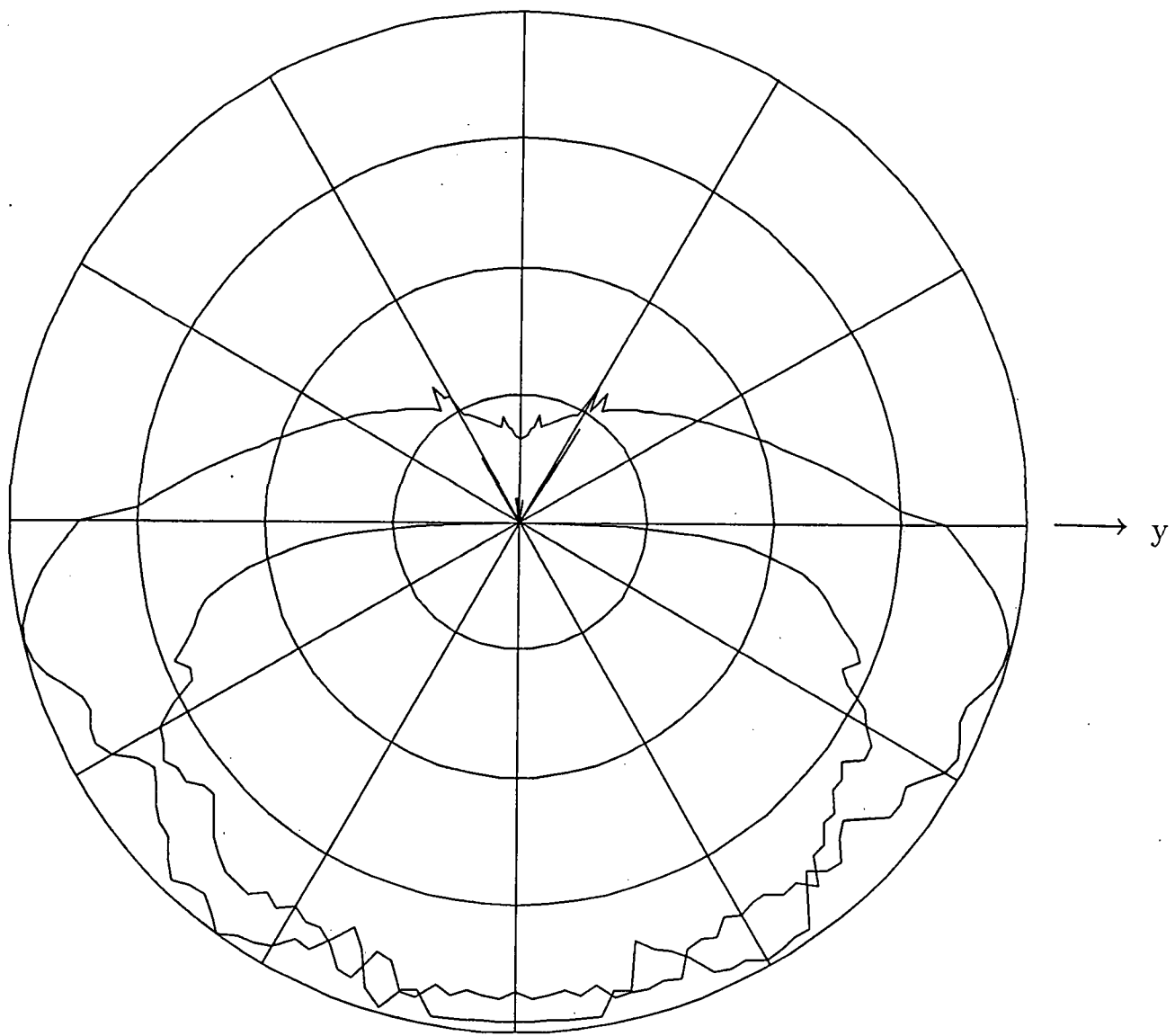
Fig 4.37 Far field radiation pattern of antenna at position 3 on backpack with astronaut ( \phi = 90^\circ ).
