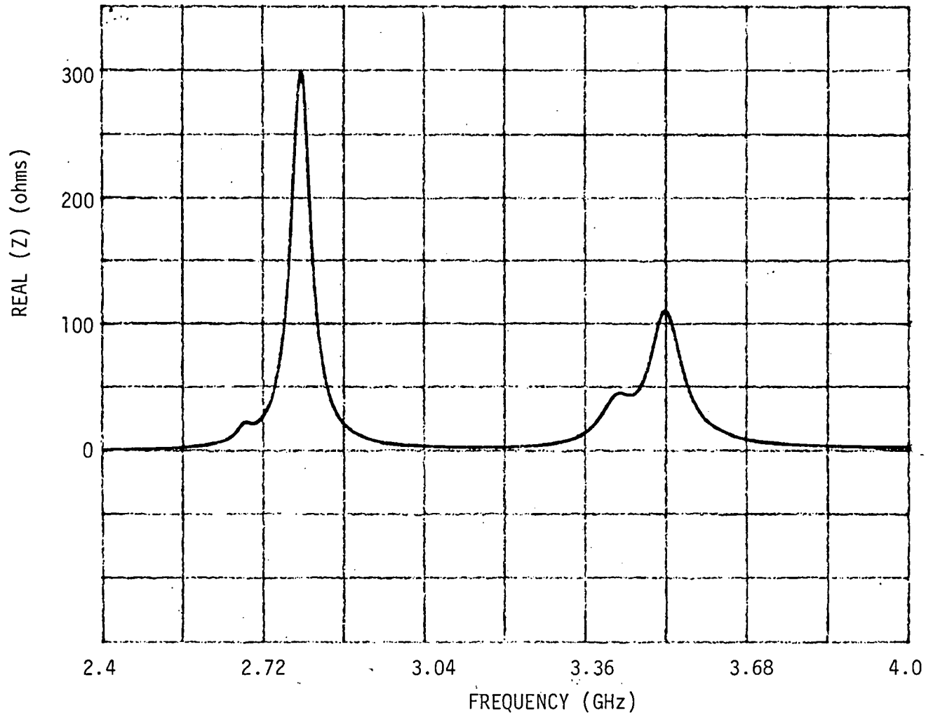
Fig. 3.100 Real part of input impedance versus frequency of the first mode for a loaded 2.96 by 2.96 cm square patch with a feed location of (.45, .85 cm), load insets of d = .60 cm, and stub lengths of s_1 = 4.4 cm and s_2 = 4.33 cm.
