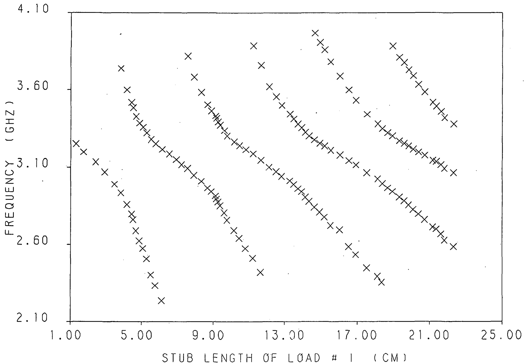
Fig. 3.115 Frequency of upper linearly polarized band ( the x -polarized band ) versus the short circuit stub length of load #1 for a loaded 2.96 by 2.96 cm square patch with a feed location of (.85, .45 cm ), and load insets of d = .60 cm .
