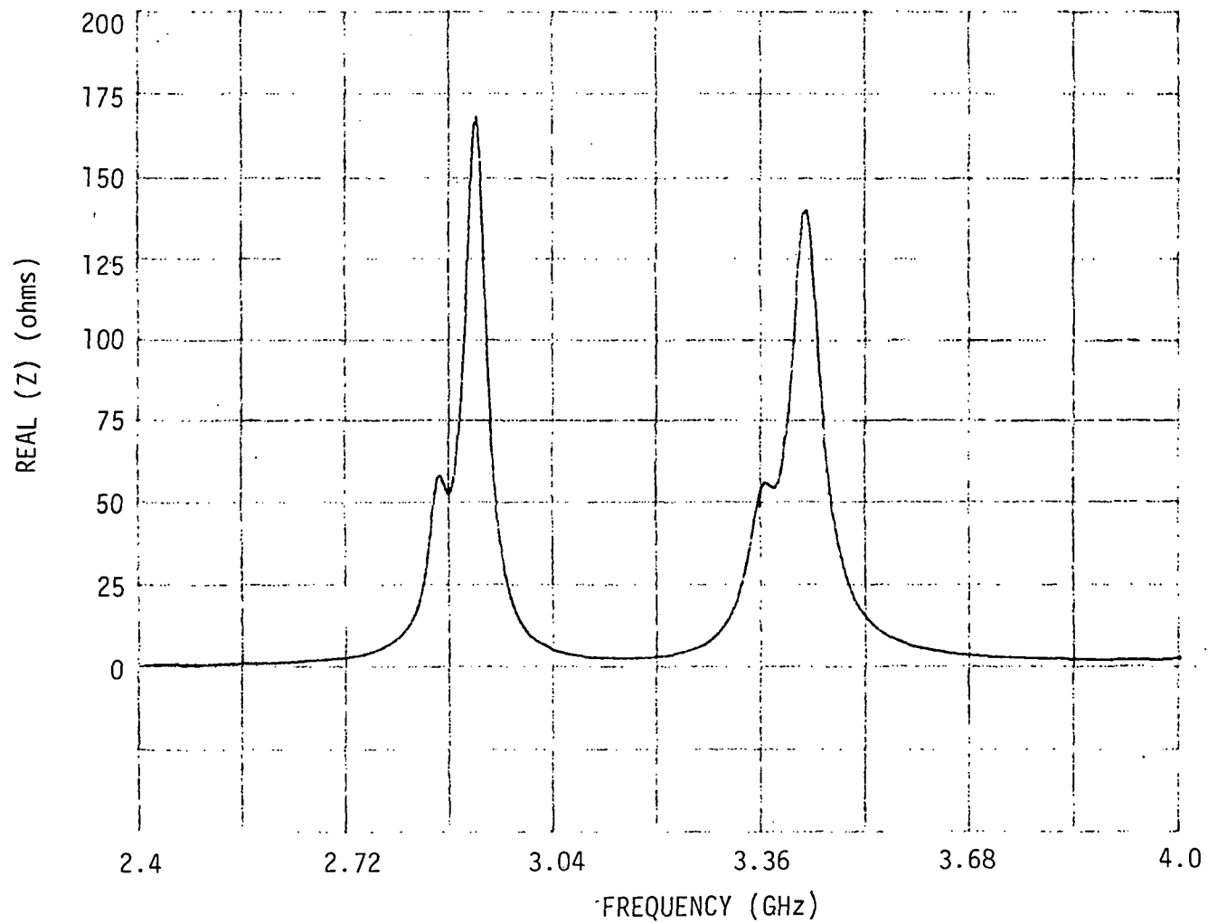
Fig. 3.60 Real part of input impedance versus frequency of the third mode for a loaded 2.96 by 2.96 cm square patch with a feed location of (.45, 1.05 cm), load insets of d = .11 cm, and stub lengths of s_1 = 13.7 cm and s_2 = 13.78 cm.
