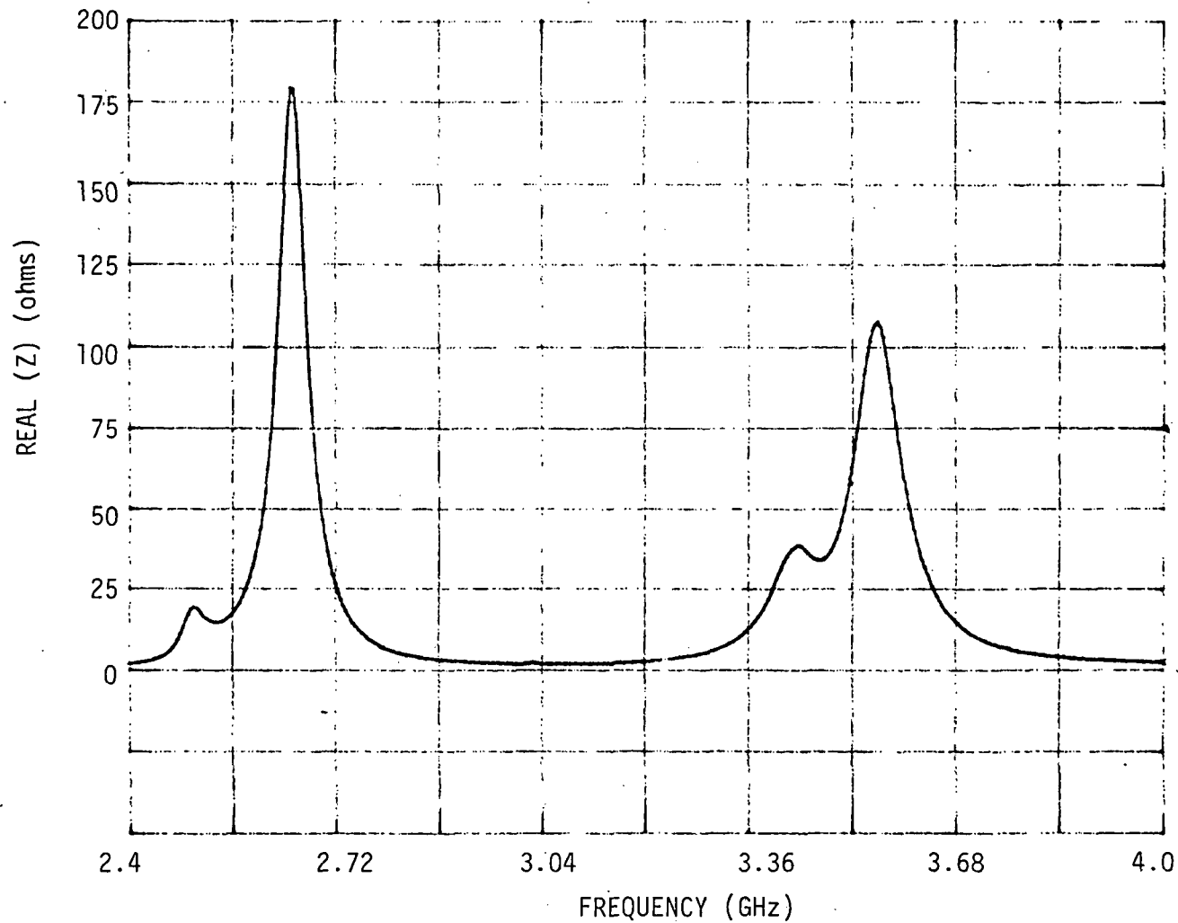
Fig. 3.54 Real part of input impedance versus frequency of the first mode for a loaded 2.96 by 2.96 cm square patch with a feed location of (.45, 1.05 cm), load insets of d = .11 cm, and stub lengths of s_1 = 4.5 cm and s_2 = 4.48 cm.
