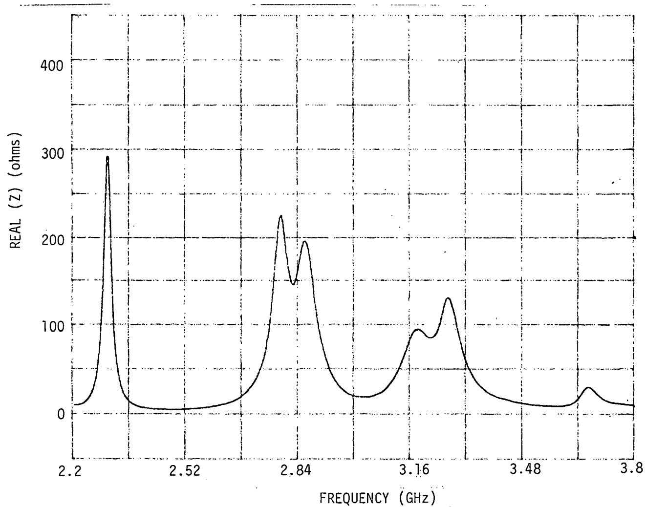
Fig. 3.18 Real part of impedance versus frequency of the fourth mode for a loaded 3.13 by 2.90 cm rectangular patch with a feed location of (.52, .48 cm), load insets of d = .70 cm, and stub lengths of s_1 = 18.1 cm and s_2 = 19.43 cm.
