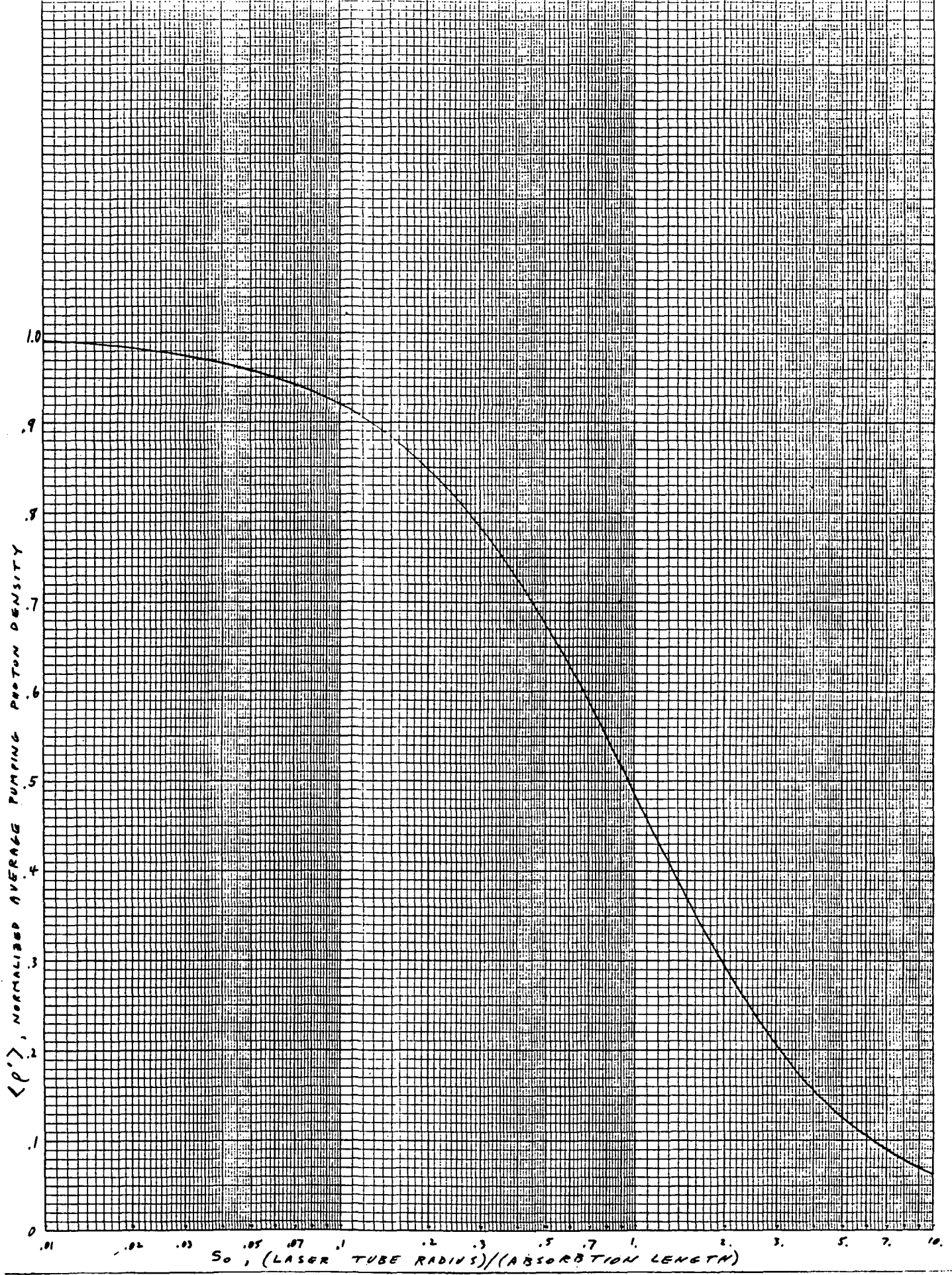
Figure A.7 \langle \rho' \rangle vs S_0 011 semi-log scale.
