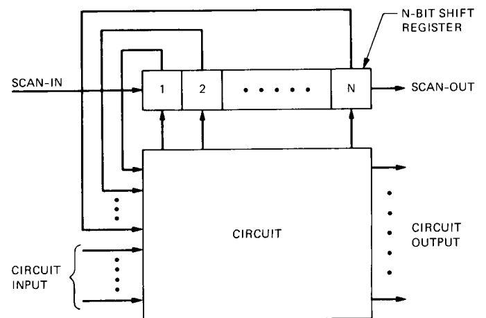
Fig. 8. Block diagram of the scan/set technique.
