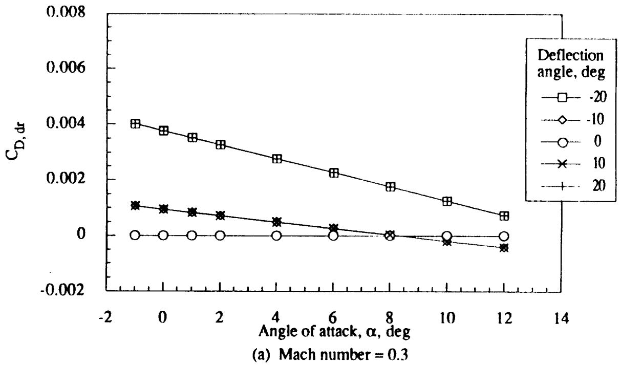
Figure 5.- Drag increment coefficient for rudder as a function of angle of attack, deflection angle, and Mach number.
