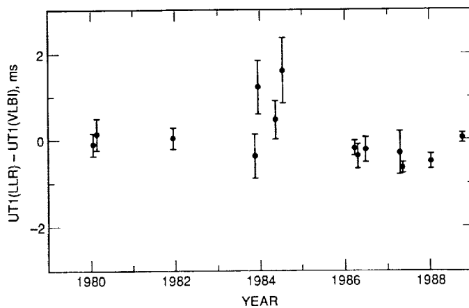
Fig. 3. Offset between the VLBI and LLR UT1 series.
