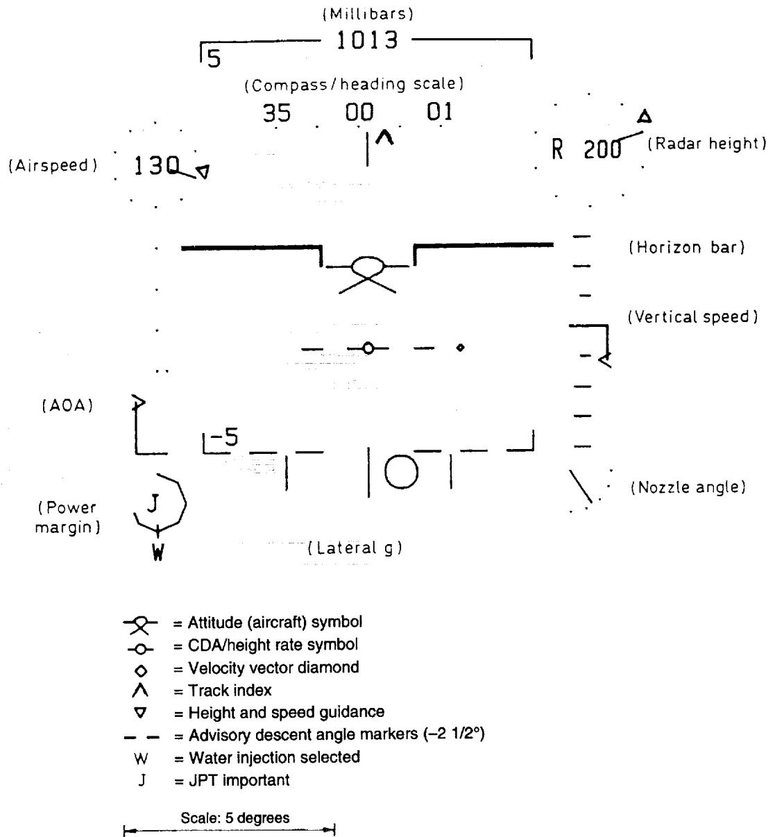
Figure 6. RAE HUD V/STOL format.
