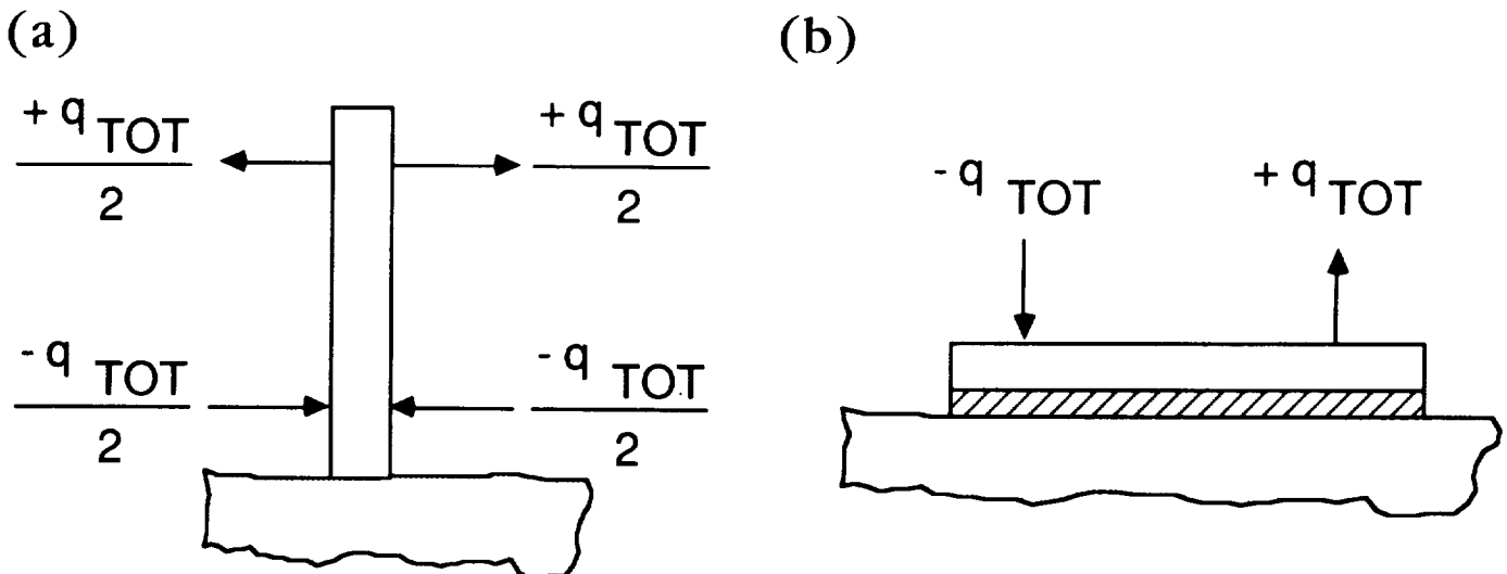
Fig. 6. Heat flux conventions used.
