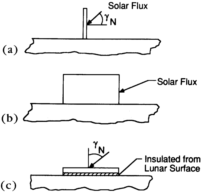
Fig. 5. Radiator orientations.
