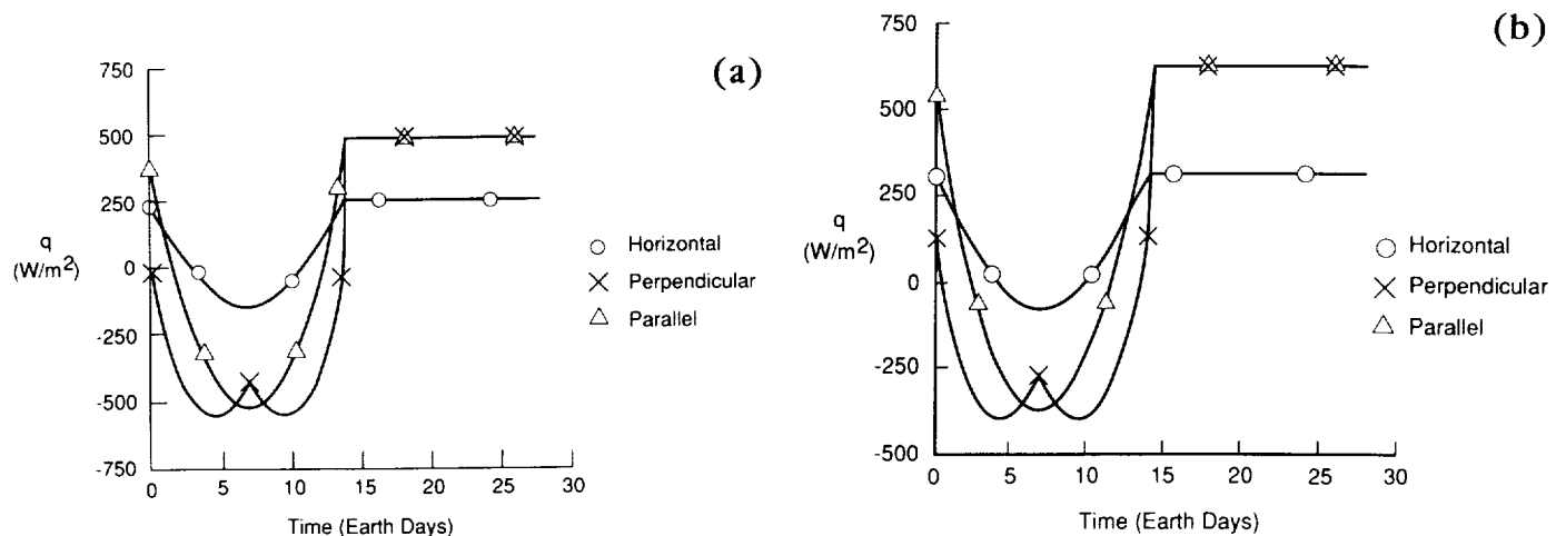
Fig. 8. (a) Heat rejection capability for radiators with a wall temperature of -6°C at Lacus Veris. (b) Heat rejection capability for radiators with a wall temperature of 13°C at Lacus Veris.
