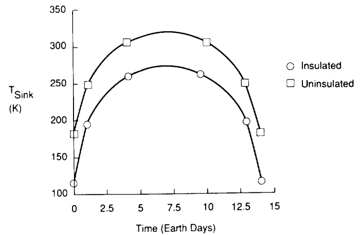
Fig. 11. Uninsulated vs. insulated sink temperatures over the lunar day for a radiator at Lacus Veris.
