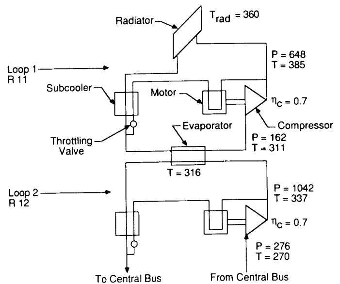
Fig. 12. Two-loop cascaded vapor cycle system.
