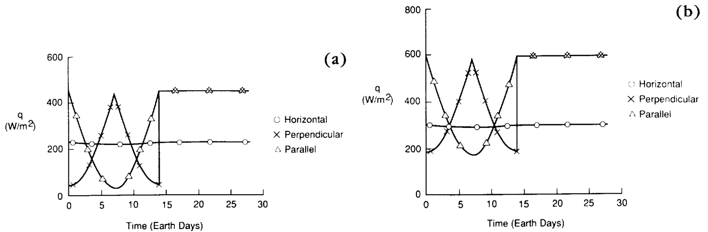
Fig. 7. (a) Heat rejection capability for radiators with a wall temperature of -6°C at the South Pole. (b) Heat rejection capability for radiators with a wall temperature of 13°C at the South Pole.
