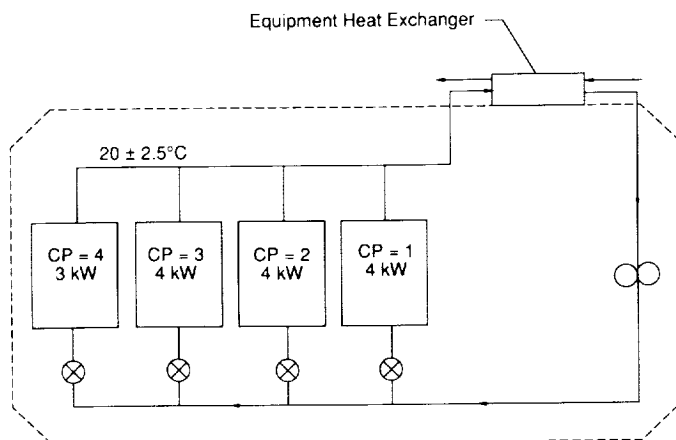
Fig. 3. Typical cold plate configuration for an integrated module.
