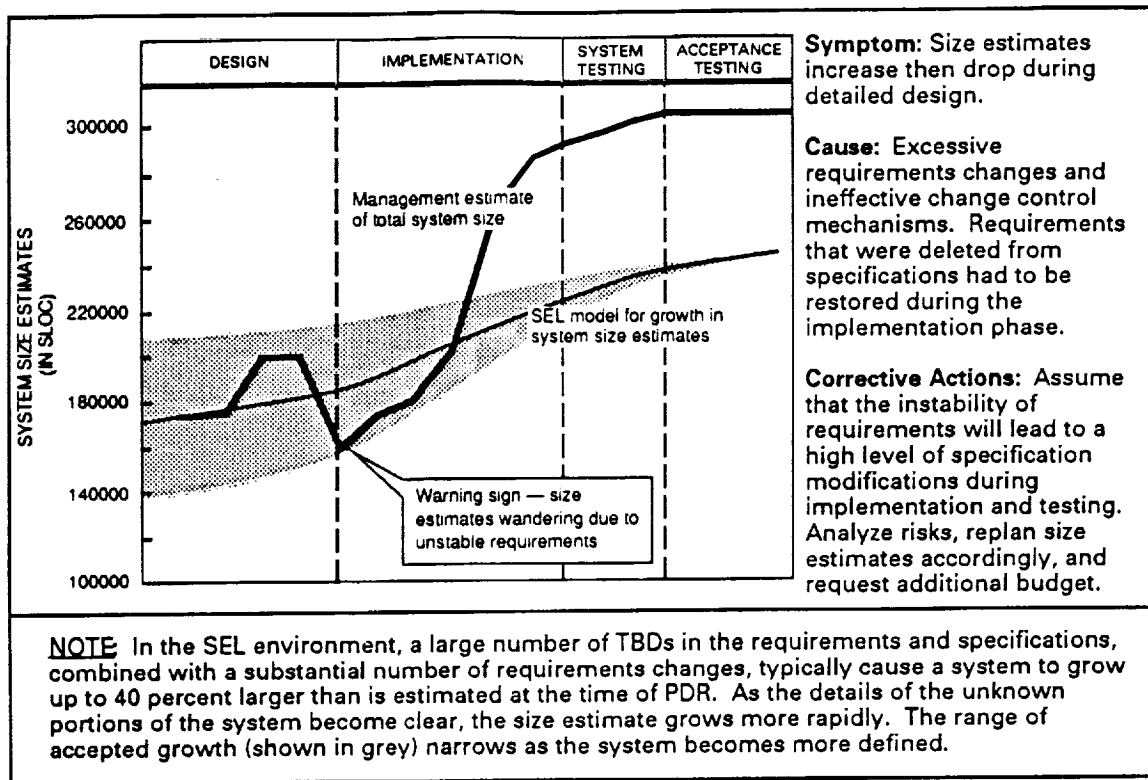
Figure 6-4. Example of the Impact of Requirements Changes on Size Estimates — the UARS Attitude Ground Support System
