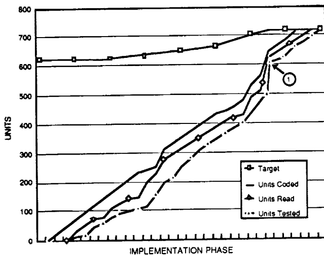
Figure 7-6. Development Profile Example
