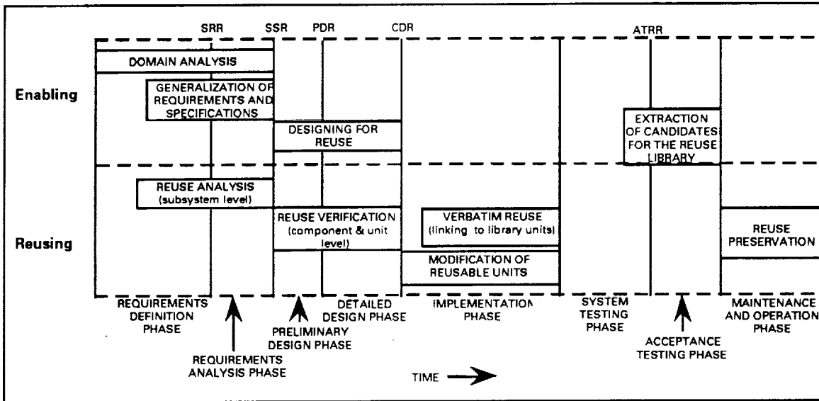
Figure 2-2. Reuse Activities Within the Life Cycle
