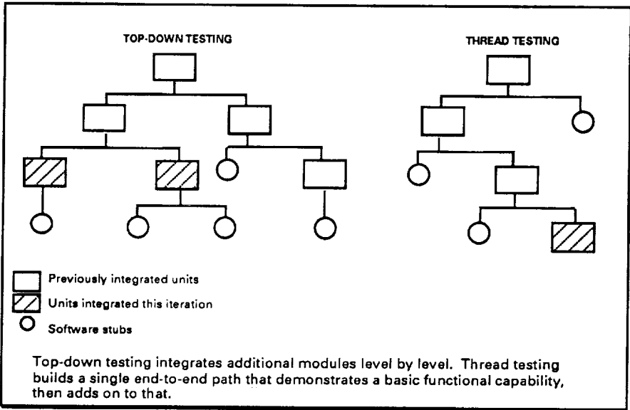
Figure 7-5. Integration Testing Techniques
