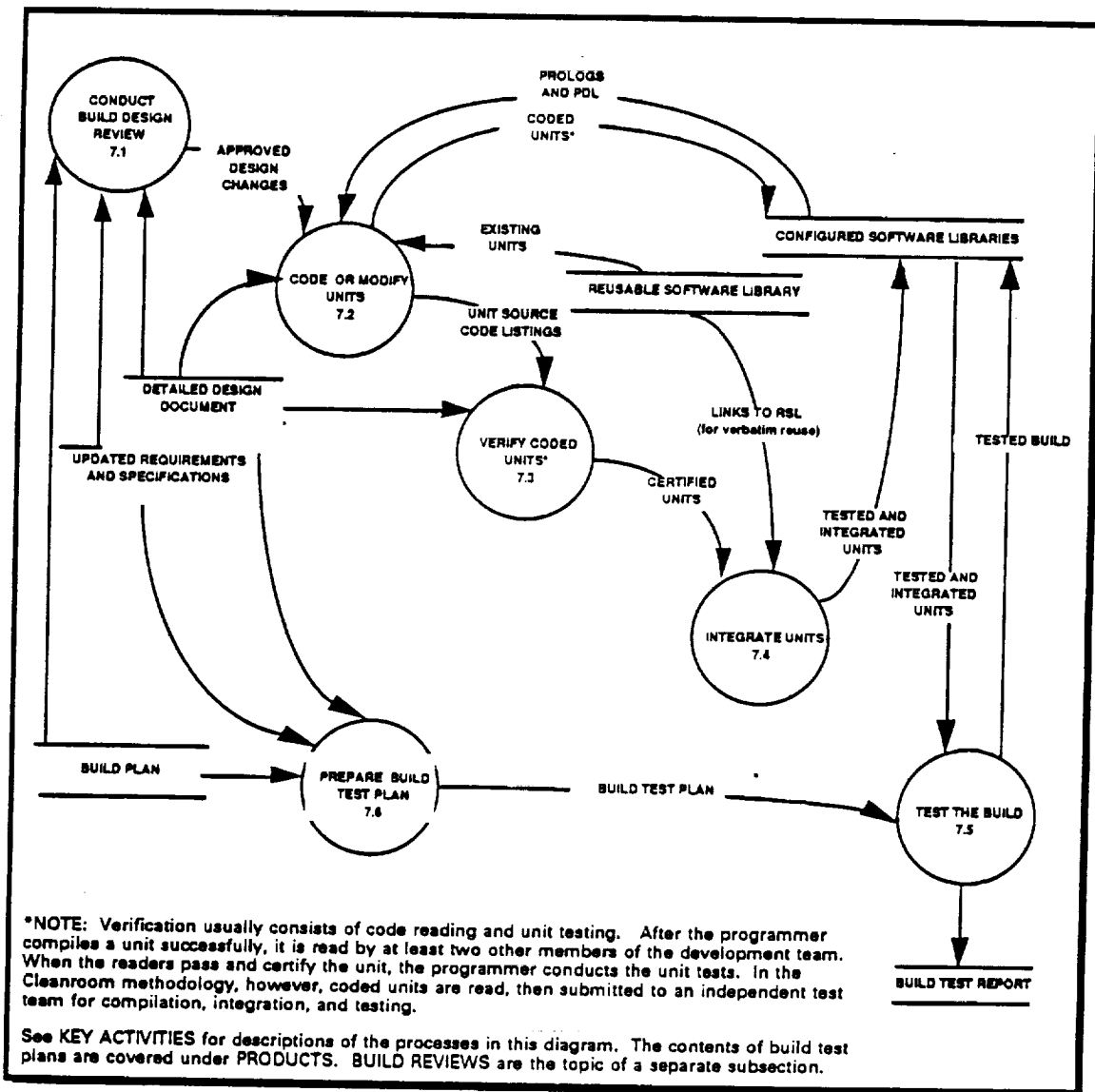
Figure 7-1. Implementing a Software Build
