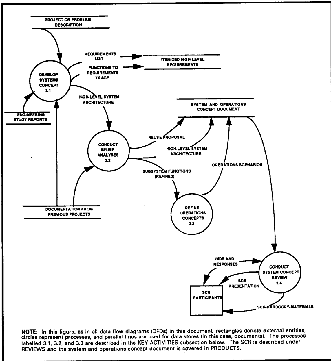
Figure 3-1. Generating the System and Operations Concept
