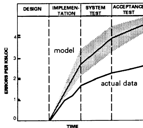
Figure 9-3. Sample Error-Rate Profile, UARS AGSS
