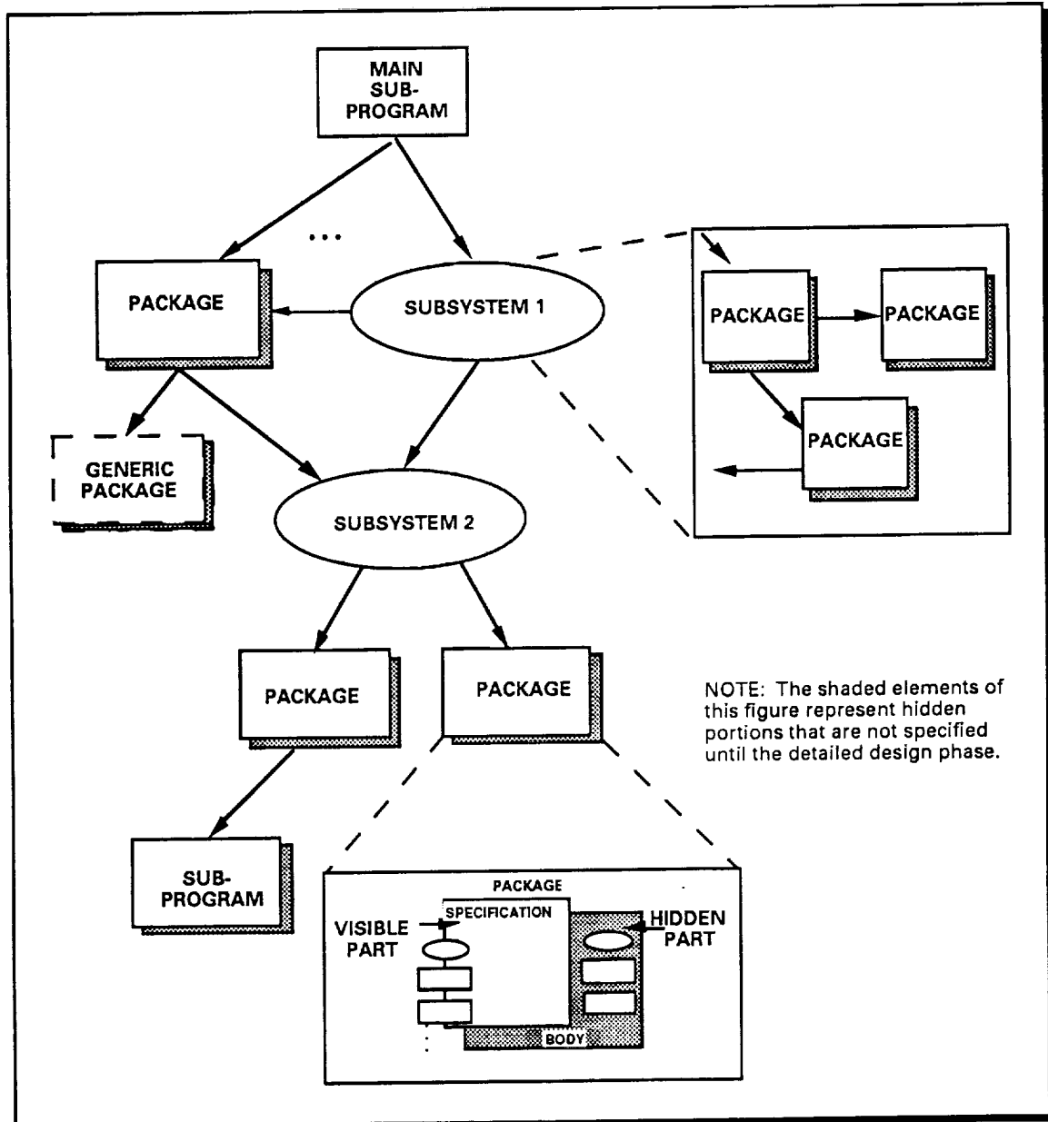
Figure 5-4. Level of Detail Produced for Ada Systems During Preliminary Design
