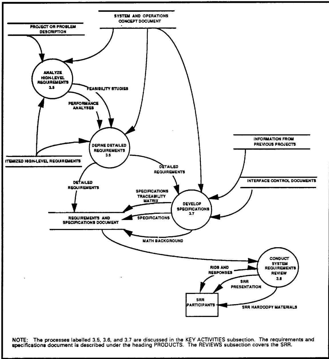
Figure 3-2. Developing Requirements and Specifications
