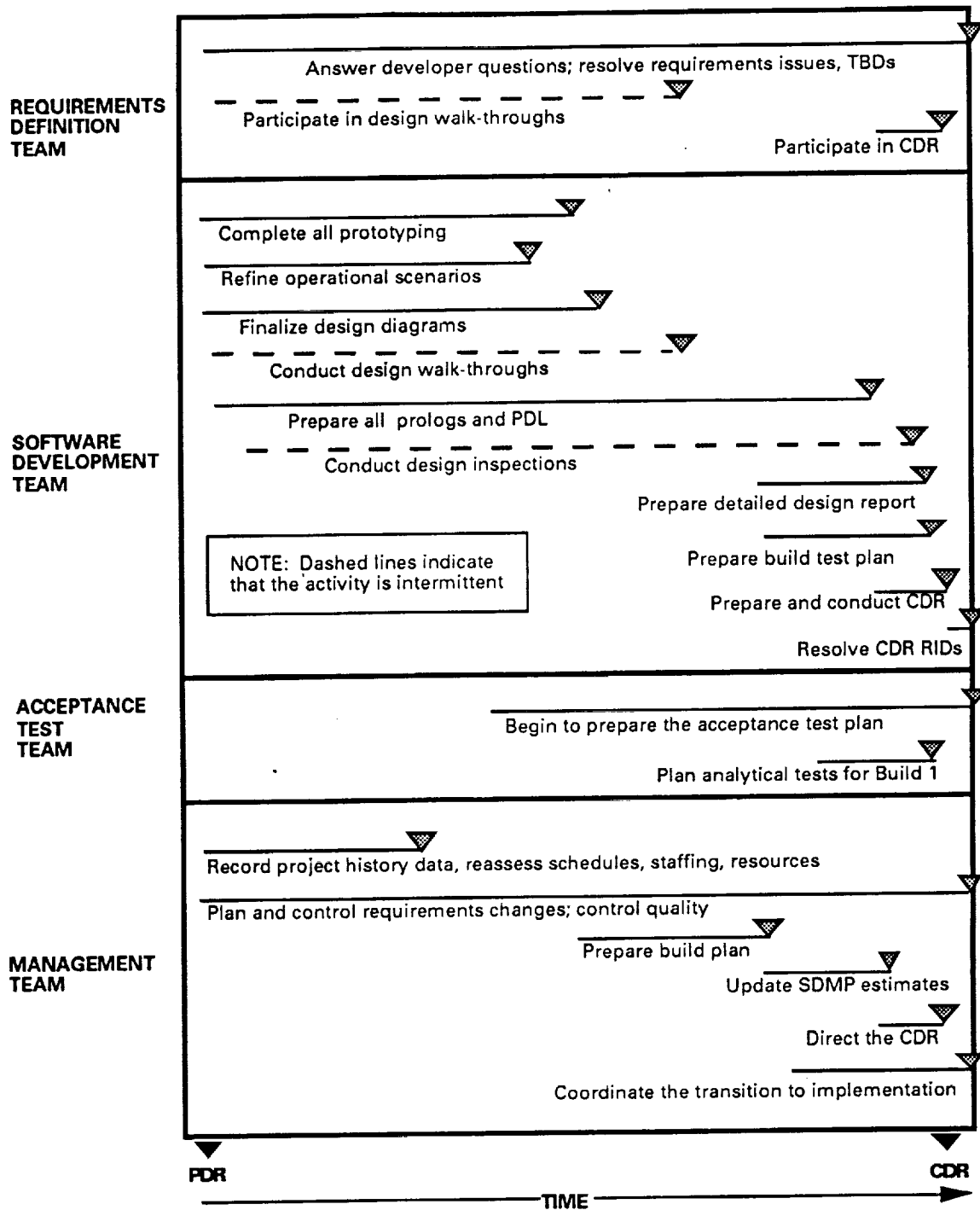
Figure 6-2. Timeline of Key Activities in the Detailed Design Phase
