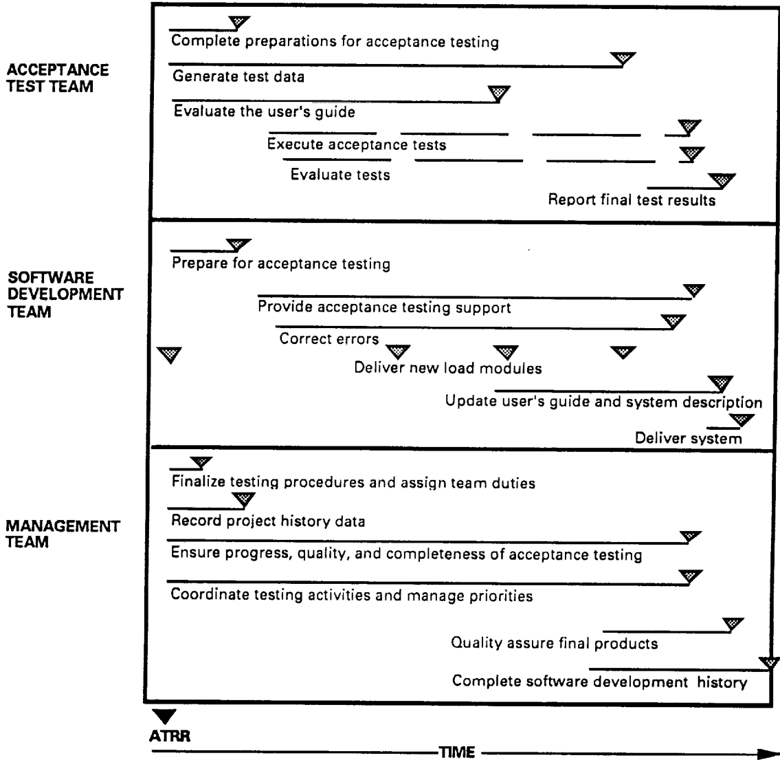
Figure 9-2. Timeline of Key Activities in the Acceptance Testing Phase
