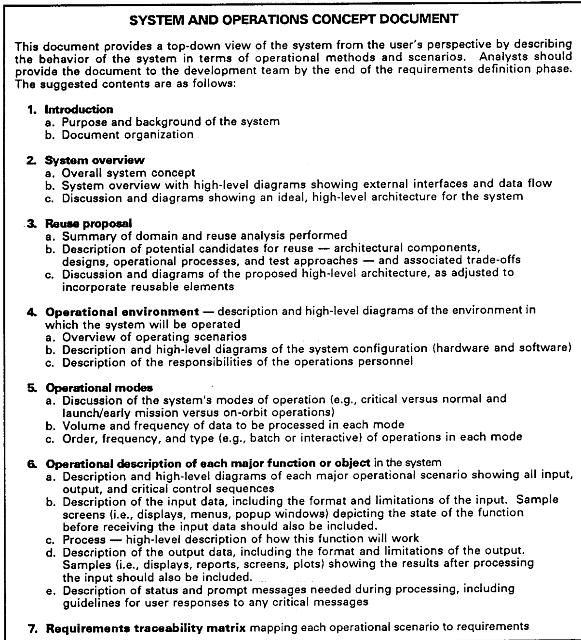
Figure 3-3. SOC Document Contents
