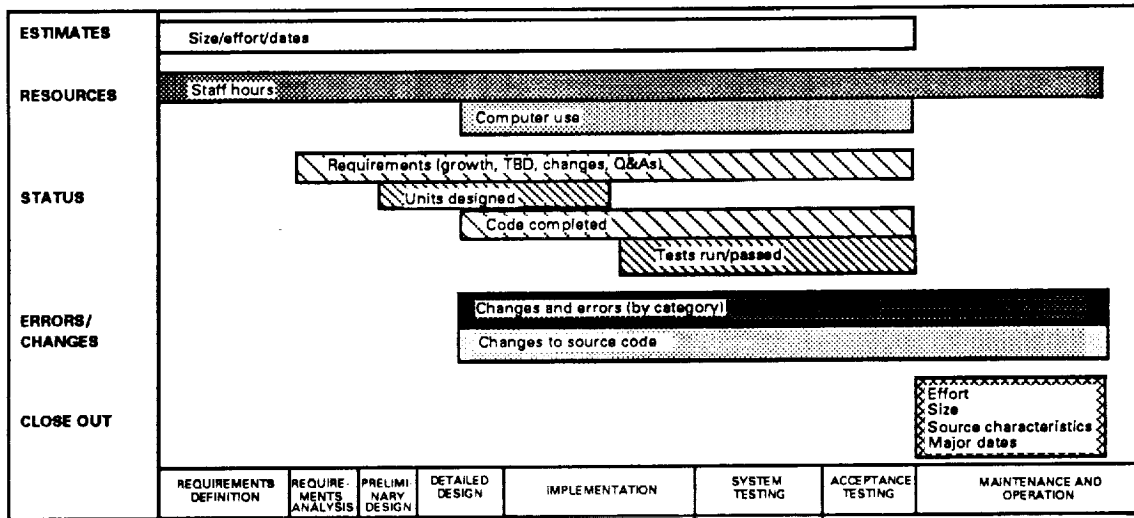
Figure 2-3. Graph Showing in Which Life-Cycle Phases Each Measure Is Collected
