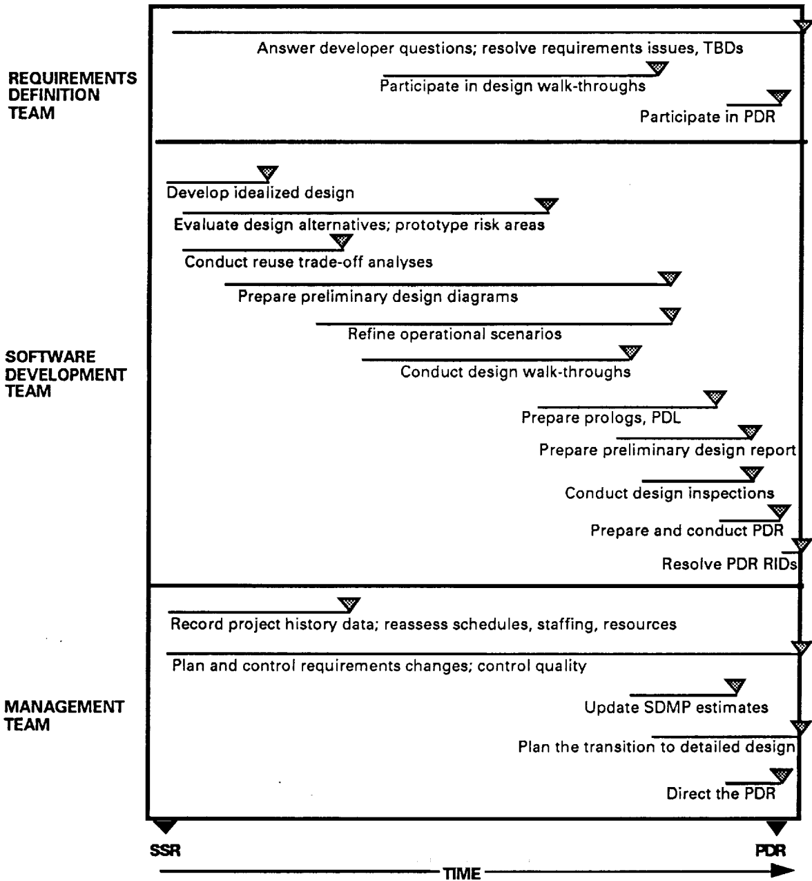
Figure 5-2. Preliminary Design Phase Timeline
